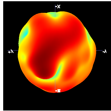
2.4G 3D
