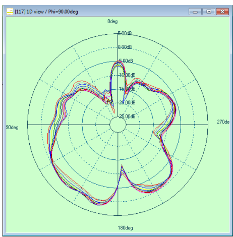
2.4G phi=90deg
