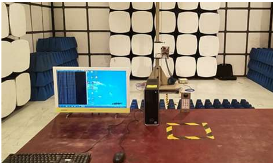
Radiated Emission Test Set-up(1-5GHz)
