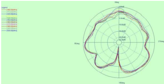
2.4G phi=90deg
