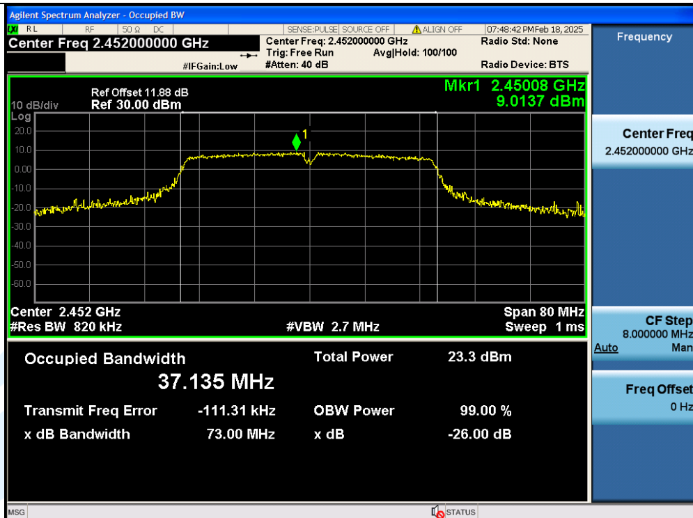
11N40SISO-Ant1-2452
