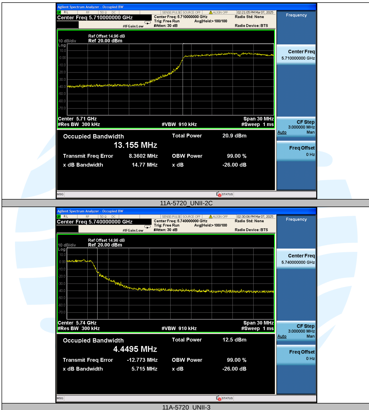
11A-5720_UNII-3
