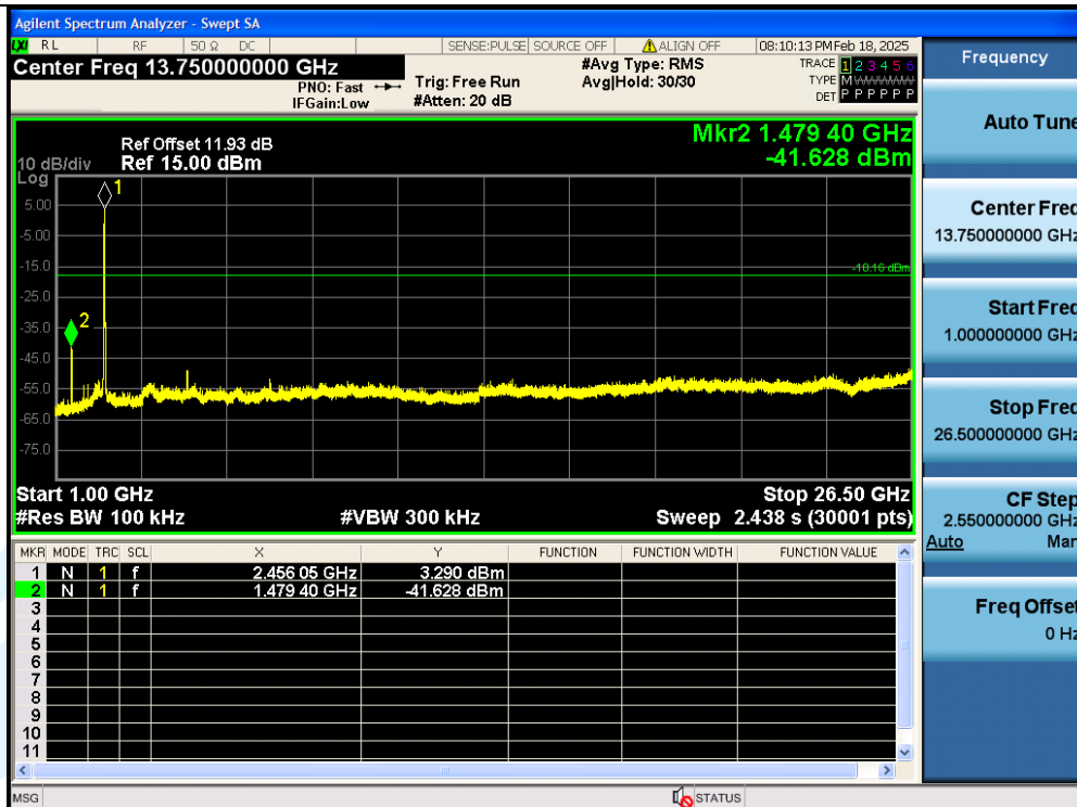
11AX20SISO-Ant1-2462-1000~26500-PASS
