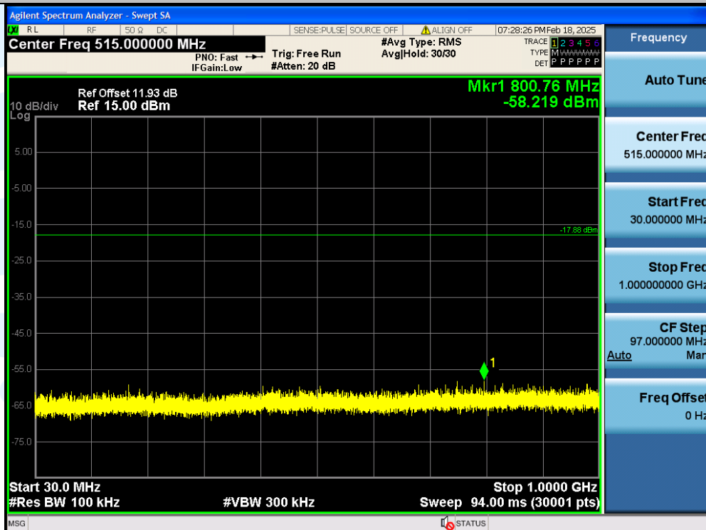
11N20SISO-Ant1-2462-30~1000-PASS
