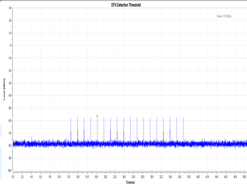
11AX20SISO-5500-Type0-PASS
