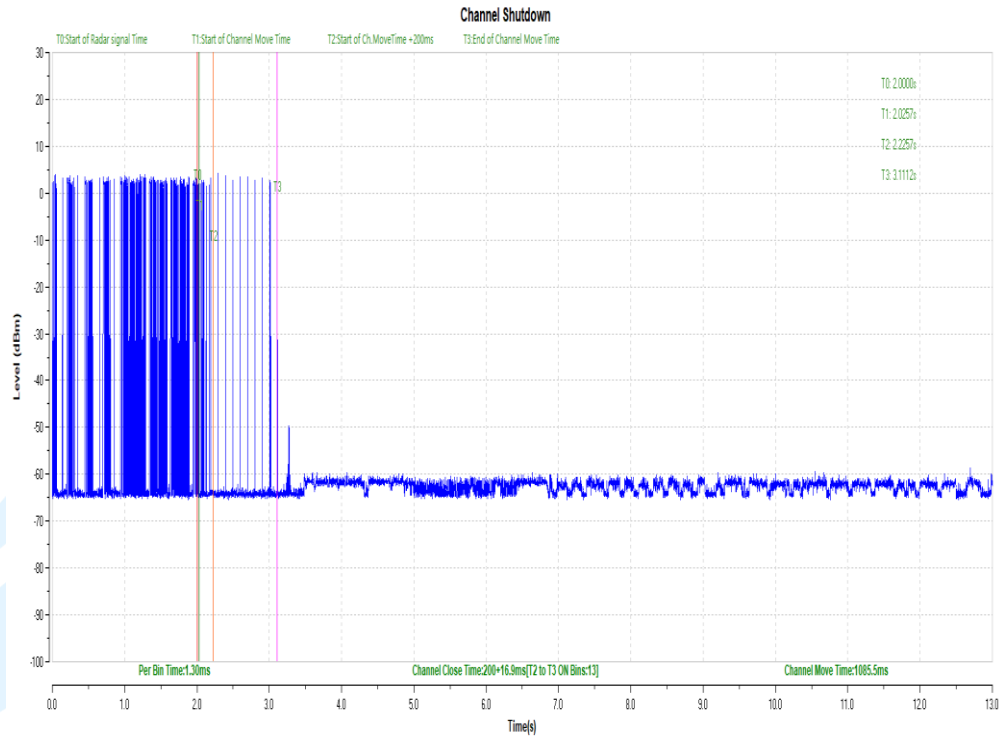
11AX20SISO-5500-Type0-PASS
