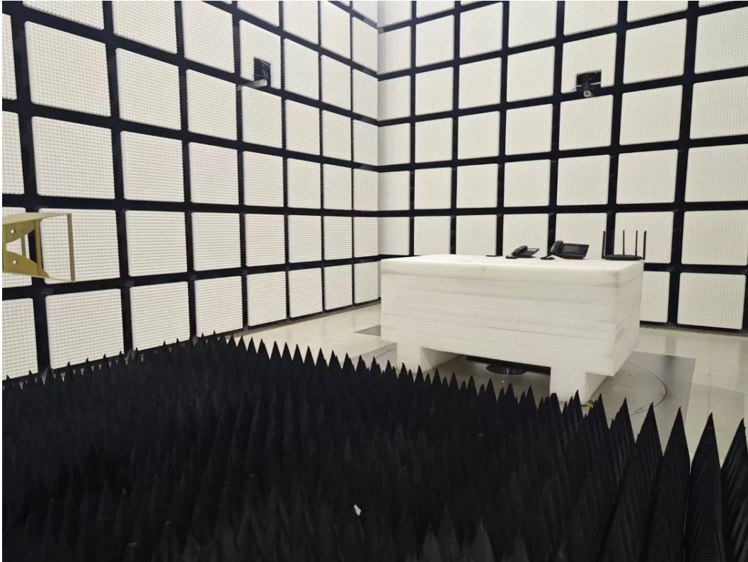
Radiated Emissions Above 1GHz Rear View-M5&M6
