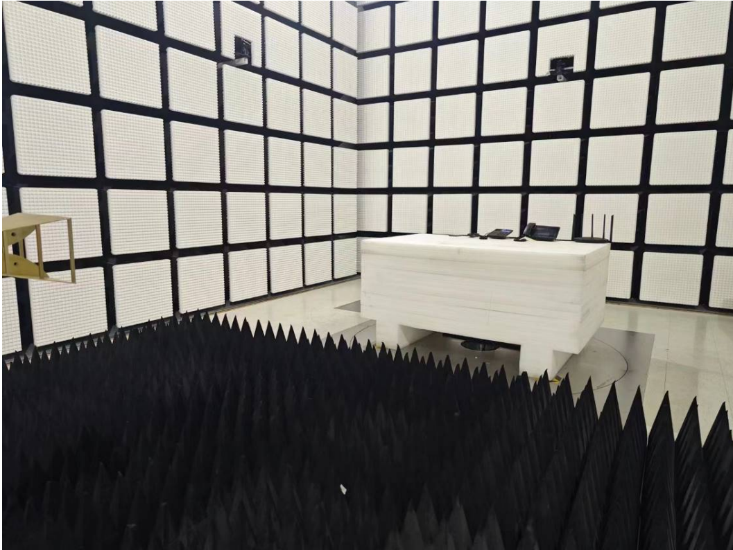
Radiated Emissions Above 1GHz Rear View-M4
