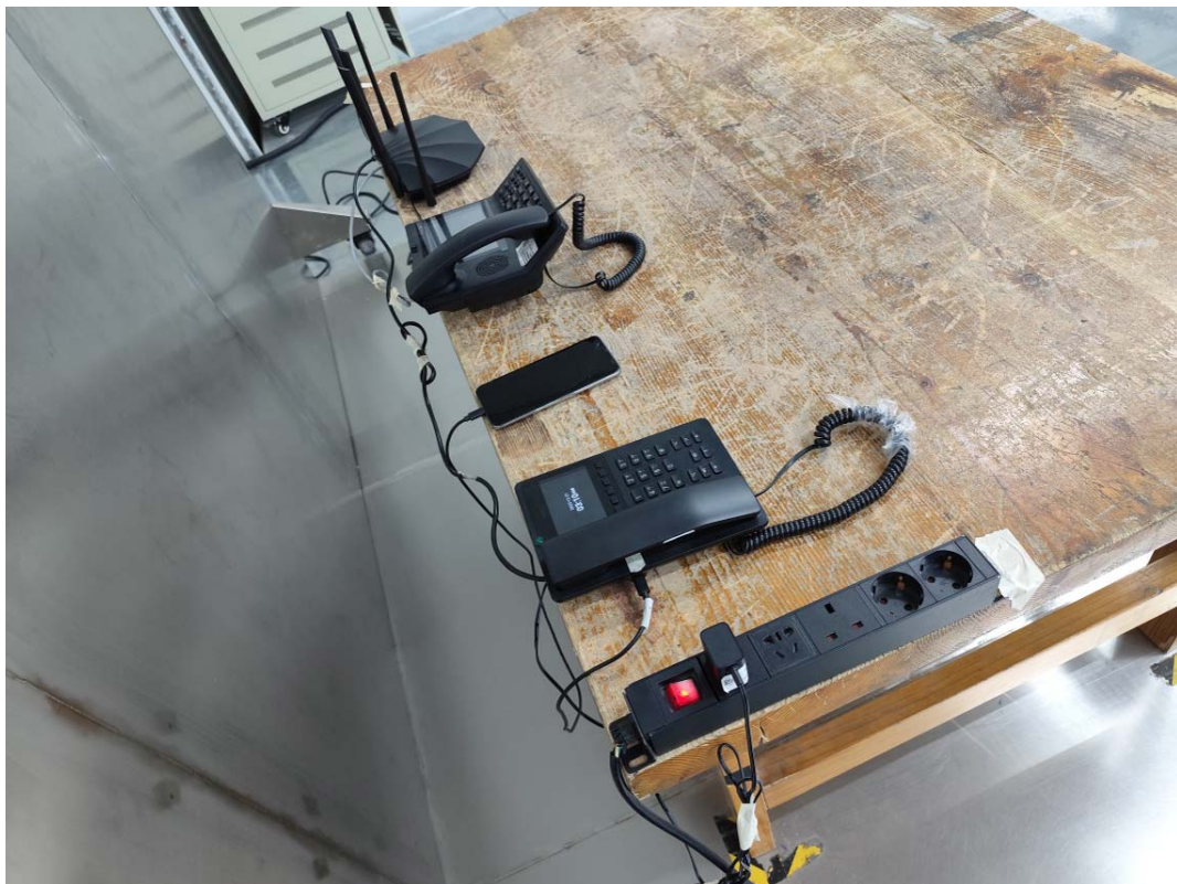
Conducted Emissions Side View-M2&M3
