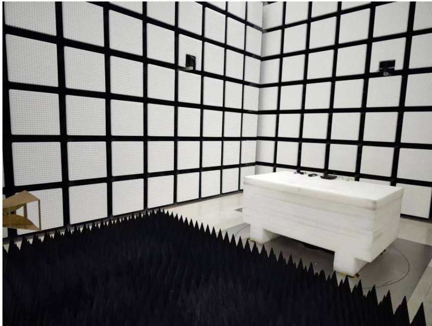
Radiated Emissions Above 1G rear View for PoE
