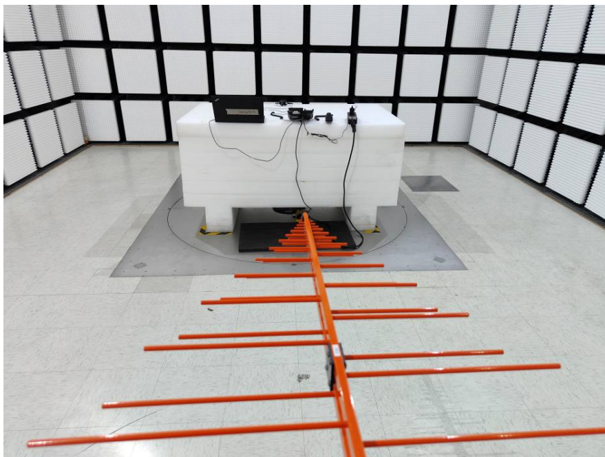
Radiated Emissions Below 1G rear View
