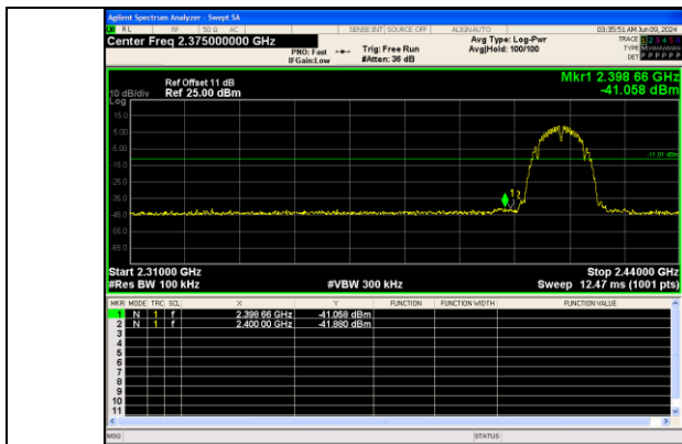
Out Of Band Emission IEEE 802.11b Channel 1 20MHz Antenna 0
