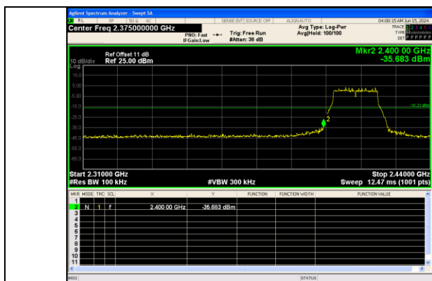
Out Of Band Emission IEEE 802.11g Channel 1 20MHz Antenna 0
