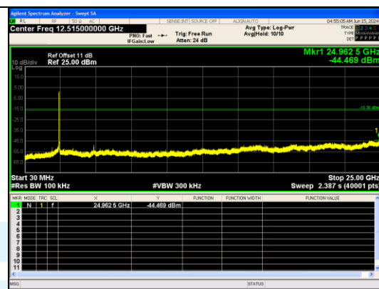
30.0 MHz - 25000.0 MHz IEEE 802.11ax Channel 6 20MHz Antenna 0 RU&Index SU
