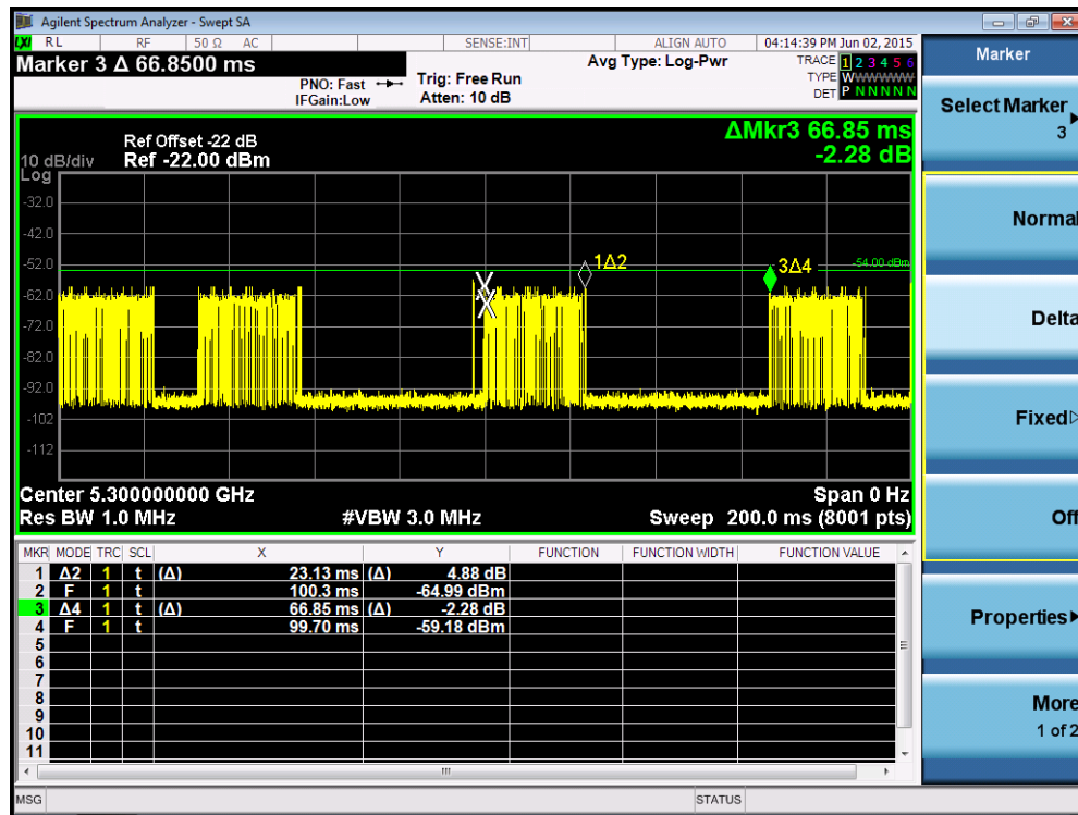
Channel Loading Plot - 802.11n-HT20 - 5300MHz
