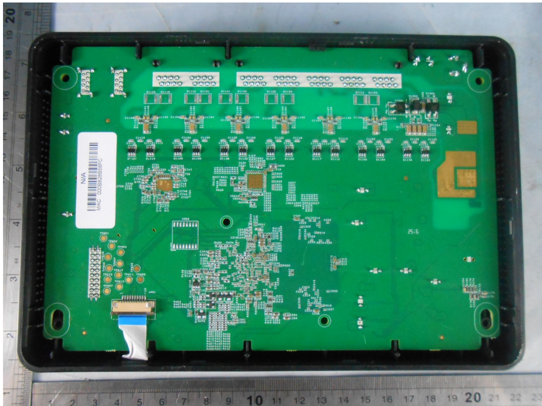
EUT-Uncovered View
