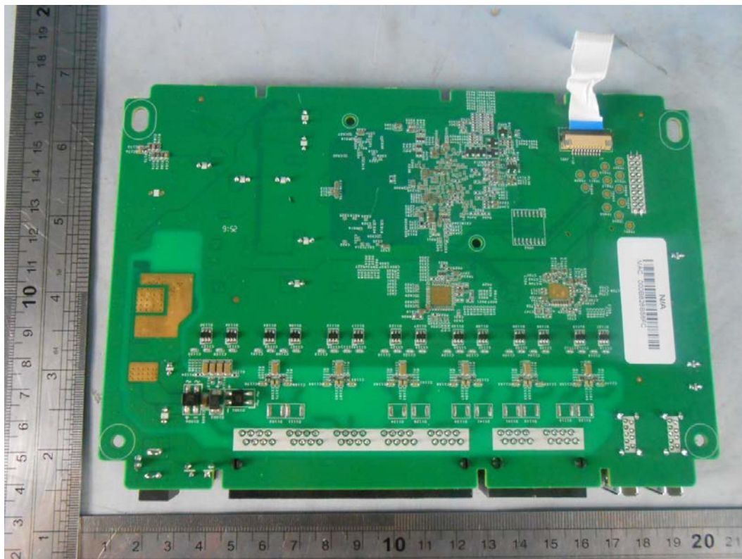
Mainboard-Bottom view -01
