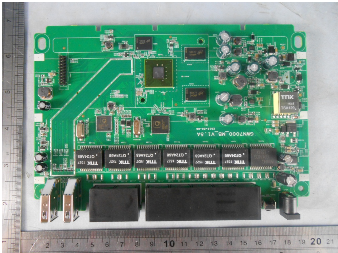
Mainboard-Top view
