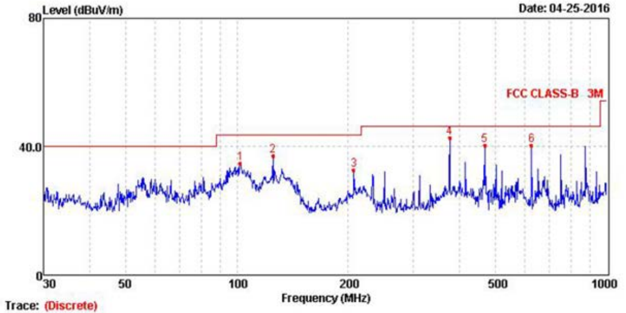
Horizontal: Radiated Emission Test Plot-(30-1000MHz)
