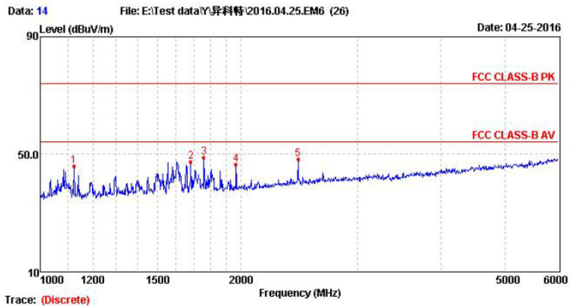
Vertical: Radiated Emission Test Plot(1-6GHz)
