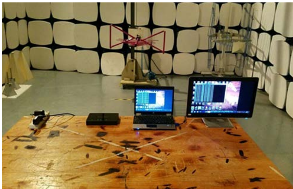
Radiated Emission Test Set-up(30-1000MHz)
