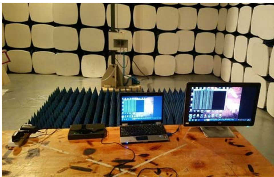
Radiated Emission Test Set-up(Above 1GHz)
