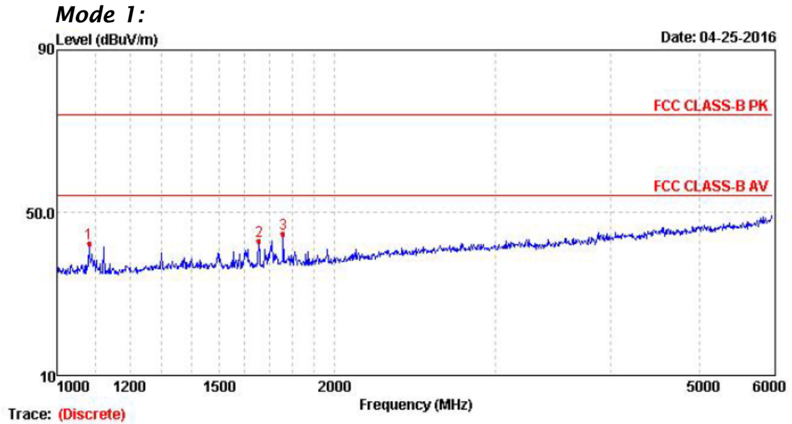
Horizontal: Radiated Emission Test Plot(1-6GHz)
