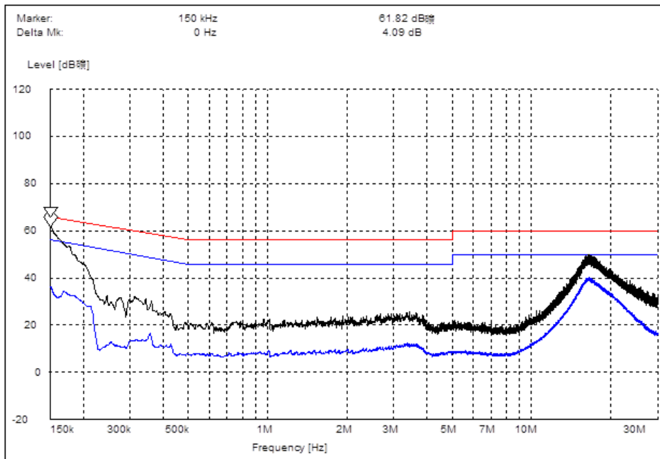
Line N Conducted Emission Graph
