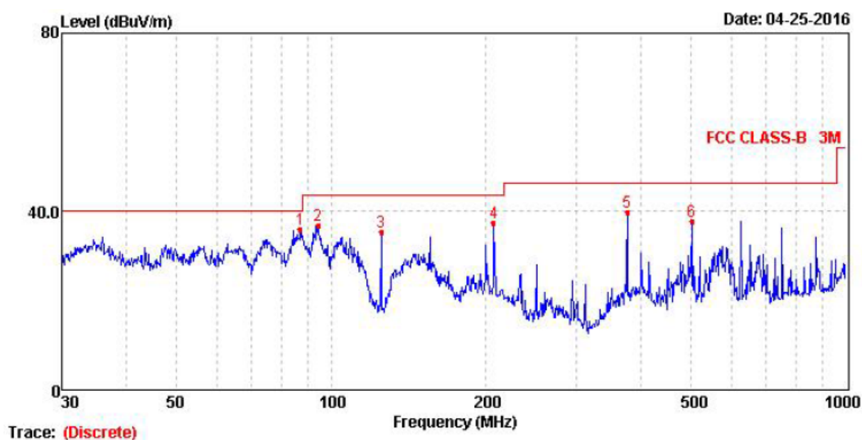
Vertical: Radiated Emission Test Plot(30-1000MHz)
