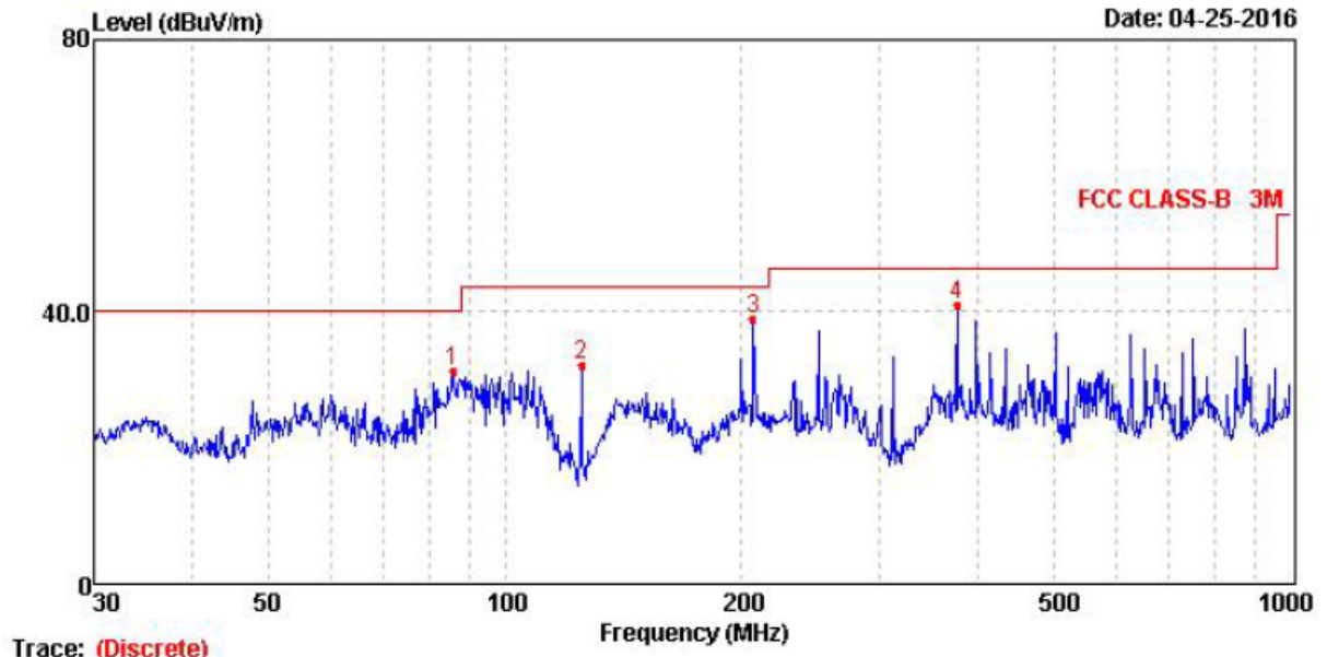
Horizontal: Radiated Emission Test Plot(30-1000MHz)
