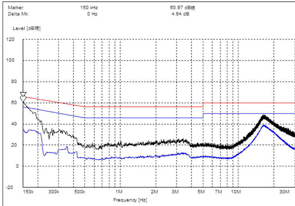
Line L Conducted Emission Graph
