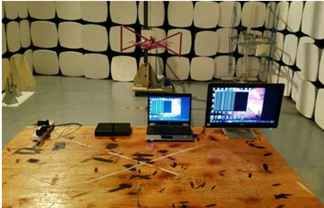
Radiated Emission Test Set-up(30-1000MHz)
