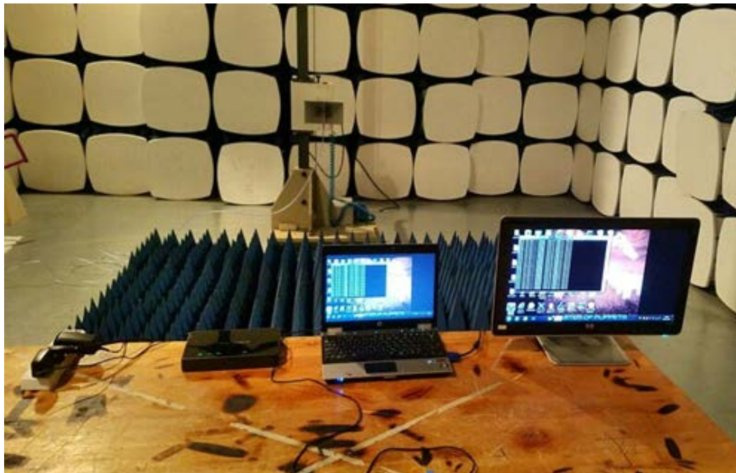
Radiated Emission Test Set-up(Above 1GHz)
