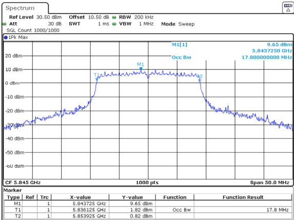
802.11ac20_5845MHz_Chain 1
