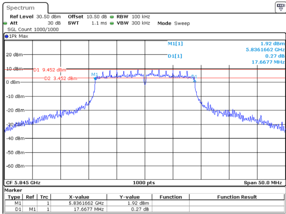
802.11ac20_5845MHz_Chain 0
