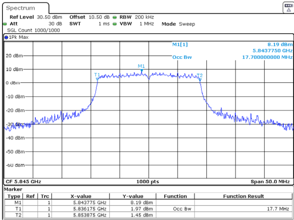
802.11ac20_5845MHz_Chain 2
