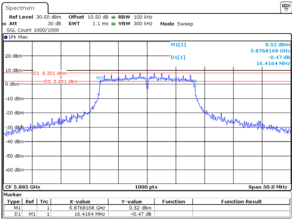
802.11a_5885MHz_Chain 2
