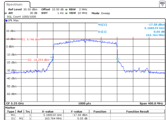
802.11ax160_5250MHz_RU_Full_Chain 2 163.764MHz
