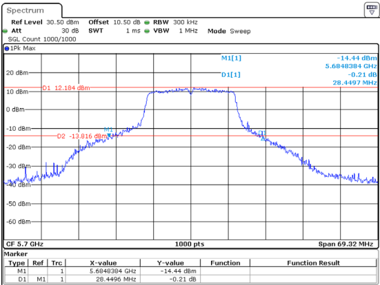
802.11a_5700MHz_Chain 1 28.450MHz
