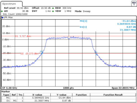
802.11ac20_5580MHz_Chain 1 21.301MHz
