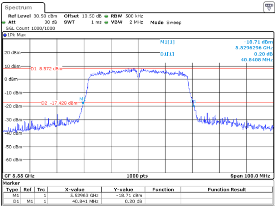
802.11ac40_5550MHz_Chain 1 40.841MHz
