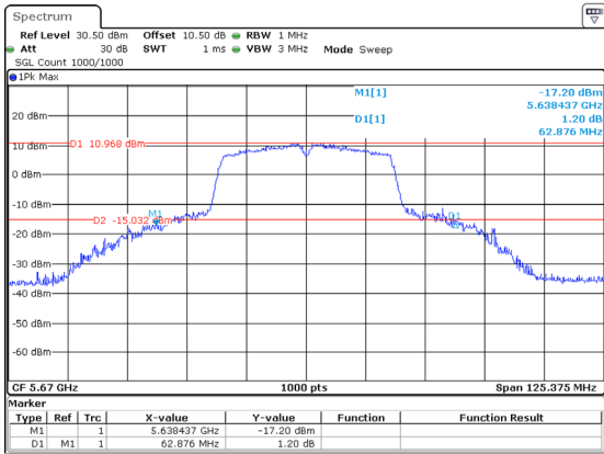
802.11ac40_5670MHz_Chain 1 62.876MHz
