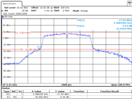
802.11ac40_5510MHz_Chain 1 45.946MHz
