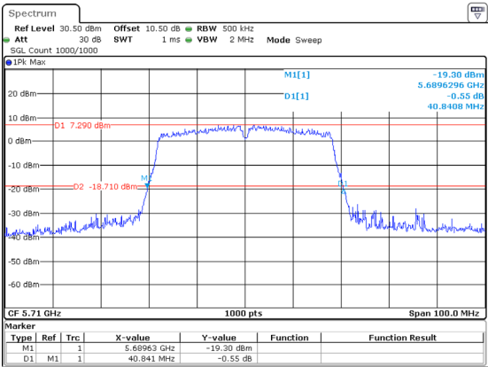
802.11ac40_5710MHz_Chain 2 40.841MHz
