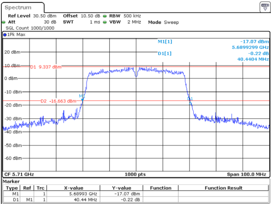
802.11ac40_5710MHz_Chain 1 40.440MHz
