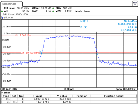
802.11ac40_5710MHz_Chain 0 41.041MHz
