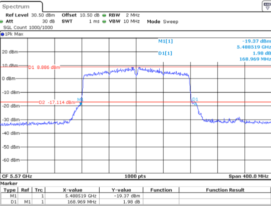
802.11ac160_5570MHz_Chain 0 168.969MHz
