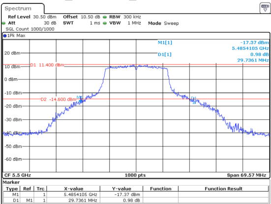
802.11a_5500MHz_Chain 2 29.736MHz
