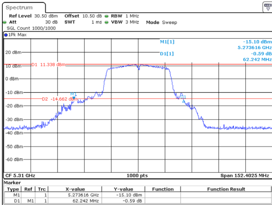
802.11ac40_5310MHz_Chain 0 62.242MHz
