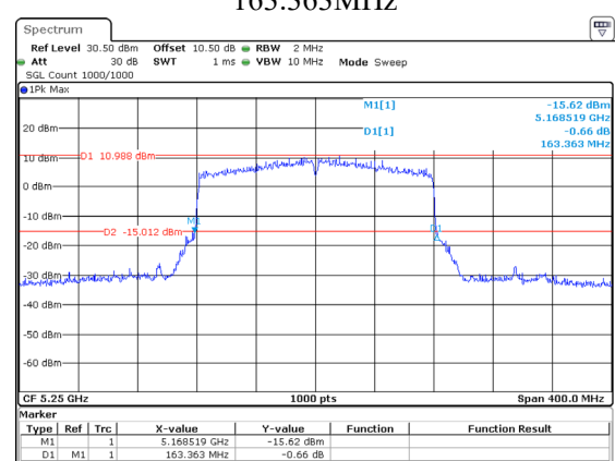
802.11ax160_5250MHz_RU_Full_Chain 0 163.363MHz
