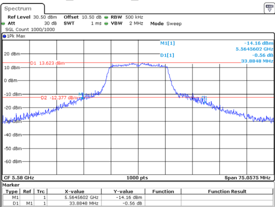
802.11a_5580MHz_Chain 2 33.885MHz
