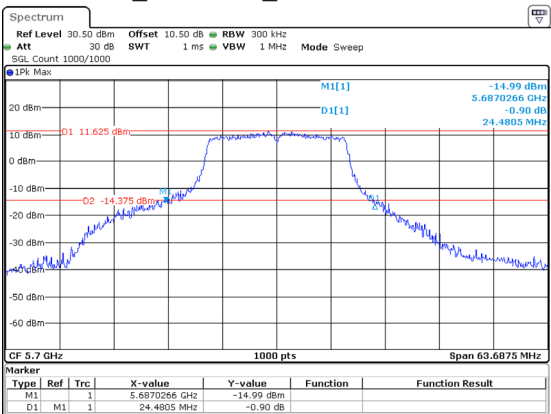
802.11a_5700MHz_Chain 2 24.480MHz
