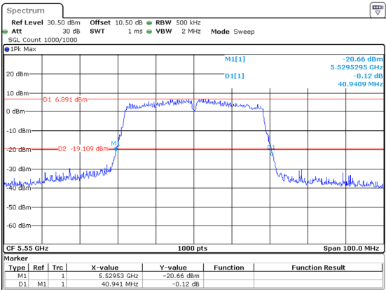
802.11ac40_5550MHz_Chain 2 40.941MHz
