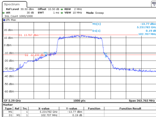
802.11ac80_5290MHz_Chain 0 102.707MHz
