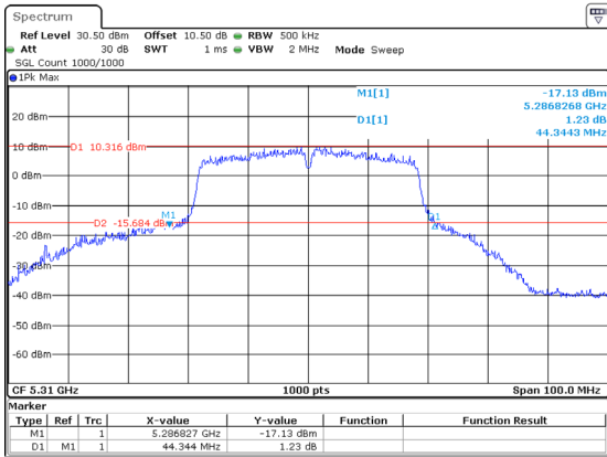
802.11ac40_5310MHz_Chain 1 44.344MHz
