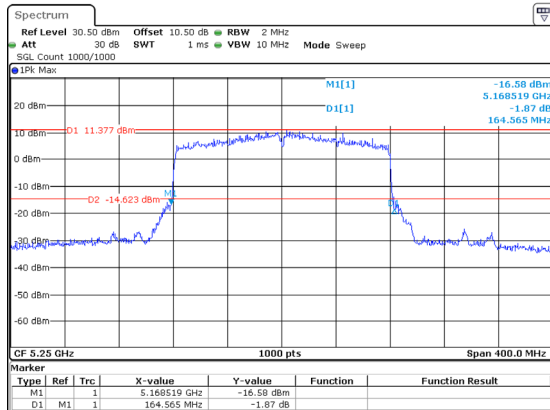
802.11ax160_5250MHz_RU_Full_Chain 1 164.565MHz
