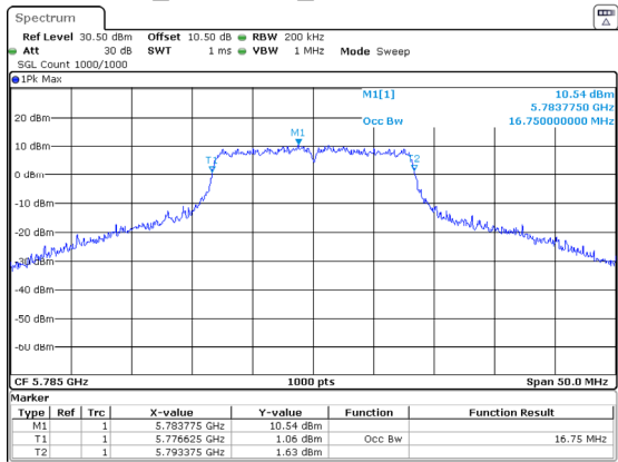
802.11a_5785MHz_Chain 0 16.750MHz
