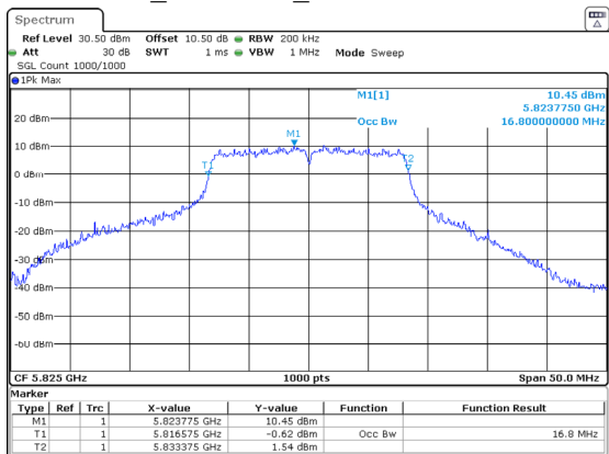
802.11a_5825MHz_Chain 1 16.800MHz
