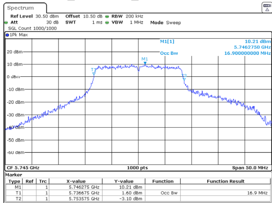
802.11a_5745MHz_Chain 0 16.900MHz
