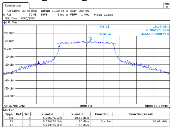
802.11a_5785MHz_Chain 1 16.650MHz
