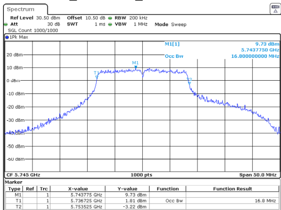
802.11a_5745MHz_Chain 1 16.800MHz
