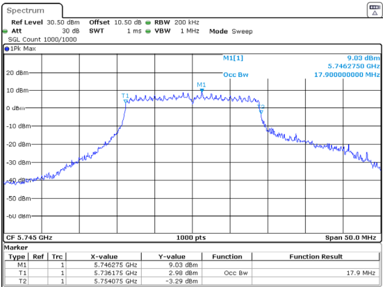
802.11ac20_5745MHz_Chain 1 17.900MHz
