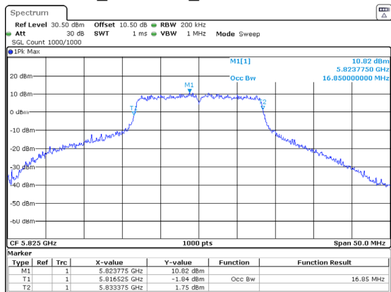
802.11a_5825MHz_Chain 0 16.850MHz
