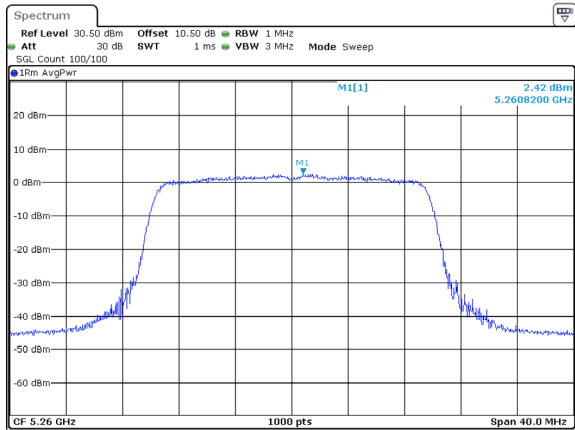
802.11ax20_5260MHz_RU_Full_Chain 1
