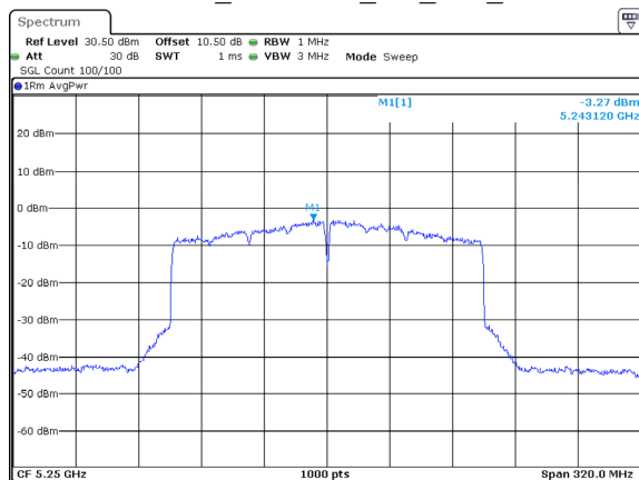
802.11ax160_5250MHz_RU_Full_Chain 1
