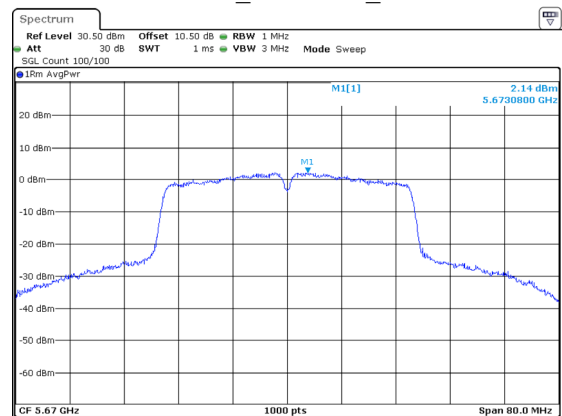
802.11ac40_5670MHz_Chain 0
