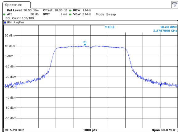
802.11a_5280MHz_Chain 1
