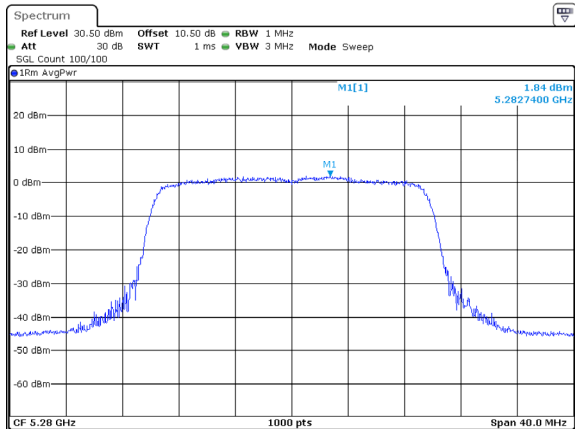
802.11ax20_5280MHz_RU_Full_Chain 0
