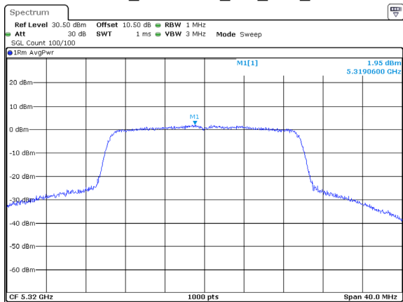
802.11ax20_5320MHz_RU_Full_Chain 1
