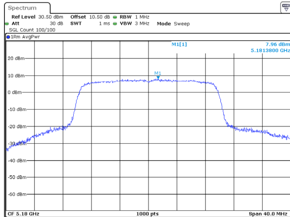
802.11ax20_5180MHz_RU_Full_Chain 1
