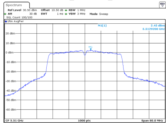
802.11ac40_5510MHz_Chain 0
