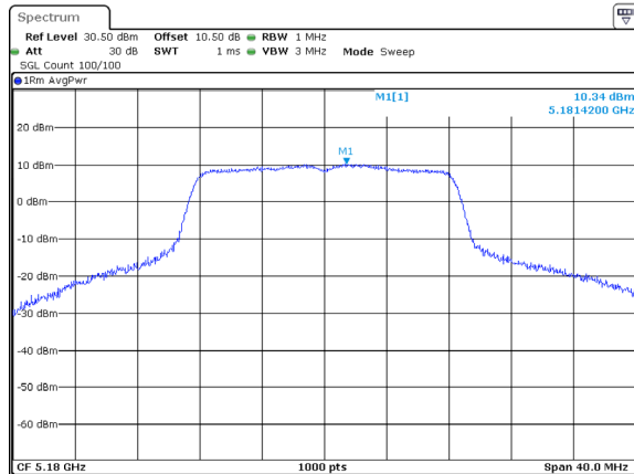
802.11a_5180MHz_Chain 2
