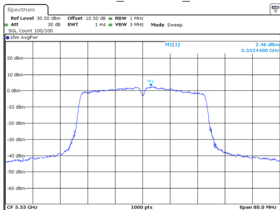
802.11ac40_5550MHz_Chain 0
