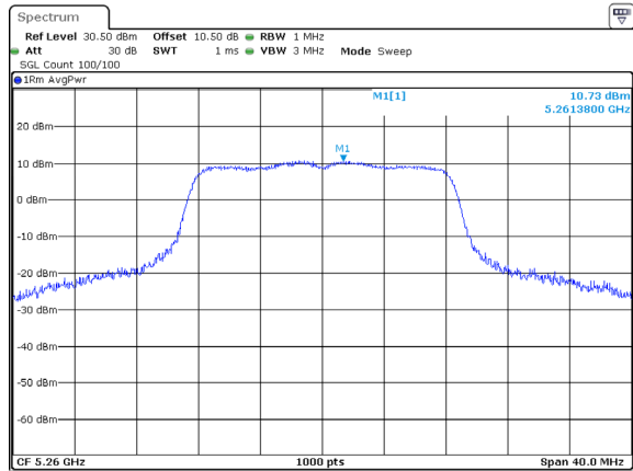
802.11a_5260MHz_Chain 2
