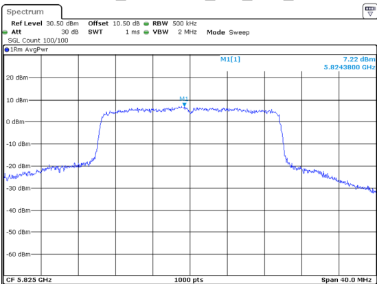
802.11ax20_5825MHz_RU_Full_Chain 1
