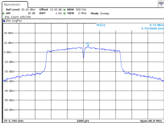
802.11ac40_5795MHz_Chain 0
