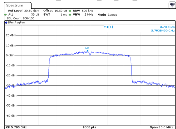
802.11ax40_5795MHz_RU_Full_Chain 2
