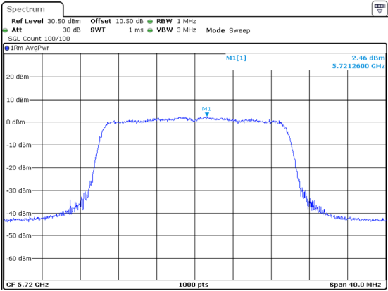
802.11ax20_5720MHz_RU_Full_Chain 0
