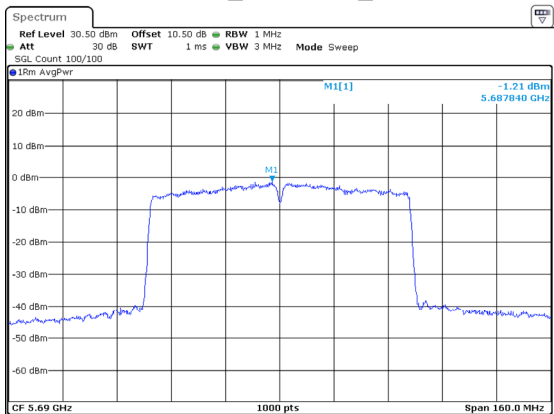
802.11ac80_5690MHz_Chain 1
