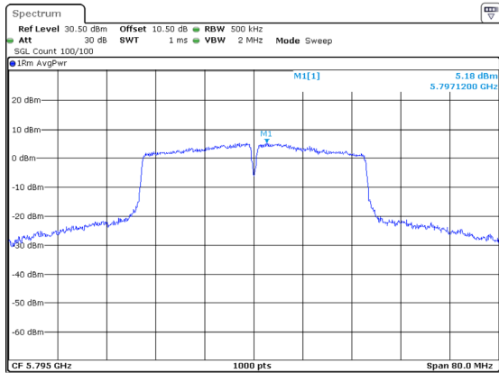
802.11ac40_5795MHz_Chain 1
