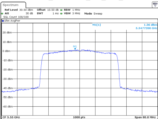
802.11ax40_5550MHz_RU_Full_Chain 1
