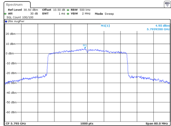
802.11ax40_5795MHz_RU_Full_Chain 1
