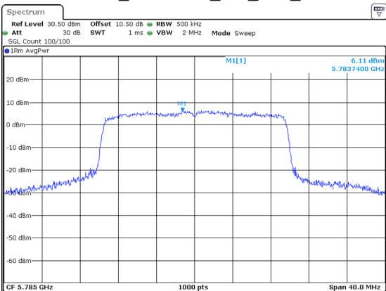
802.11ax20_5785MHz_RU_Full_Chain 2
