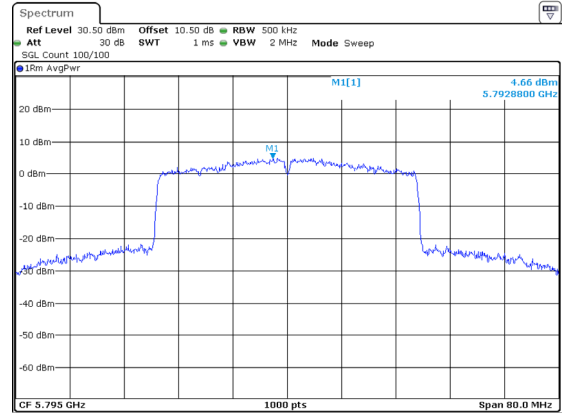
802.11ax40_5795MHz_RU_Full_Chain 0
