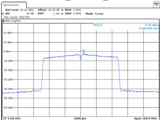
802.11ac80_5690MHz_Chain 2
