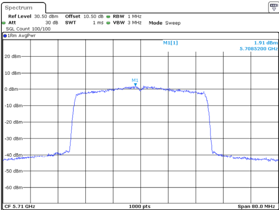
802.11ax40_5710MHz_RU_Full_Chain 0
