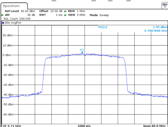
802.11ax40_5710MHz_RU_Full_Chain 1
