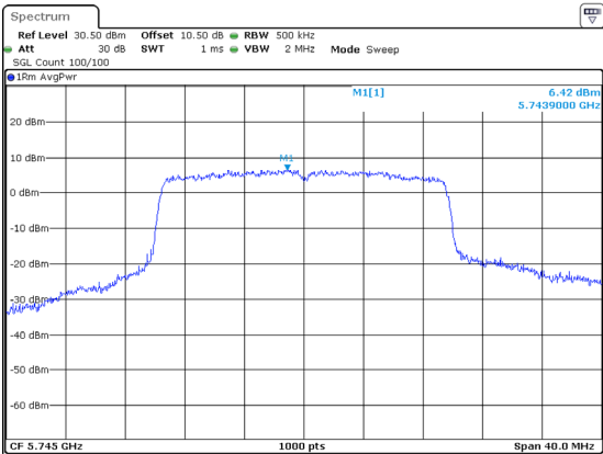
802.11ax20_5745MHz_RU_Full_Chain 1
