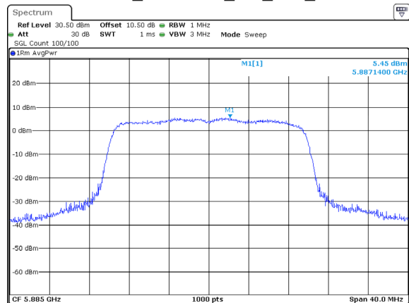
802.11ax20_5885MHz_RU_Full_Chain 1
