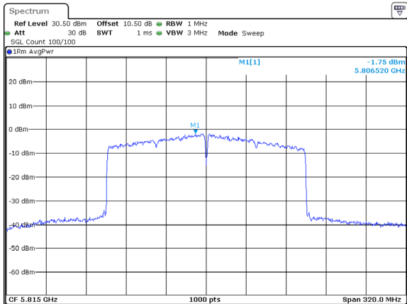
802.11ax160_5815MHz_RU_Full_Chain 1
