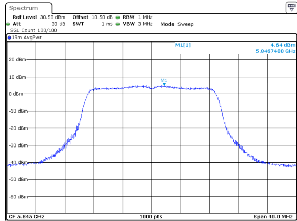
802.11ac20_5845MHz_Chain 2
