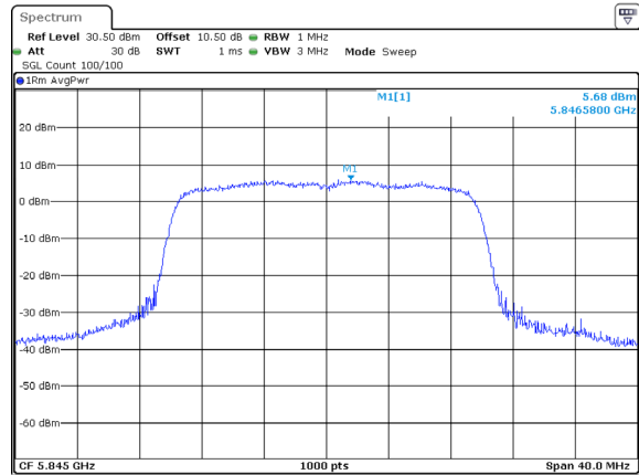
802.11ax20_5845MHz_RU_Full_Chain 1
