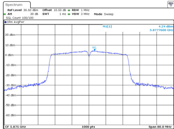
802.11ac40_5875MHz_Chain 2
