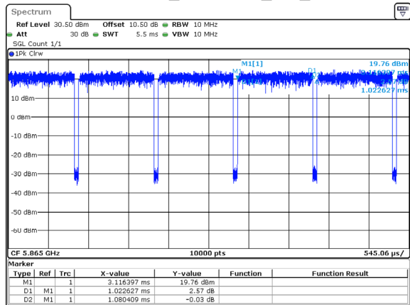
802.11ax20_5865MHz_RU_Full
