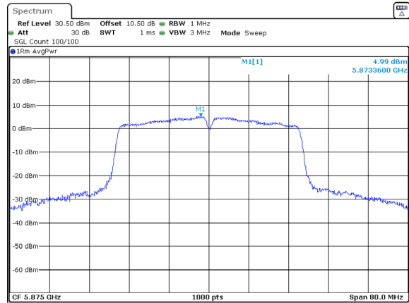
802.11ac40_5875MHz_Chain 1
