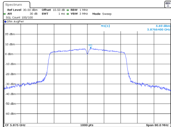
802.11ac40_5875MHz_Chain 0
