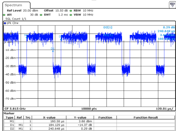
802.11ac160_5815MHz
