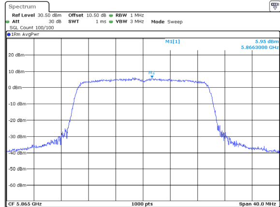
802.11ax20_5865MHz_RU_Full_Chain 0
