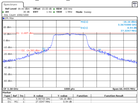
802.11a_5580MHz_Chain 1 27.535MHz
