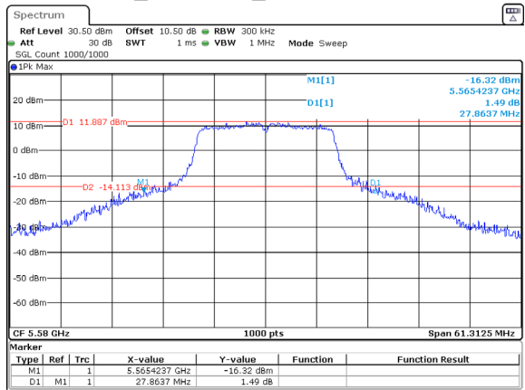
802.11a_5580MHz_Chain 0 27.864MHz
