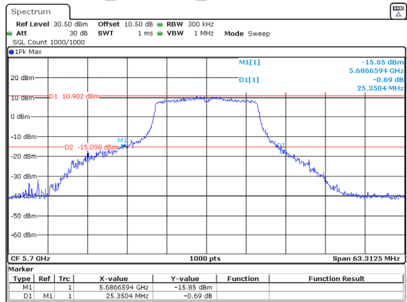
802.11a_5700MHz_Chain 0 25.350MHz
