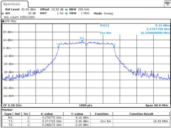
802.11a_5280MHz_Chain 2
