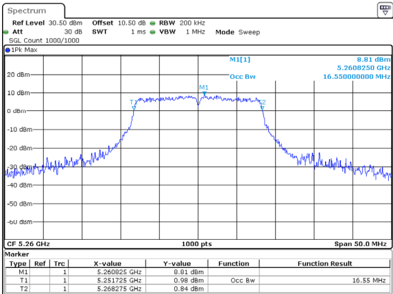
802.11a_5260MHz_Chain 1
