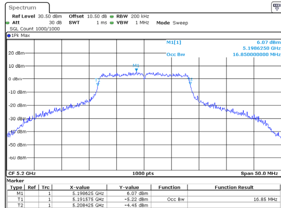
802.11a_5200MHz_Chain 2
