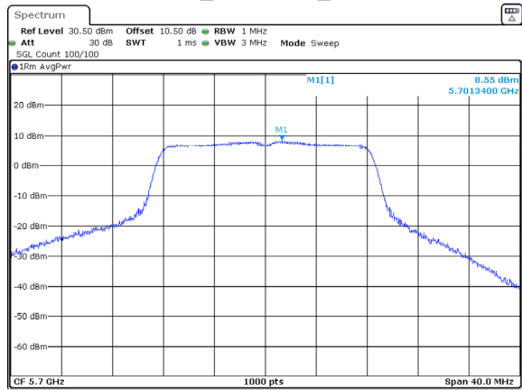
802.11a_5700MHz_Chain 0
