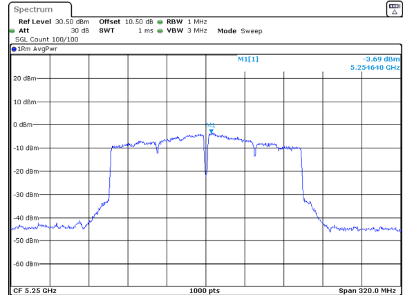
802.11ac160_5250MHz_Chain 1
