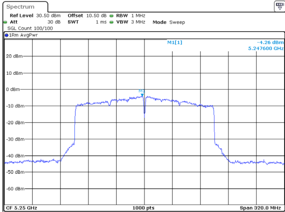
802.11ax160_5250MHz_RU_Full_Chain 0
