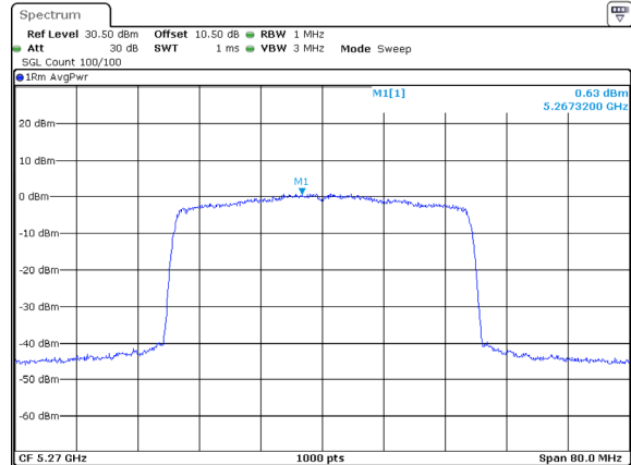
802.11ax40_5270MHz_RU_Full_Chain 2
