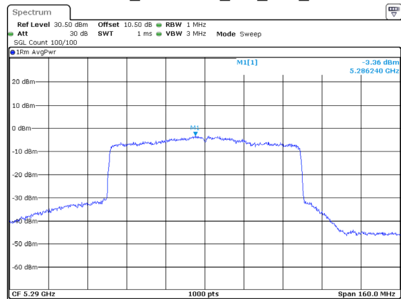
802.11ax80_5290MHz_RU_Full_Chain 2
