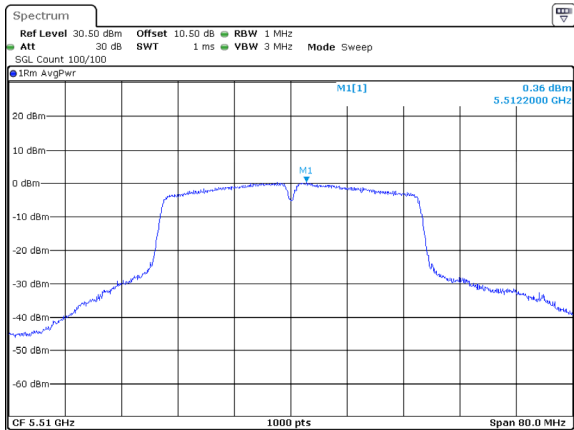
802.11ac40_5510MHz_Chain 2
