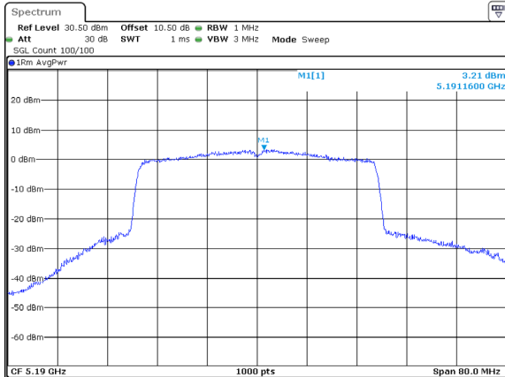
802.11ax40_5190MHz_RU_Full_Chain 0
