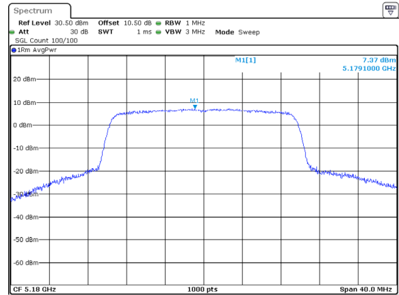
802.11ax20_5180MHz_RU_Full_Chain 0
