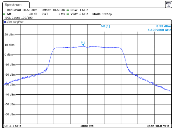
802.11a_5700MHz_Chain 2
