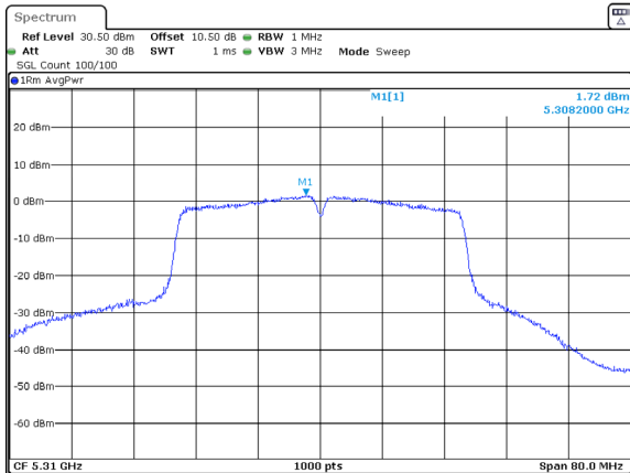
802.11ac40_5310MHz_Chain 0
