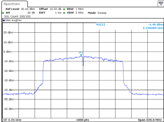
802.11ax160_5250MHz_RU_Full_Chain 2
