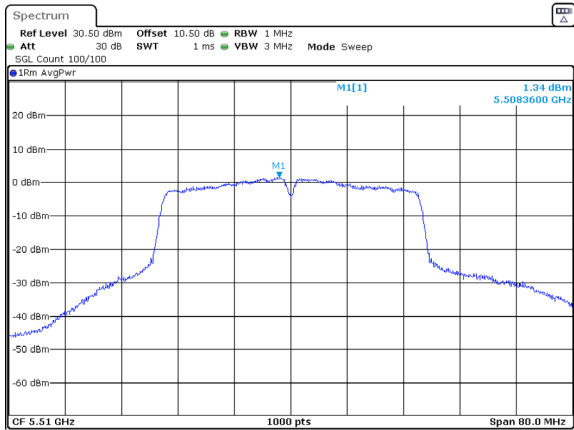
802.11ac40_5510MHz_Chain 0
