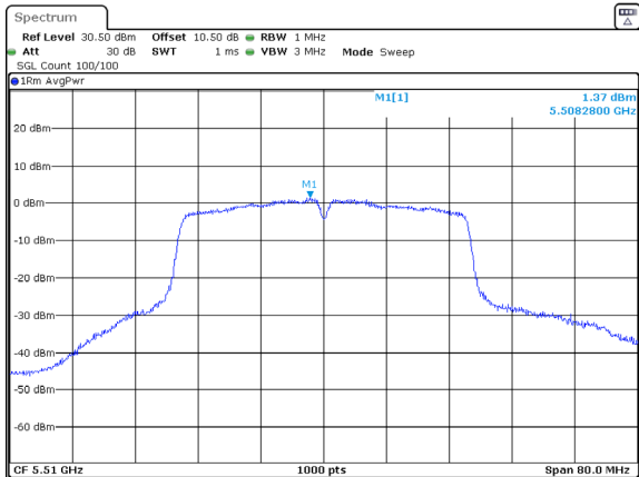
802.11ac40_5510MHz_Chain 1
