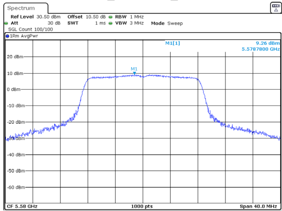
802.11a_5580MHz_Chain 0
