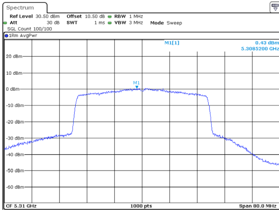
802.11ax40_5310MHz_RU_Full_Chain 2
