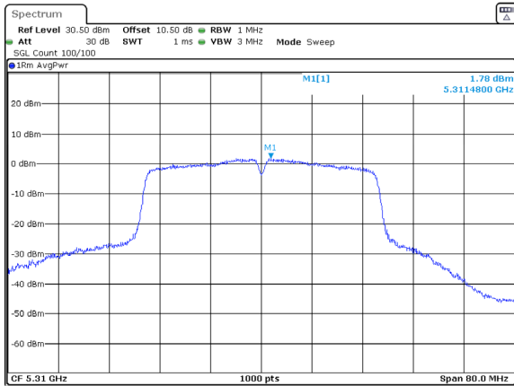
802.11ac40_5310MHz_Chain 1
