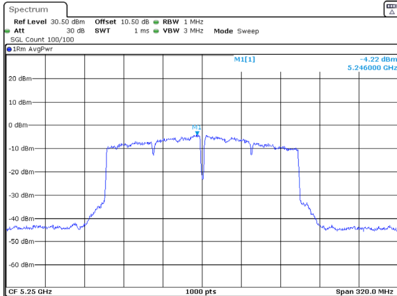
802.11ac160_5250MHz_Chain 0
