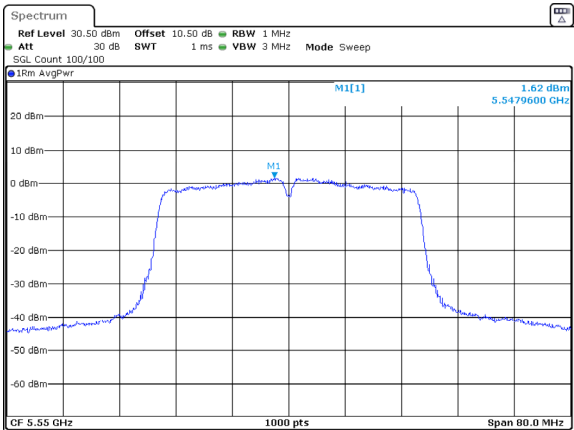
802.11ac40_5550MHz_Chain 0
