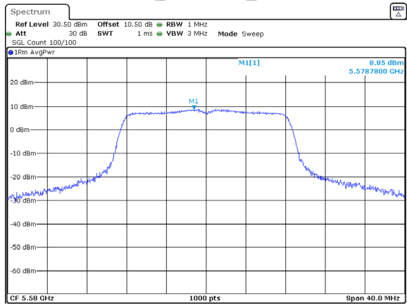
802.11a_5580MHz_Chain 1
