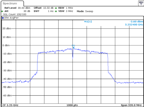
802.11ax160_5250MHz_RU_Full_Chain 1
