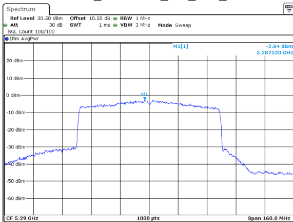
802.11ax80_5290MHz_RU_Full_Chain 1
