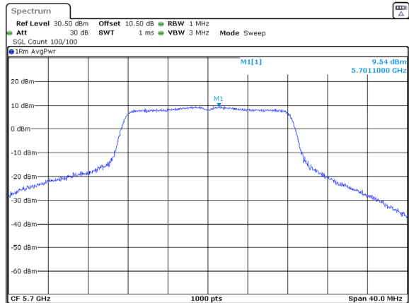
802.11a_5700MHz_Chain 1
