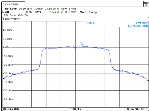
802.11ac40_5670MHz_Chain 0
