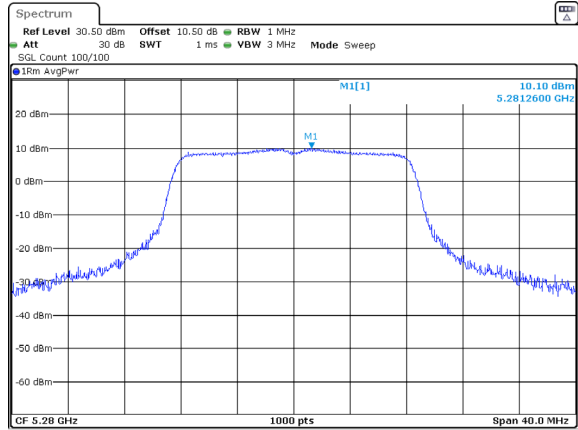
802.11a_5280MHz_Chain 2
