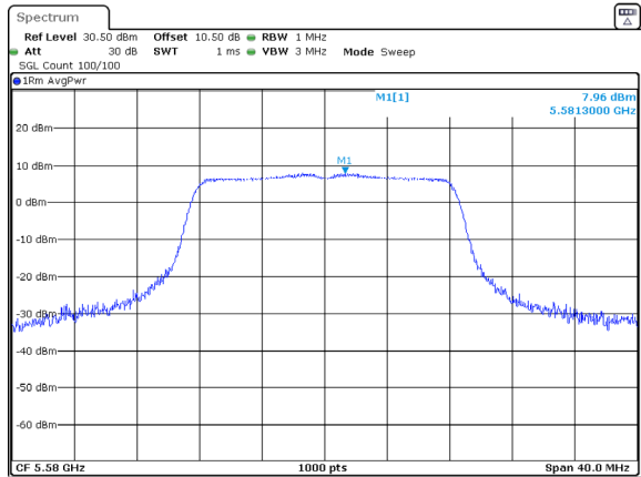
802.11a_5580MHz_Chain 2
