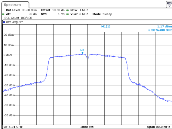
802.11ac40_5310MHz_Chain 2
