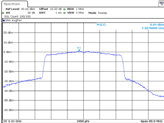
802.11ax40_5310MHz_RU_Full_Chain 1
