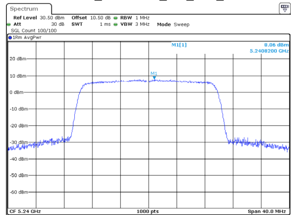
802.11ax20_5240MHz_RU_Full_Chain 0
