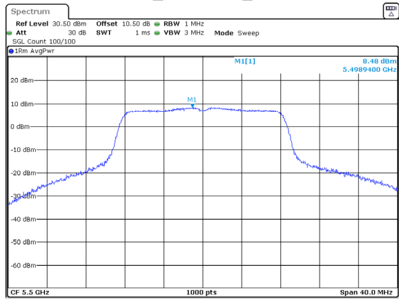
802.11a_5500MHz_Chain 0
