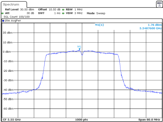
802.11ac40_5550MHz_Chain 1
