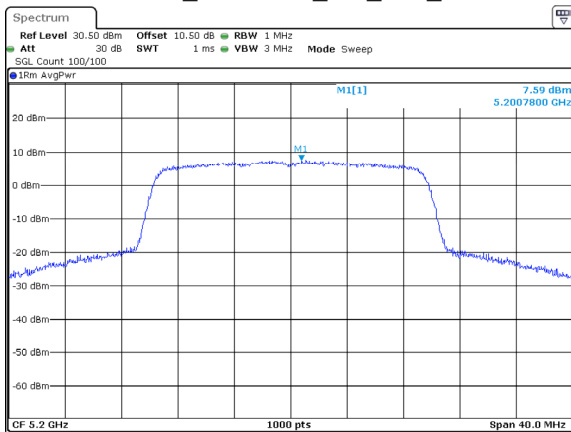
802.11ax20_5200MHz_RU_Full_Chain 0
