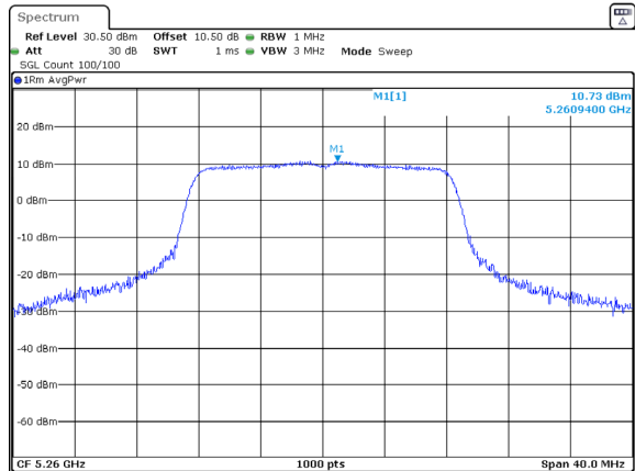
802.11a_5260MHz_Chain 1
