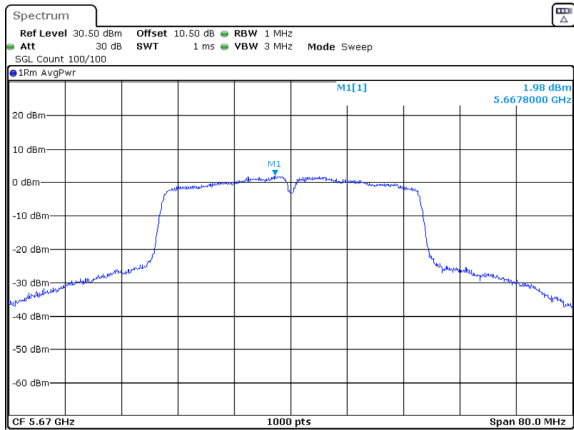
802.11ac40_5670MHz_Chain 1
