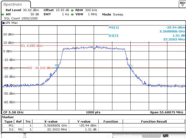
802.11ax20_5580MHz_RU_FULL_Chain 0
