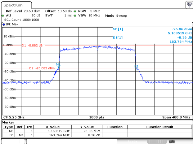
802.11ax160_5250MHz_RU_FULL_Chain 2
