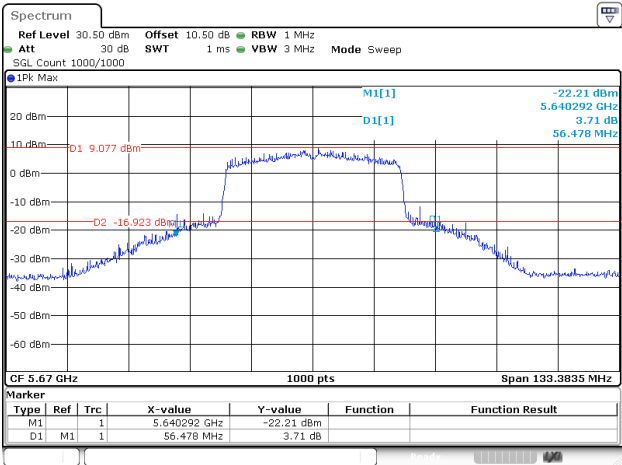
802.11ax40_5670MHz_RU_FULL_Chain 2
