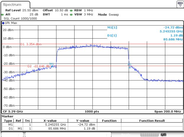
802.11ax80_5290MHz_RU_FULL_Chain 2
