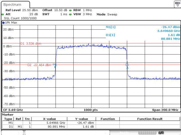
802.11ax80_5690MHz_RU_FULL_Chain 1
