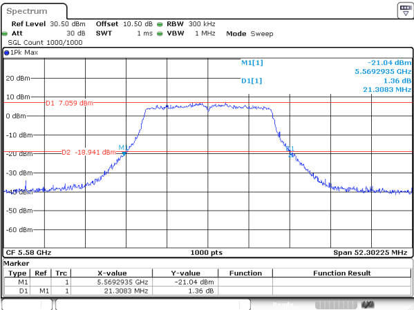
802.11a_5580MHz_Chain 0
