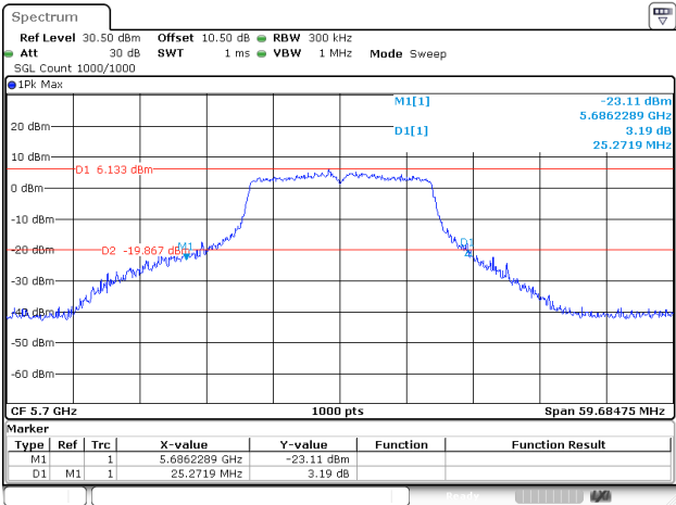
802.11a_5700MHz_Chain 2
