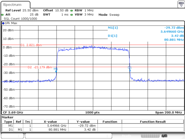
802.11ax80_5690MHz_RU_FULL_Chain 2
