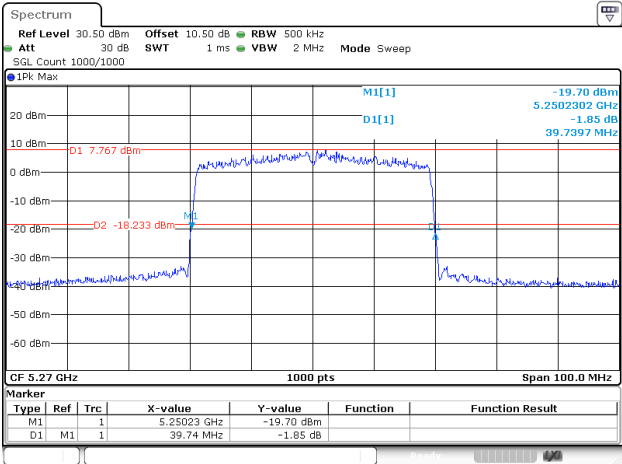
802.11ax40_5270MHz_RU_FULL_Chain 0
