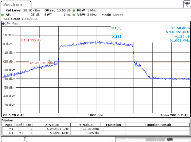
802.11ax80_5290MHz_RU_FULL_Chain 0
