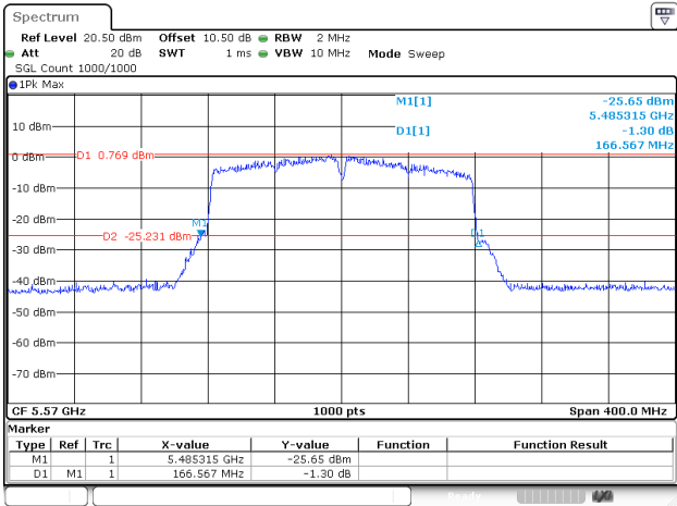
802.11ac160_5570MHz_RU_FULL_Chain 0
