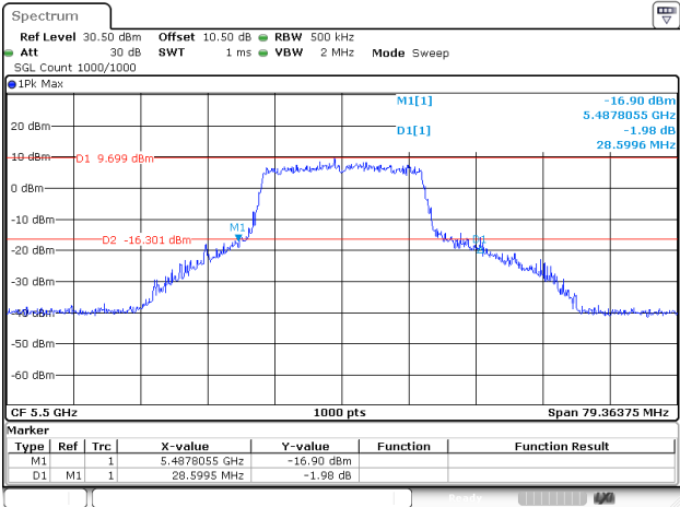
802.11ax20_5500MHz_RU_FULL_Chain 0
