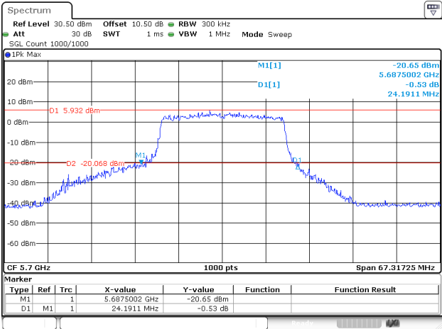
802.11ax20_5700MHz_RU_FULL_Chain 1
