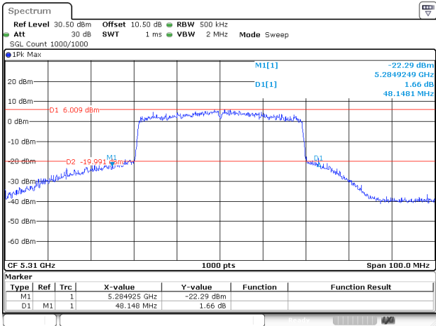
802.11ax40_5310MHz_RU_FULL_Chain 2
