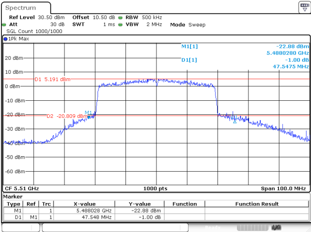
802.11ax40_5510MHz_RU_FULL_Chain 2
