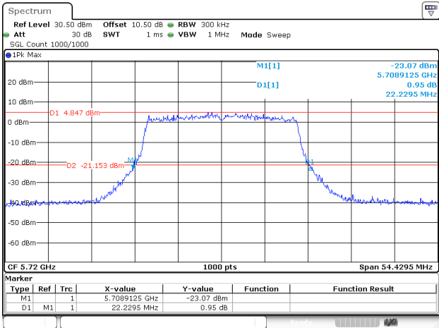
802.11ax20_5720MHz_RU_FULL_Chain 2
