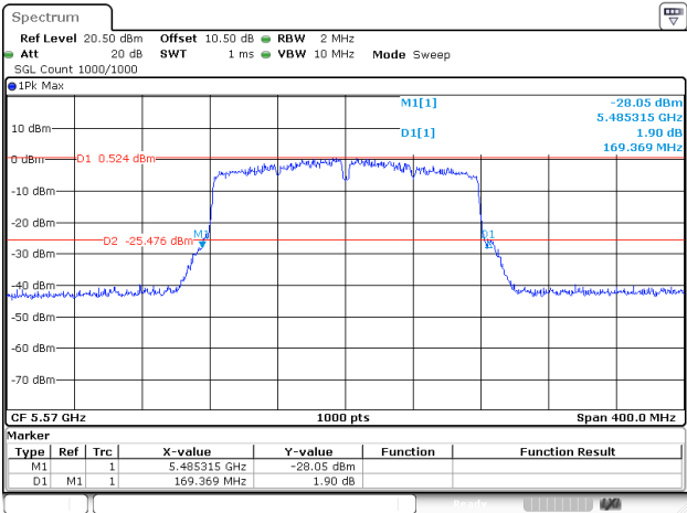
802.11ac160_5570MHz_RU_FULL_Chain 1
