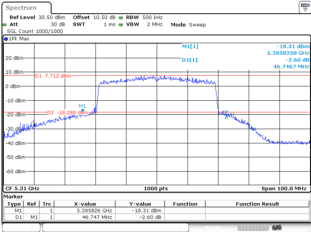
802.11ax40_5310MHz_RU_FULL_Chain 1
