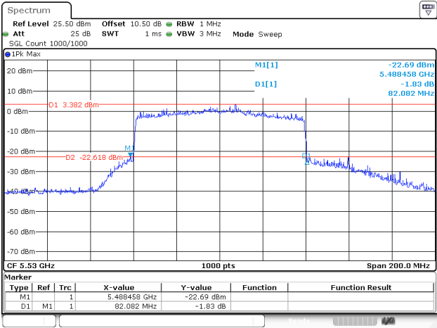
802.11ax80_5530MHz_RU_FULL_Chain 2
