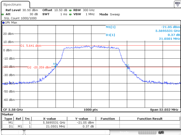
802.11a_5580MHz_Chain 2
