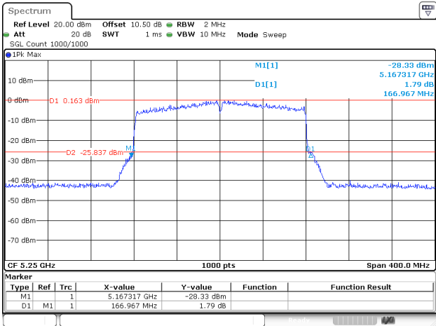
802.11ax160_5250MHz_RU_FULL_Chain 0
