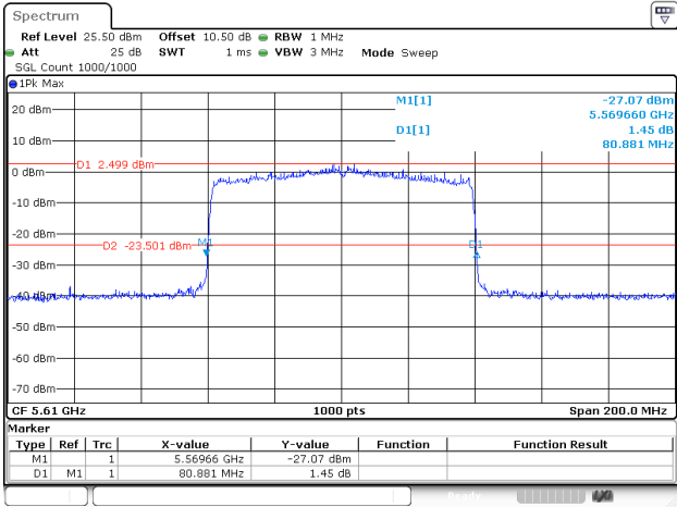
802.11ax80_5610MHz_RU_FULL_Chain 2
