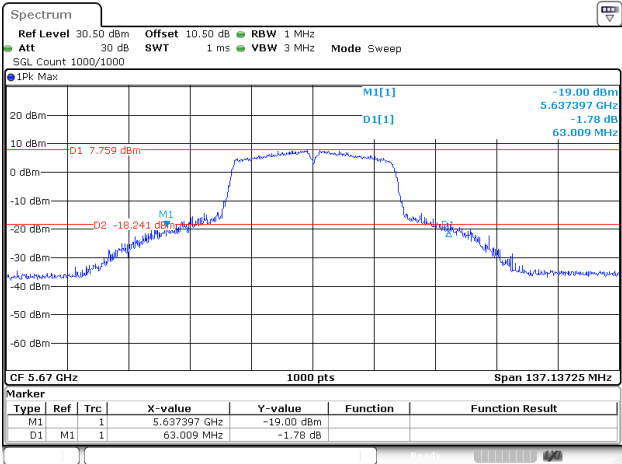
802.11ac40_5670MHz_Chain 1
