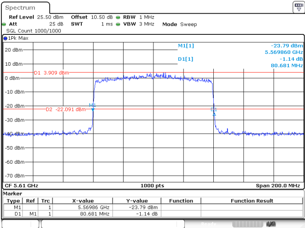
802.11ax80_5610MHz_RU_FULL_Chain 1
