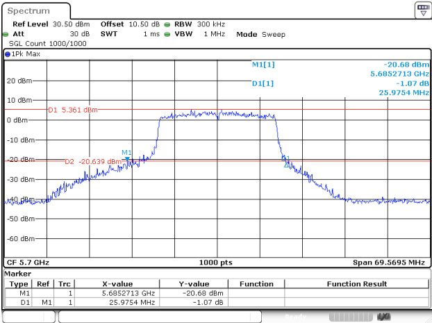
802.11ax20_5700MHz_RU_FULL_Chain 0
