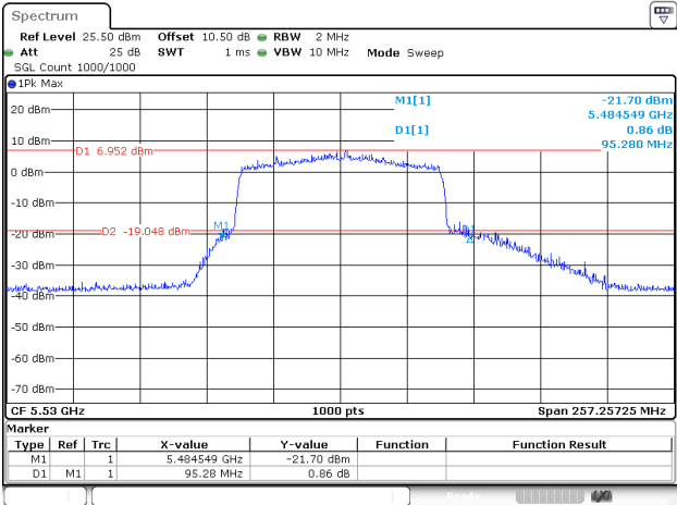
802.11ax80_5530MHz_RU_FULL_Chain 0
