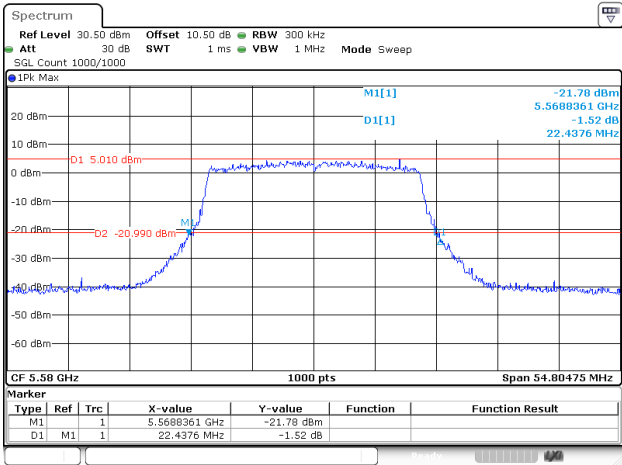
802.11ax20_5580MHz_RU_FULL_Chain 2
