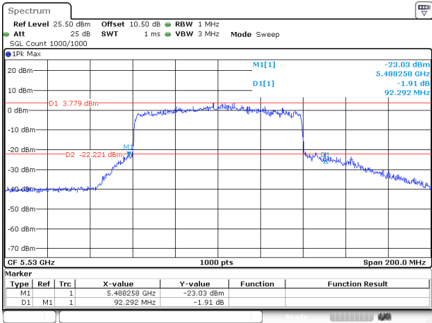
802.11ax80_5530MHz_RU_FULL_Chain 1
