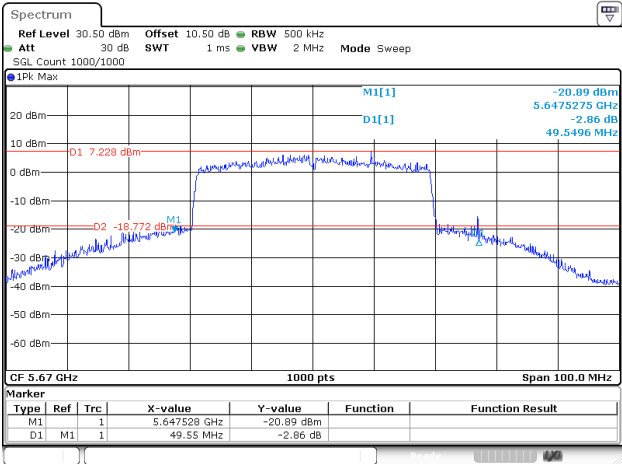
802.11ax40_5670MHz_RU_FULL_Chain 1
