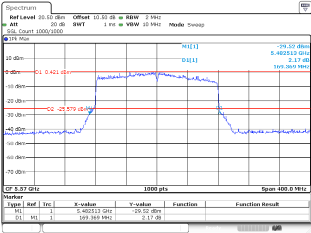
802.11ax160_5570MHz_RU_FULL_Chain 2
