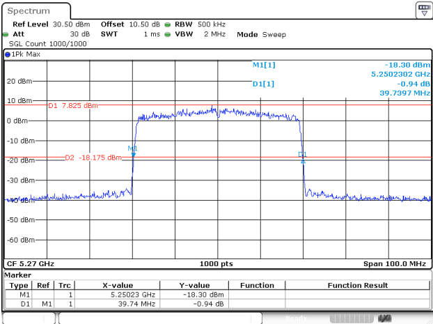
802.11ax40_5270MHz_RU_FULL_Chain 2
