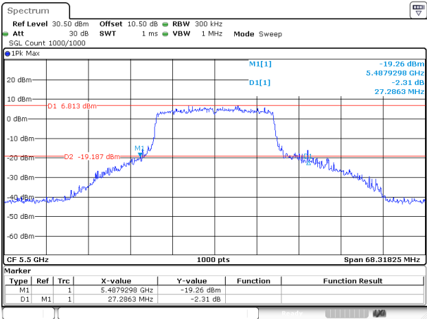
802.11ax20_5500MHz_RU_FULL_Chain 1
