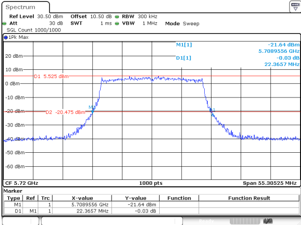
802.11ax20_5720MHz_RU_FULL_Chain 1
