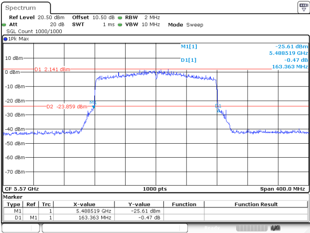
802.11ax160_5570MHz_RU_FULL_Chain 1
