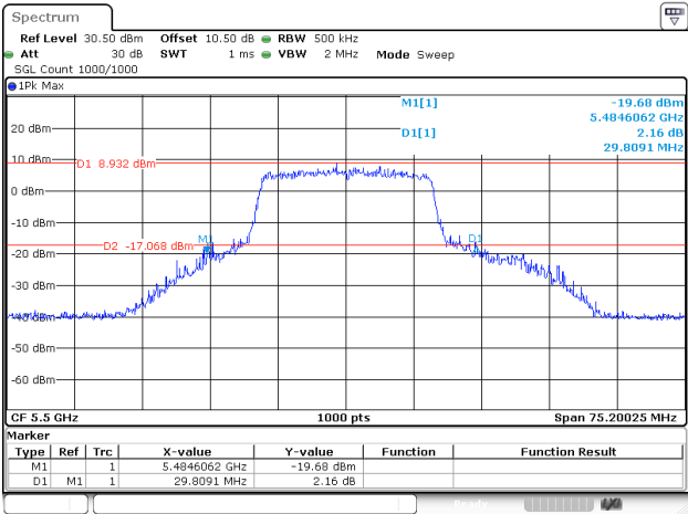
802.11ax20_5500MHz_RU_FULL_Chain 2
