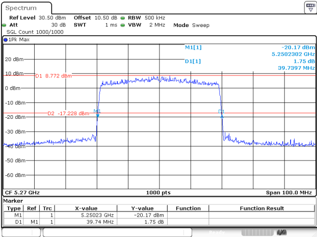
802.11ax40_5270MHz_RU_FULL_Chain 1
