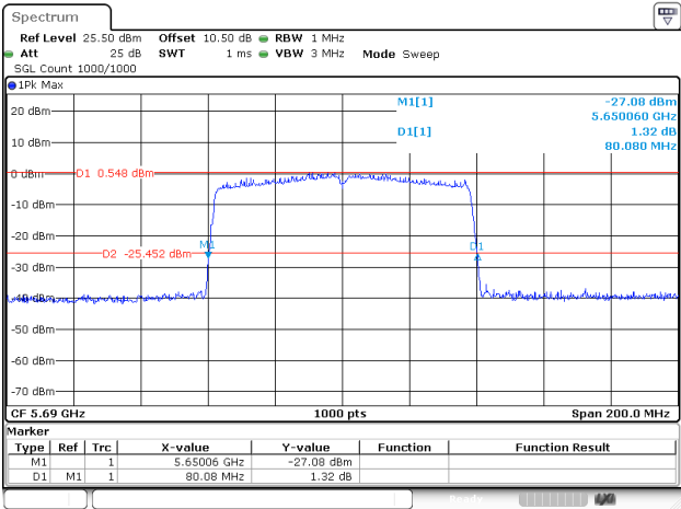
802.11ac80_5690MHz_Chain 2
