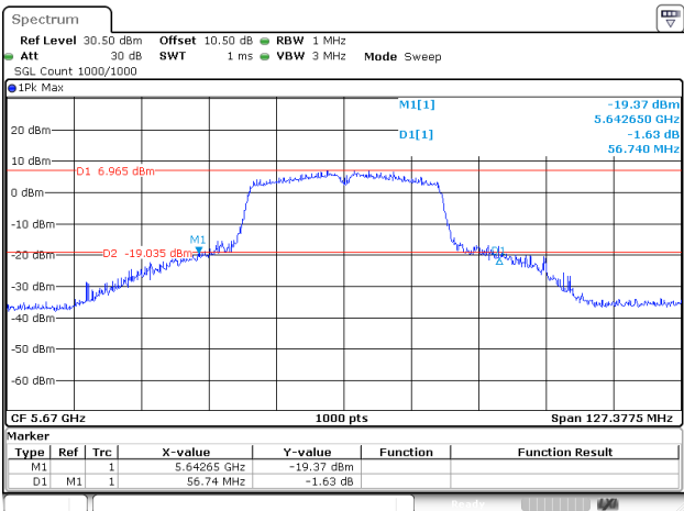
802.11ac40_5670MHz_Chain 2
