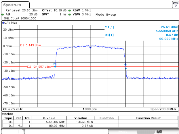
802.11ac80_5690MHz_Chain 1
