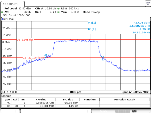
802.11ax20_5700MHz_RU_FULL_Chain 2
