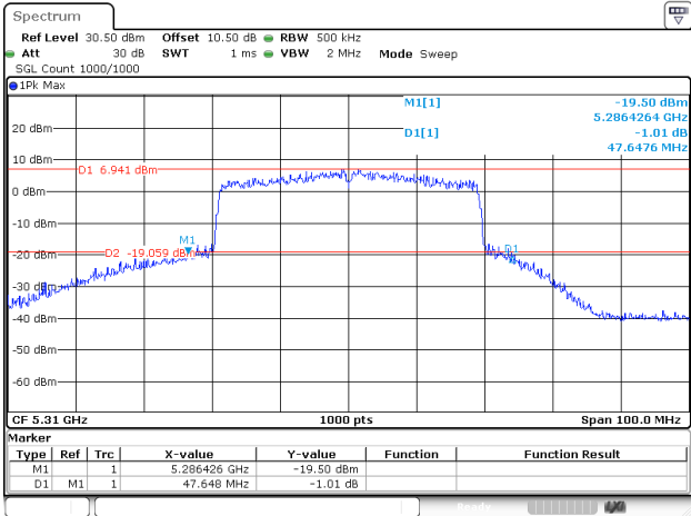
802.11ax40_5310MHz_RU_FULL_Chain 0
