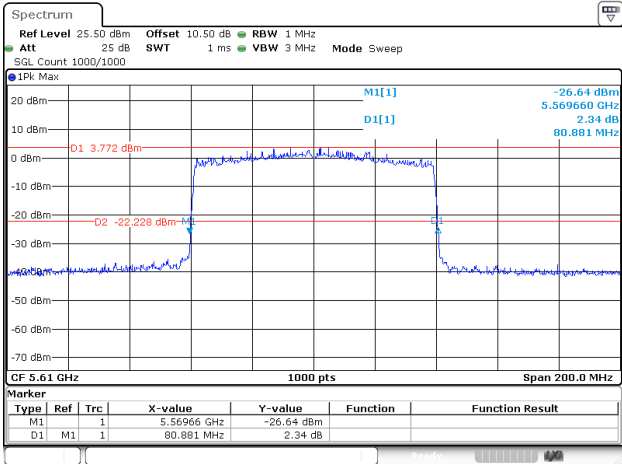
802.11ax80_5610MHz_RU_FULL_Chain 0
