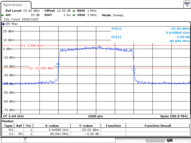
802.11ax80_5690MHz_RU_FULL_Chain 0
