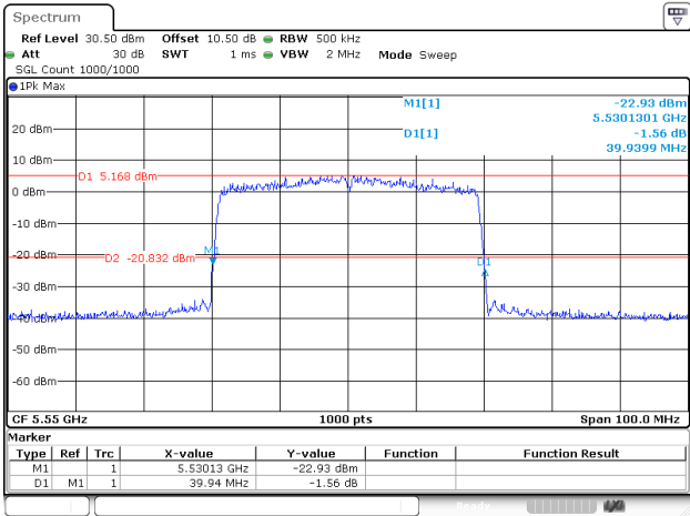
802.11ax40_5550MHz_RU_FULL_Chain 2
