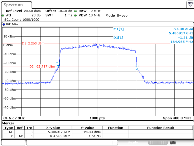
802.11ax160_5570MHz_RU_FULL_Chain 0
