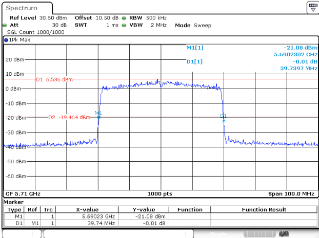
802.11ax40_5710MHz_RU_FULL_Chain 2
