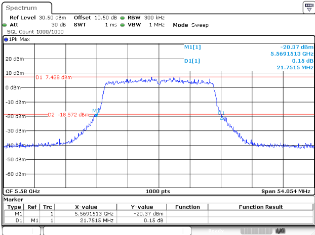
802.11ax20_5580MHz_RU_FULL_Chain 1
