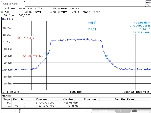
802.11ax20_5720MHz_RU_FULL_Chain 0
