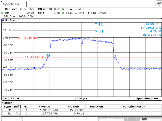
802.11ac160_5570MHz_RU_FULL_Chain 2
