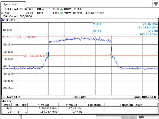
802.11ax160_5250MHz_RU_FULL_Chain 1
