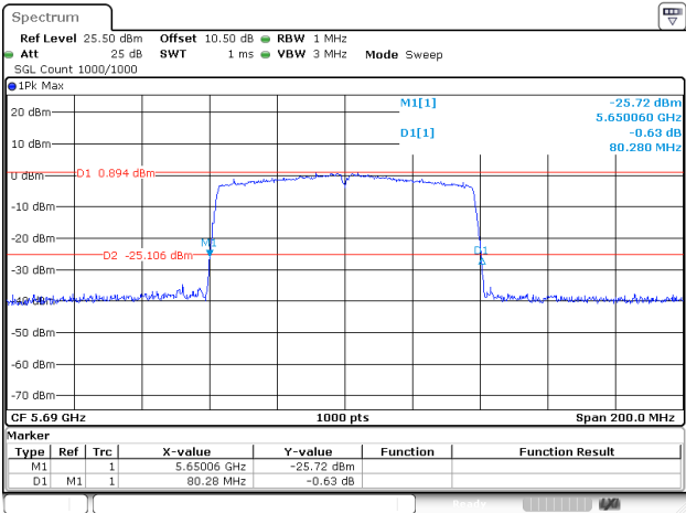
802.11ac80_5690MHz_Chain 0
