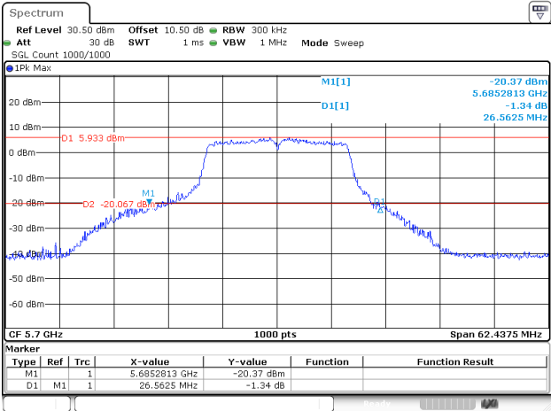
802.11a_5700MHz_Chain 1
