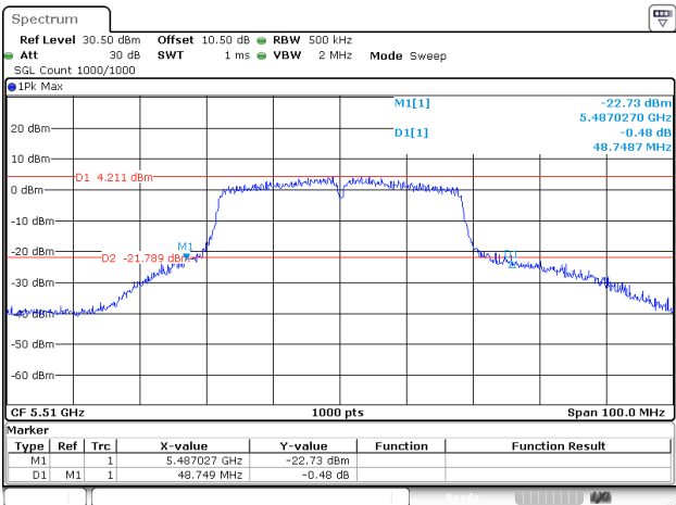
802.11ac40_5510MHz_Chain 2
