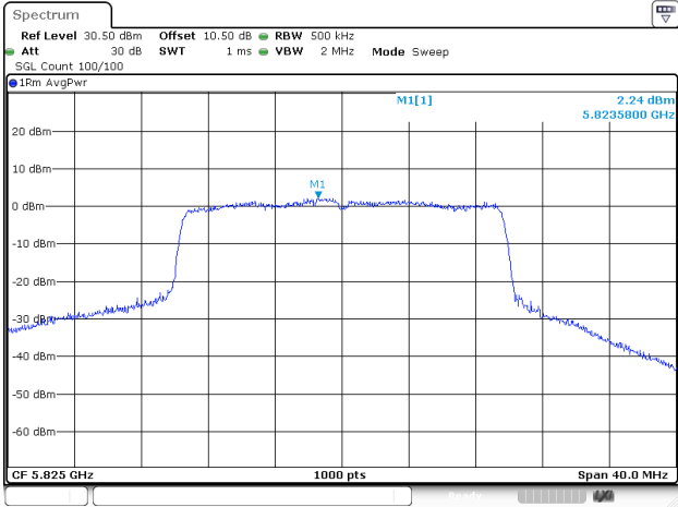
802.11ax20_5825MHz_RU_FULL_Chain 2
