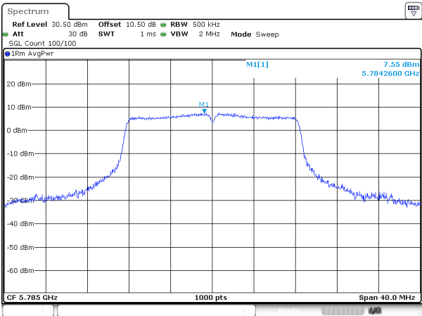
802.11a_5785MHz_Chain 1
