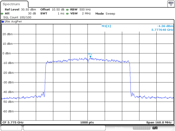
802.11ax80_5775MHz_RU_FULL_Chain 1
