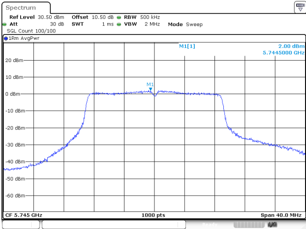
802.11ac20_5745MHz_Chain 2
