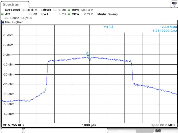
802.11ax40_5755MHz_RU_FULL_Chain 2
