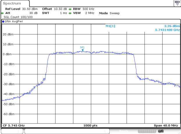
802.11ax20_5745MHz_RU_FULL_Chain 1
