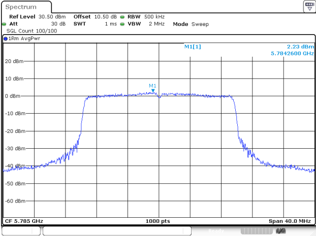
802.11ax20_5785MHz_RU_FULL_Chain 2
