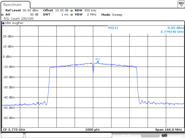
802.11ac80_5775MHz_Chain 2
