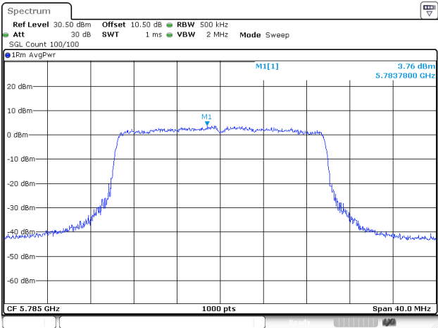
802.11ax20_5785MHz_RU_FULL_Chain 0
