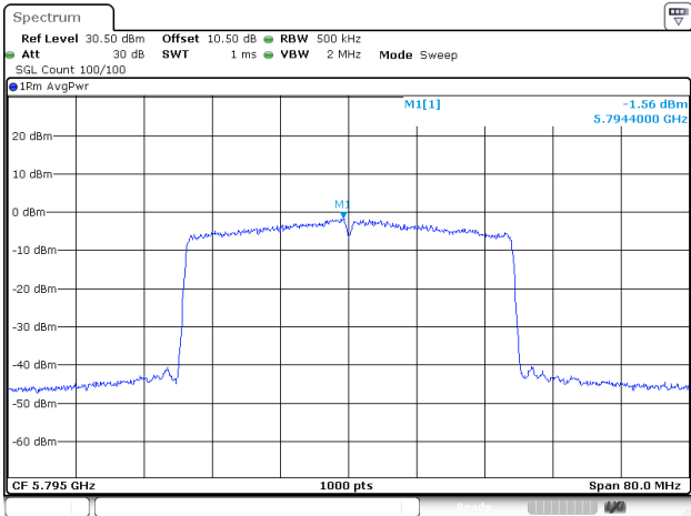
802.11ax40_5795MHz_RU_FULL_Chain 2
