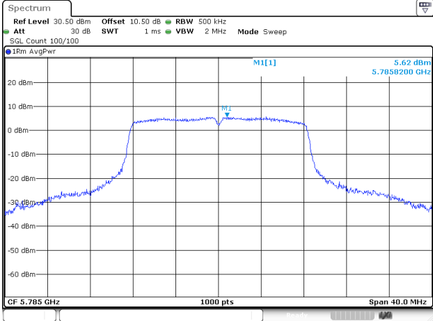
802.11a_5785MHz_Chain 2
