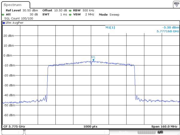
802.11ax80_5775MHz_RU_FULL_Chain 2
