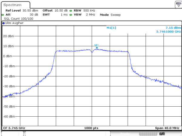
802.11a_5745MHz_Chain 1
