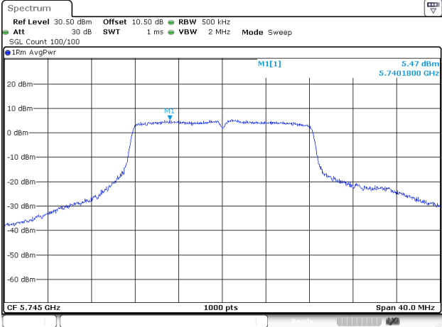
802.11a_5745MHz_Chain 2
