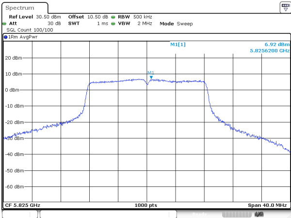
802.11a_5825MHz_Chain 1
