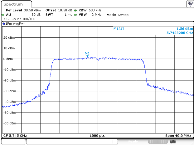
802.11ax20_5745MHz_RU_FULL_Chain 2
