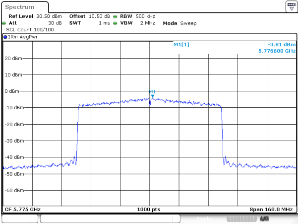
802.11ax80_5775MHz_RU_FULL_Chain 0
