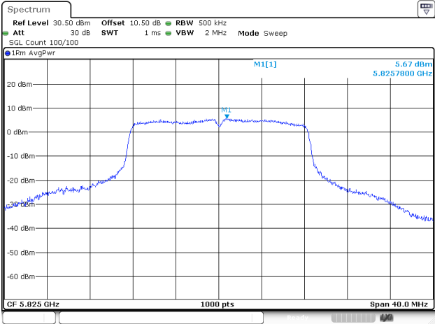
802.11a_5825MHz_Chain 2
