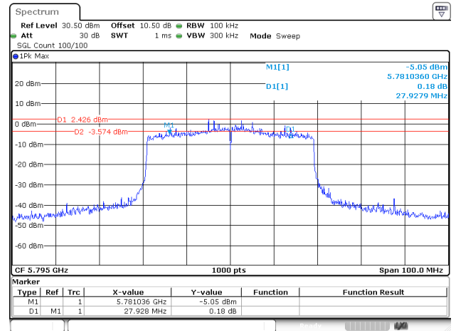
802.11ax40_5795MHz_RU_Full_ANT2
