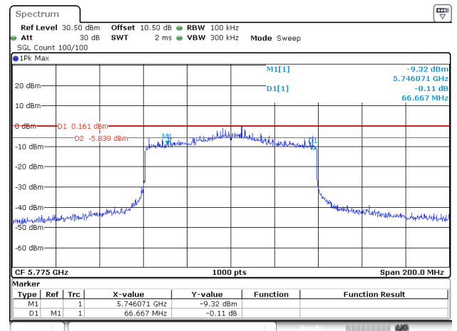
802.11ax80_5775MHz_RU_Full_ANT2
