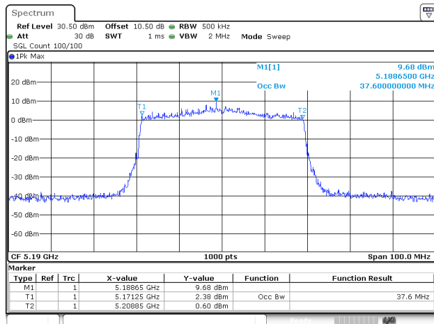
802.11ax40_5190MHz_RU_Full_ANT2
