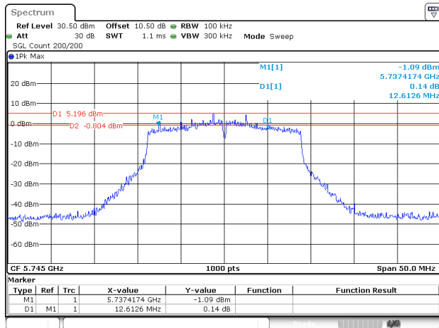
802.11ac20_5745MHz_ANT1
