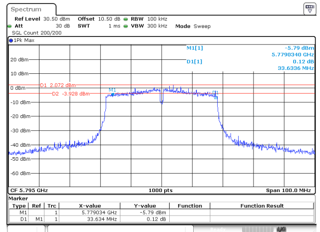
802.11ac40_5795MHz_ANT2
