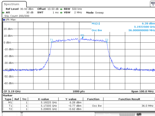
802.11ac40_5190MHz_ANT2
