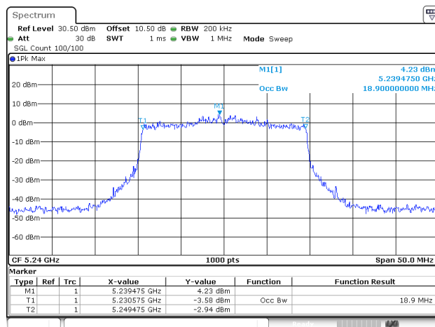
802.11ax20_5240MHz_RU_Full_ANT2
