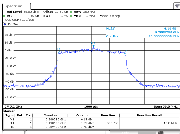
802.11ax20_5200MHz_RU_Full_ANT2
