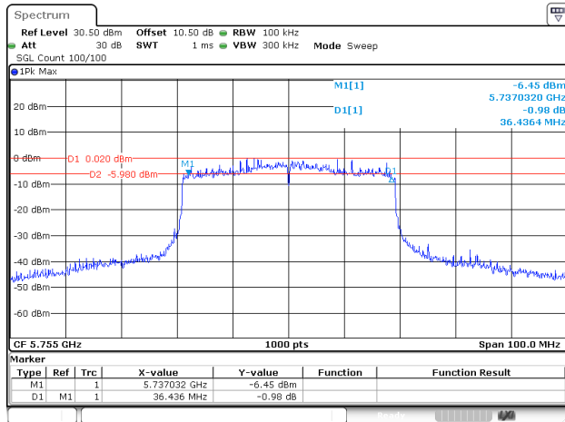
802.11ax40_5755MHz_RU_Full_ANT2
