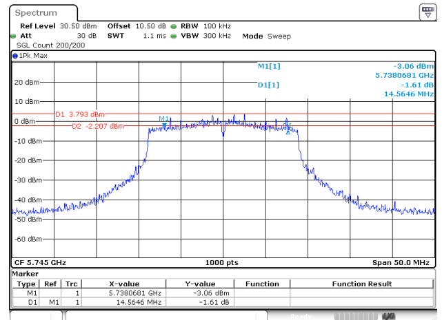
802.11ac20_5745MHz_ANT2
