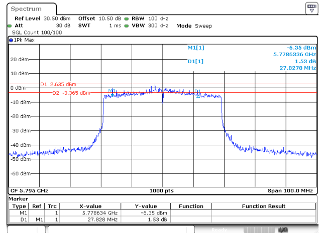
802.11ax40_5795MHz_RU_Full_ANT1
