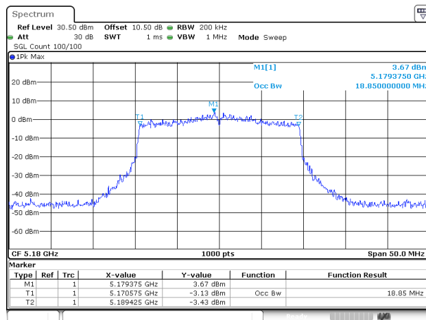
802.11ax20_5180MHz_RU_Full_ANT2
