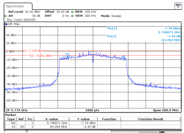
802.11ac80_5775MHz_ANT2
