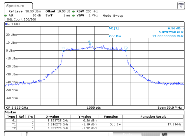
802.11ac20_5825MHz_ANT2
