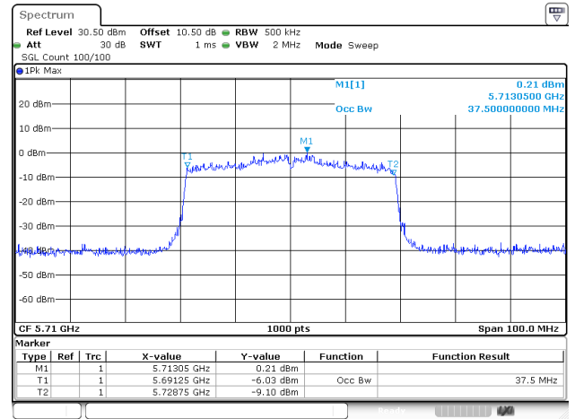
802.11ax40_5710MHz_RU_Full_ANT2
