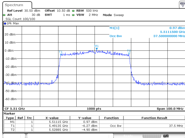
802.11ax40_5510MHz_RU_Full_ANT1
