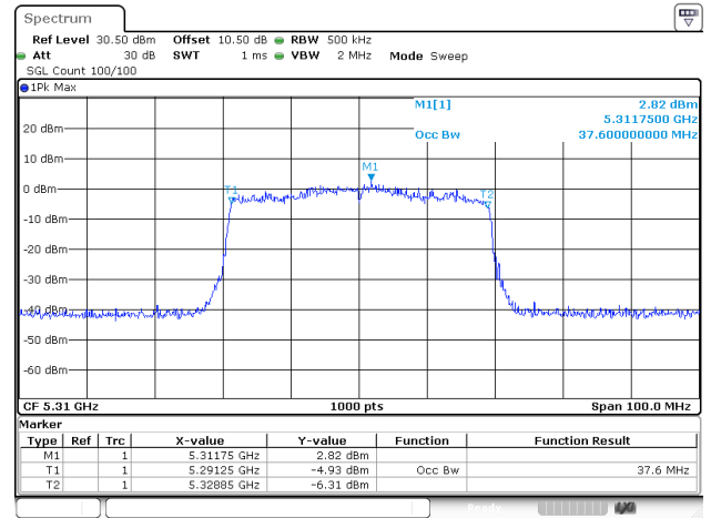
802.11ax40_5310MHz_RU_Full_ANT1
