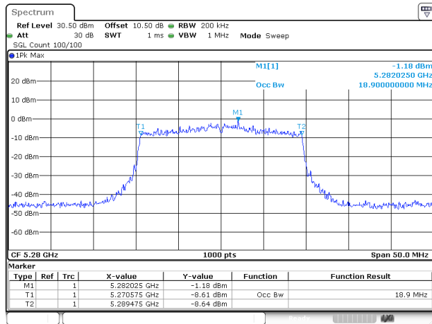
802.11ax20_5280MHz_RU_Full_ANT2
