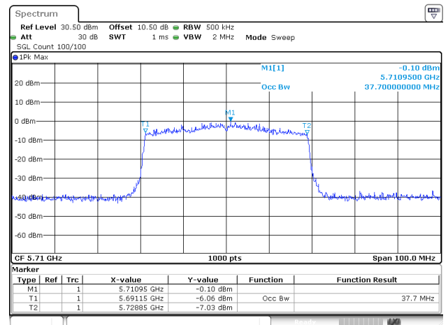
802.11ax40_5710MHz_RU_Full_ANT1
