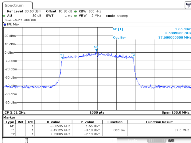
802.11ax40_5510MHz_RU_Full_ANT2
