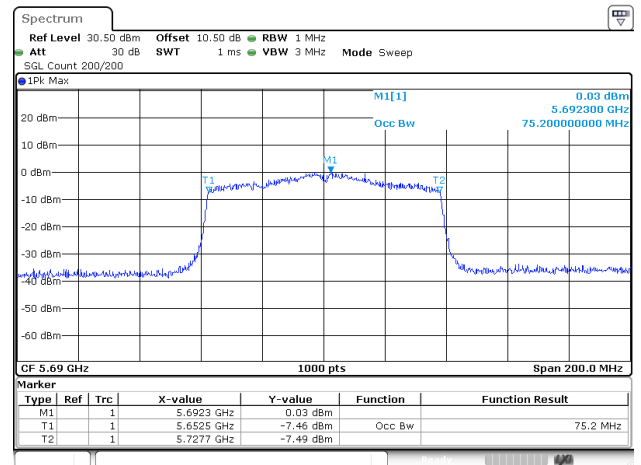
802.11ac80_5690MHz_ANT2
