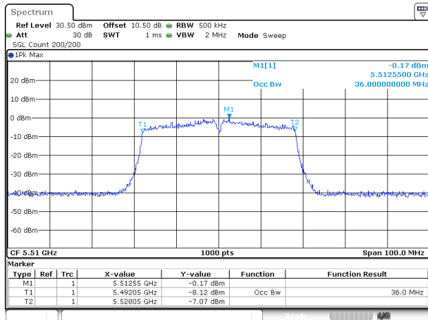
802.11ac40_5510MHz_ANT2
