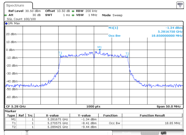
802.11ax20_5280MHz_RU_Full_ANT1
