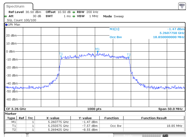
802.11ax20_5260MHz_RU_Full_ANT2
