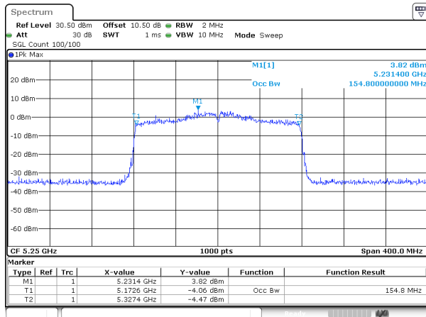
802.11ax160_5250MHz_RU_Full_ANT1
