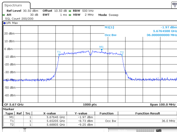
802.11ac40_5670MHz_ANT2
