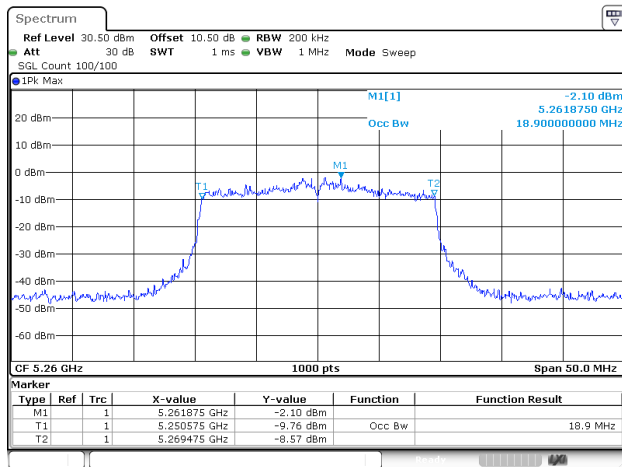
802.11ax20_5260MHz_RU_Full_ANT1
