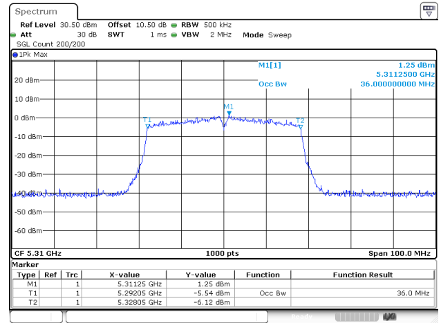
802.11ac40_5310MHz_ANT2
