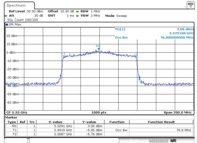
802.11ax80_5530MHz_RU_Full_ANT2
