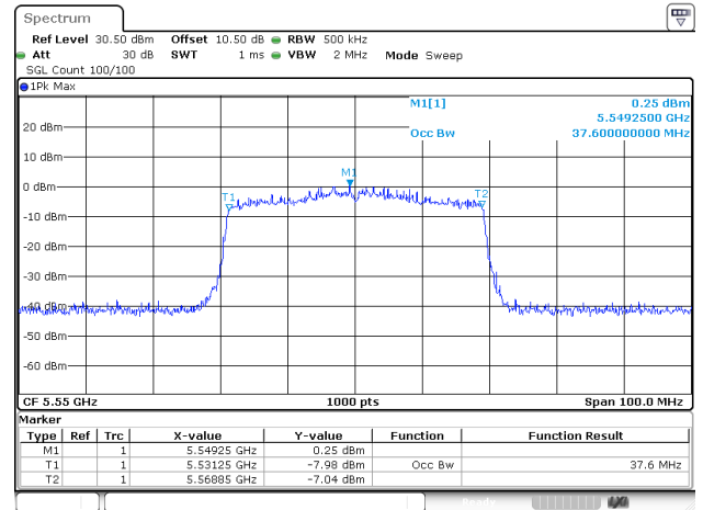
802.11ax40_5550MHz_RU_Full_ANT1
