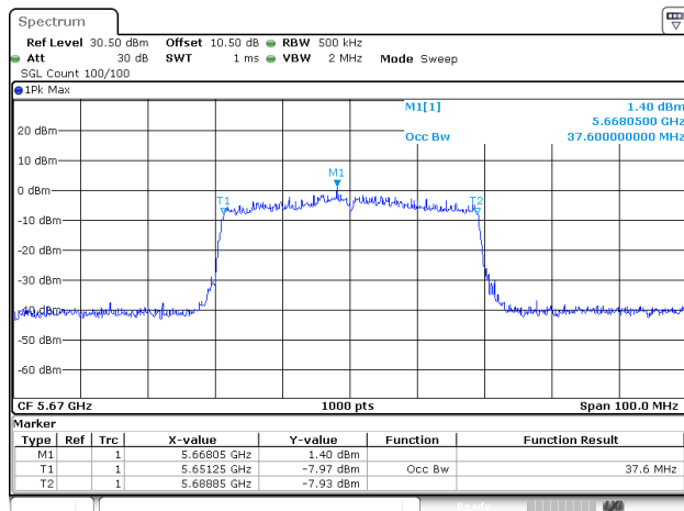
802.11ax40_5670MHz_RU_Full_ANT1
