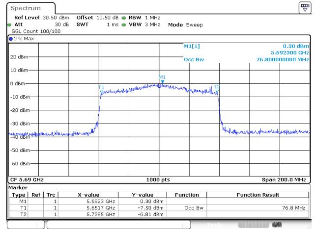
802.11ax80_5690MHz_RU_Full_ANT2
