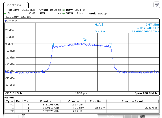
802.11ax40_5310MHz_RU_Full_ANT2
