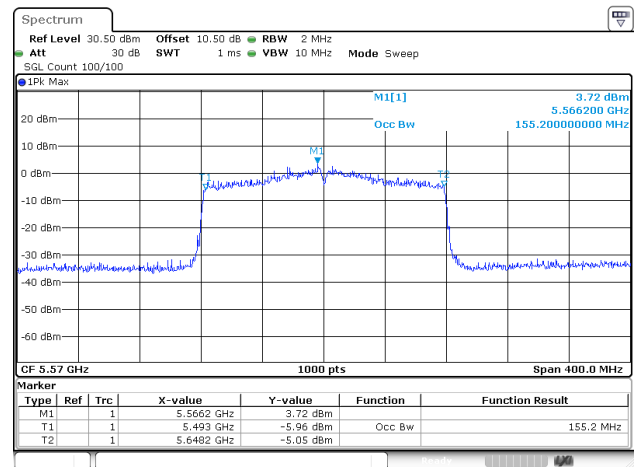
802.11ax160_5570MHz_RU_Full_ANT2
