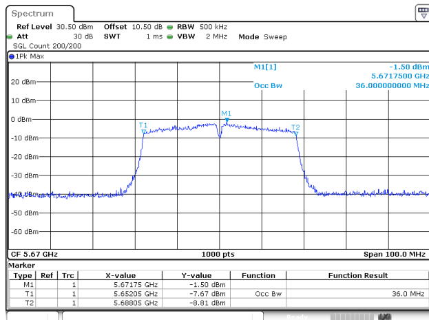
802.11ac40_5670MHz_ANT1
