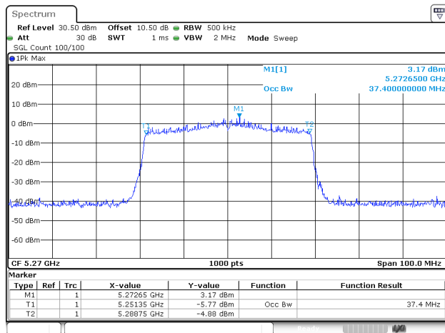
802.11ax40_5270MHz_RU_Full_ANT2
