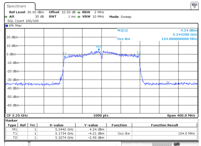
802.11ac160_5250MHz_ANT2
