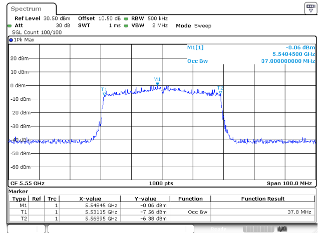
802.11ax40_5550MHz_RU_Full_ANT2
