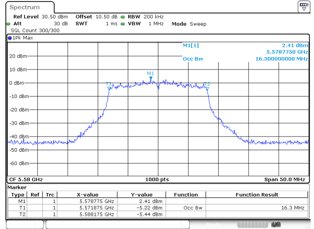
802.11a_5580MHz_ANT2
