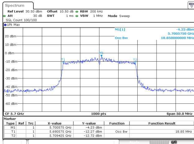
802.11ax20_5700MHz_RU_Full_ANT2
