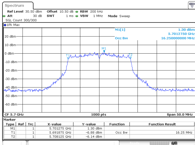
802.11a_5700MHz_ANT2
