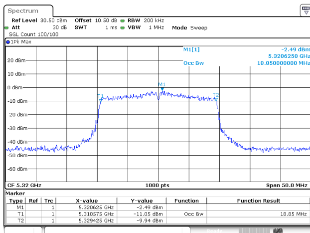
802.11ax20_5320MHz_RU_Full_ANT1
