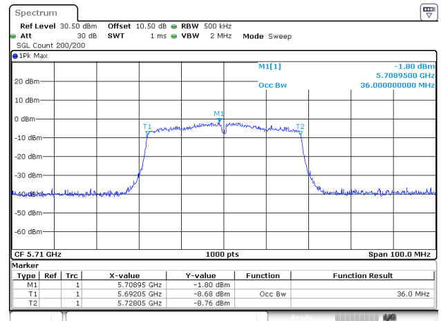
802.11ac40_5710MHz_ANT2
