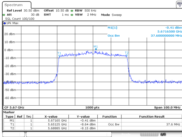
802.11ax40_5670MHz_RU_Full_ANT2
