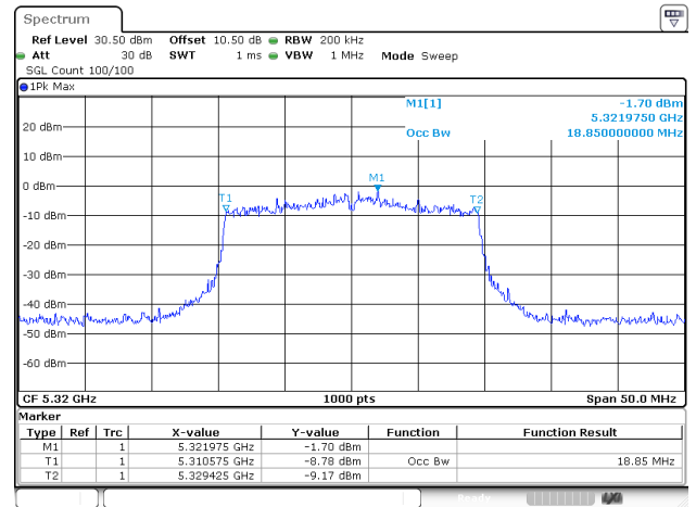
802.11ax20_5320MHz_RU_Full_ANT2
