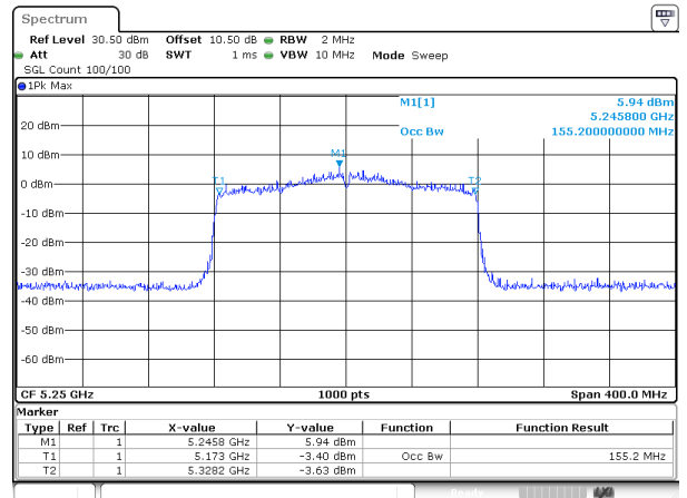
802.11ax160_5250MHz_RU_Full_ANT2
