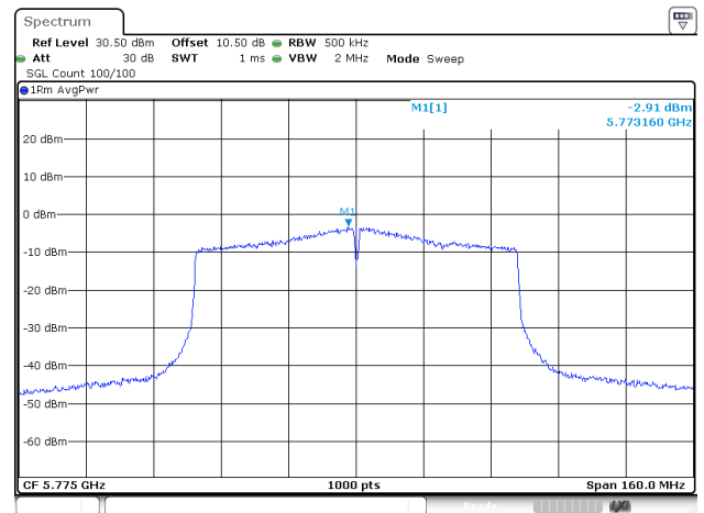
802.11ac80_5775MHz_ANT2
