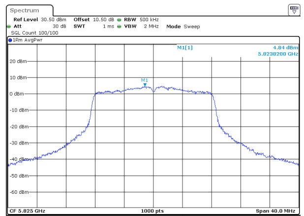
802.11a_5825MHz_ANT2
