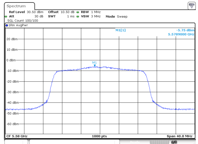
802.11ax20_5580MHz_RU_Full_ANT2
