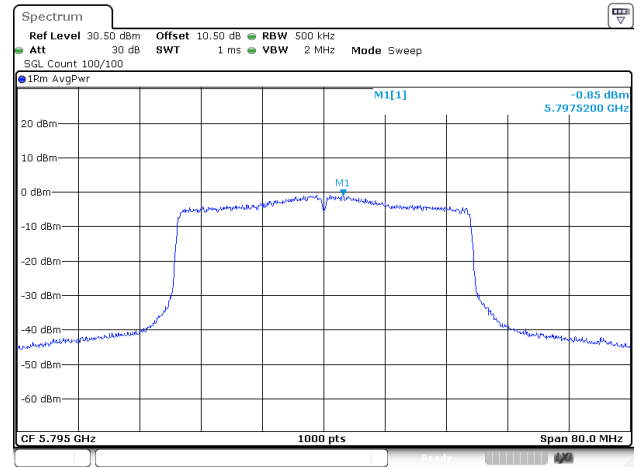
802.11ax40_5795MHz_RU_Full_ANT2
