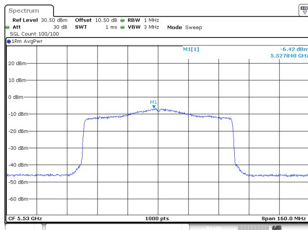
802.11ax80_5530MHz_RU_Full_ANT2
