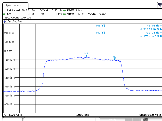
802.11ax40_5710MHz_RU_Full_ANT2
