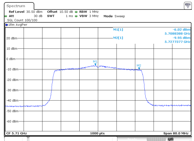
802.11ax40_5710MHz_RU_Full_ANT1
