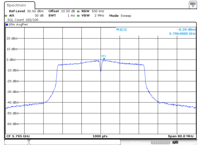
802.11ac40_5795MHz_ANT2
