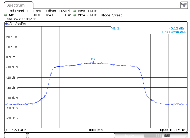
802.11ax20_5580MHz_RU_Full_ANT1
