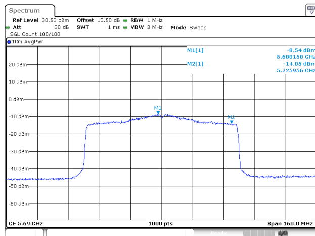
802.11ax80_5690MHz_RU_Full_ANT2
