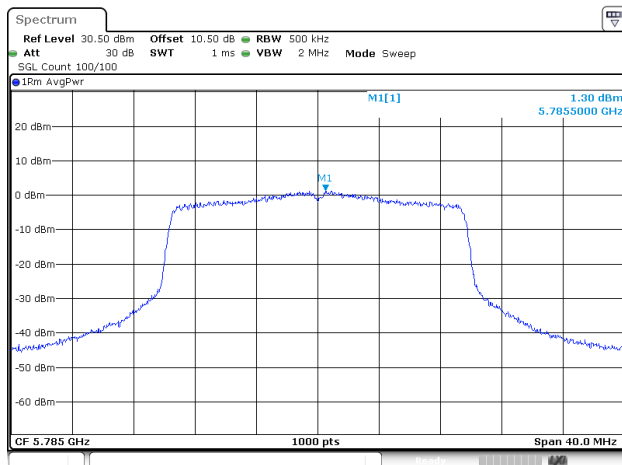
802.11ax20_5785MHz_RU_Full_ANT2
