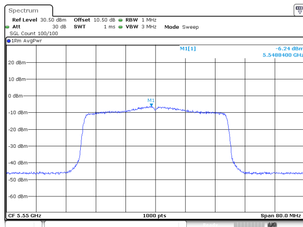
802.11ax40_5550MHz_RU_Full_ANT2
