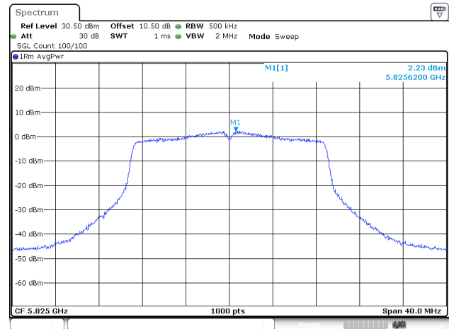
802.11ac20_5825MHz_ANT2
