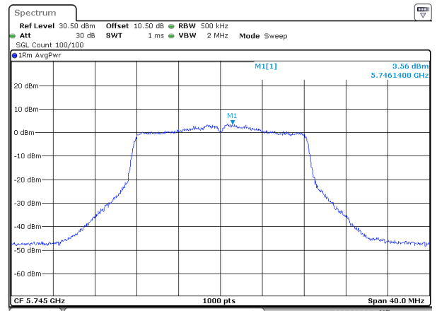
802.11a_5745MHz_ANT2
