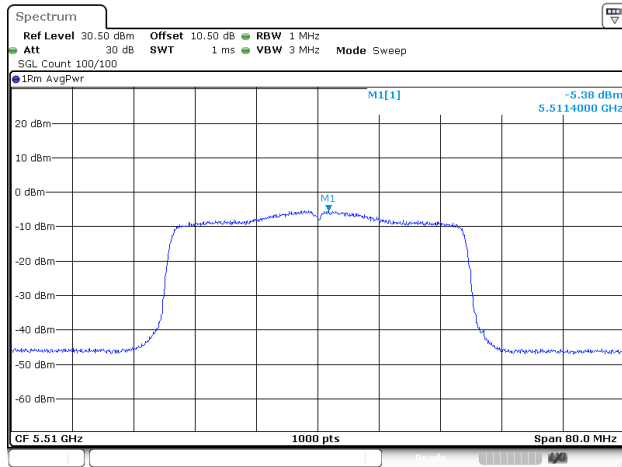
802.11ax40_5510MHz_RU_Full_ANT1
