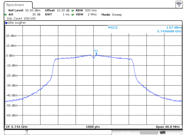
802.11ac20_5745MHz_ANT2
