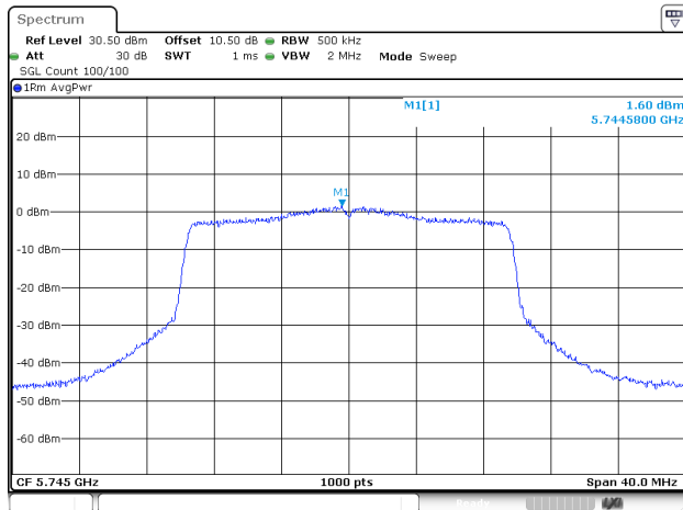
802.11ax20_5745MHz_RU_Full_ANT1
