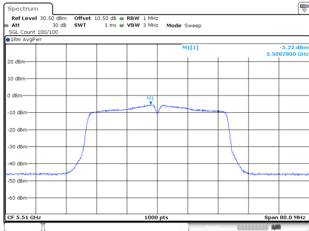
802.11ac40_5510MHz_ANT2
