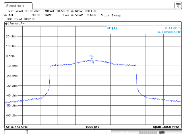
802.11ax80_5775MHz_RU_Full_ANT2
