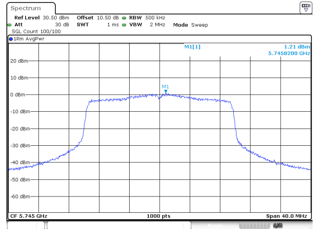
802.11ax20_5745MHz_RU_Full_ANT2
