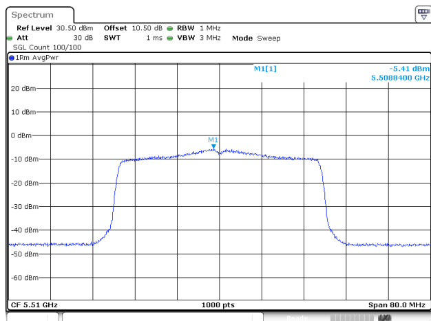
802.11ax40_5510MHz_RU_Full_ANT2
