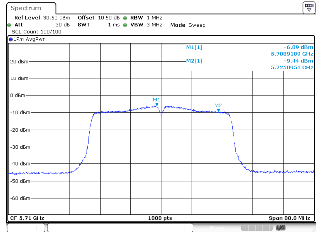
802.11ac40_5710MHz_ANT2
