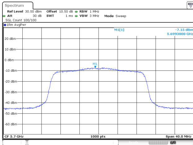
802.11ax20_5700MHz_RU_Full_ANT2
