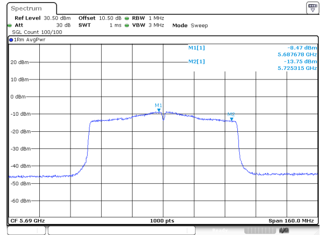
802.11ac80_5690MHz_ANT2
