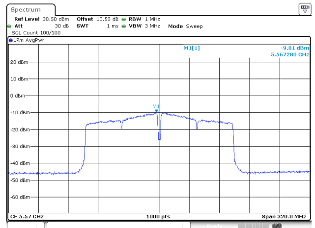
802.11ac160_5570MHz_ANT2
