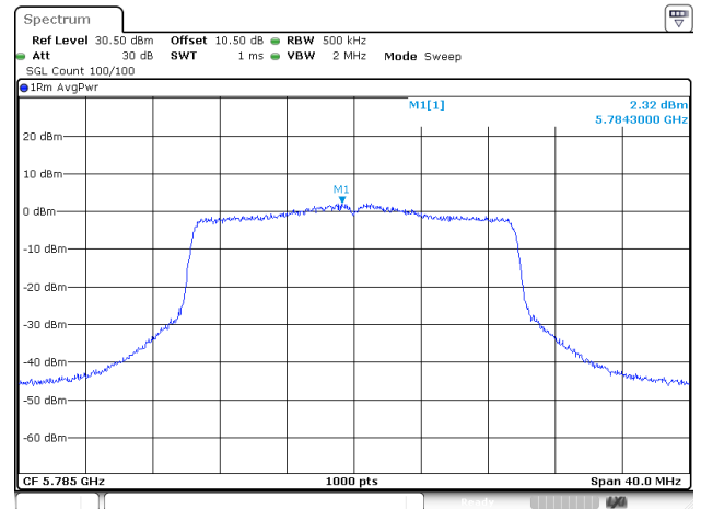
802.11ax20_5785MHz_RU_Full_ANT1
