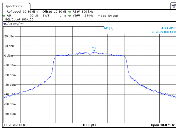
802.11a_5785MHz_ANT2
