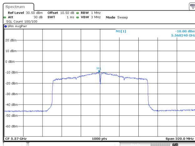
802.11ax160_5570MHz_RU_Full_ANT2
