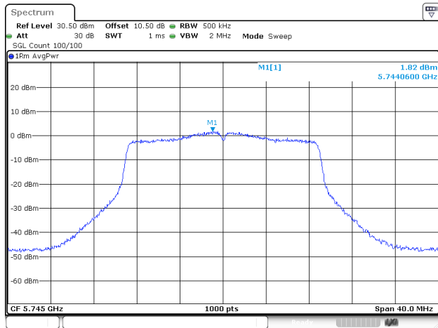
802.11ac20_5745MHz_ANT1
