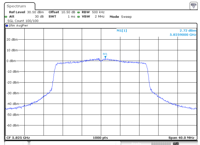
802.11ax20_5825MHz_RU_Full_ANT2
