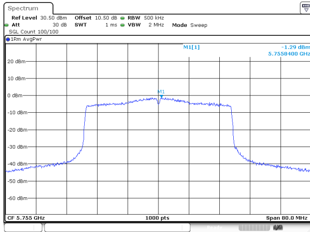
802.11ax40_5755MHz_RU_Full_ANT2
