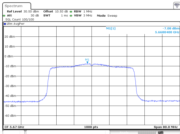
802.11ax40_5670MHz_RU_Full_ANT2
