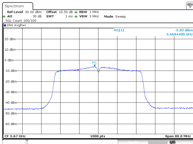
802.11ac40_5670MHz_ANT1
