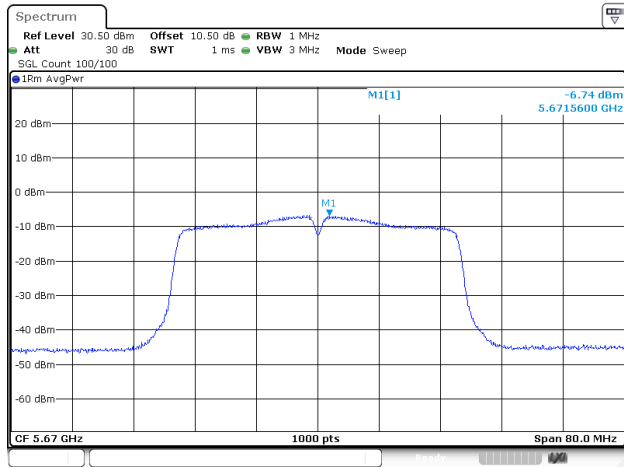
802.11ac40_5670MHz_ANT2
