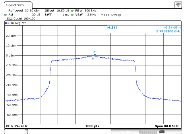
802.11ax40_5795MHz_RU_Full_ANT1
