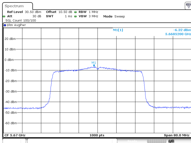
802.11ax40_5670MHz_RU_Full_ANT1
