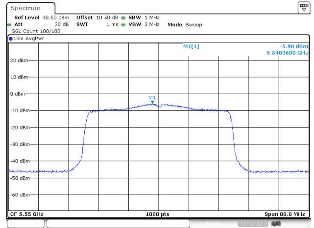
802.11ax40_5550MHz_RU_Full_ANT1
