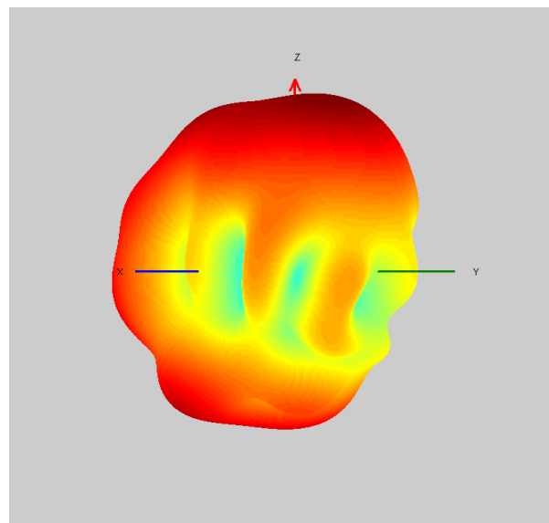
2.4G 3D
