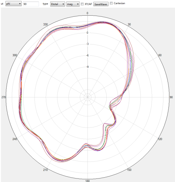
2.4G phi=90deg
