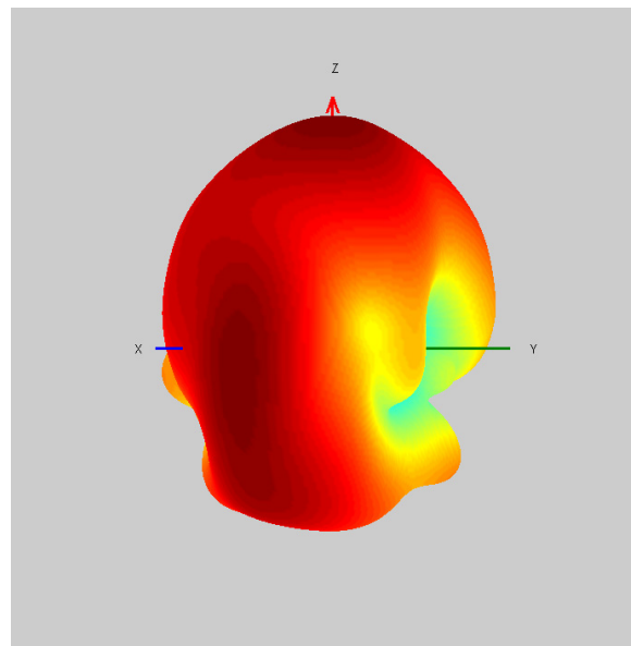
2.4G 3D
