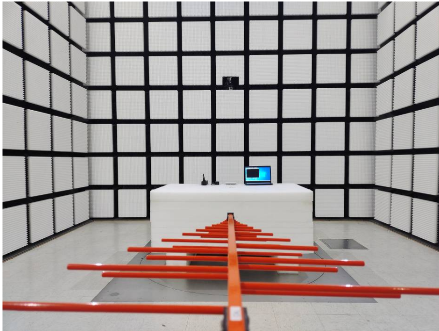
Radiated Emissions Below 1G rear View for M2
