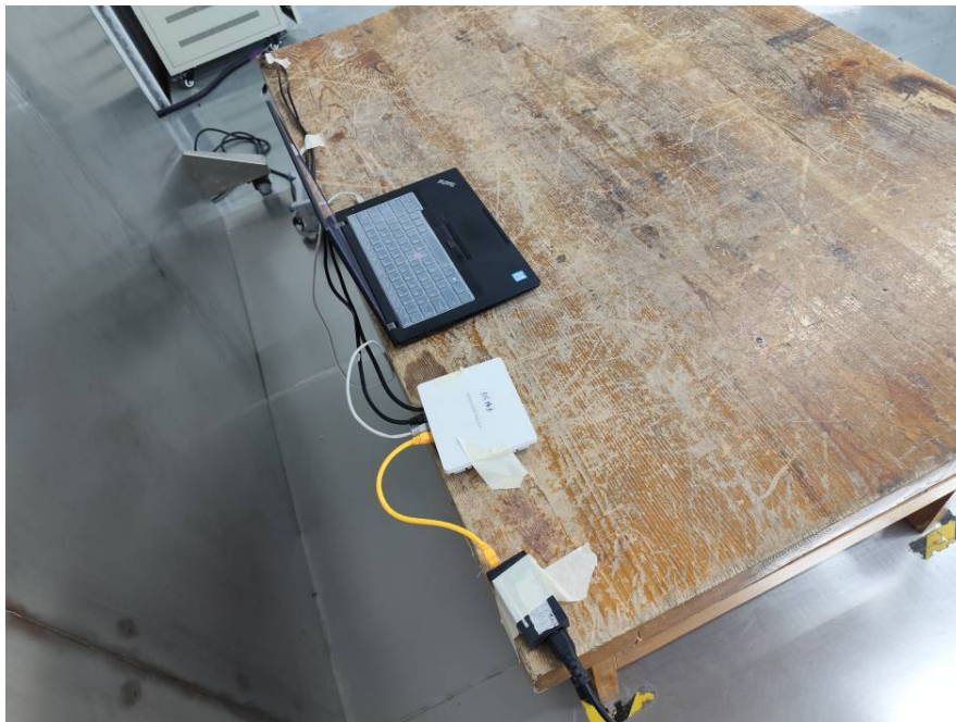
Conducted emissions side View for M2
