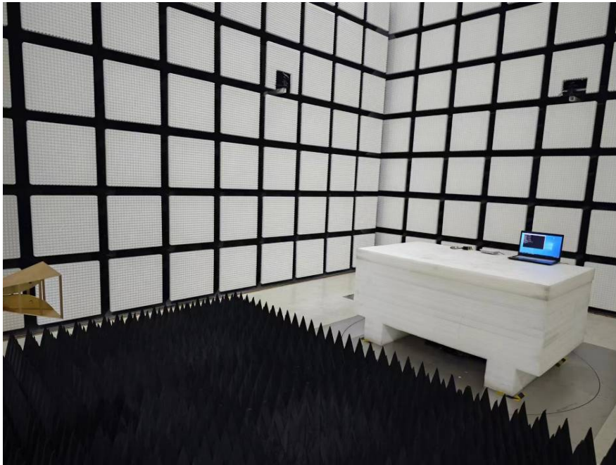
Radiated Emissions Above 1G rear View for M2
