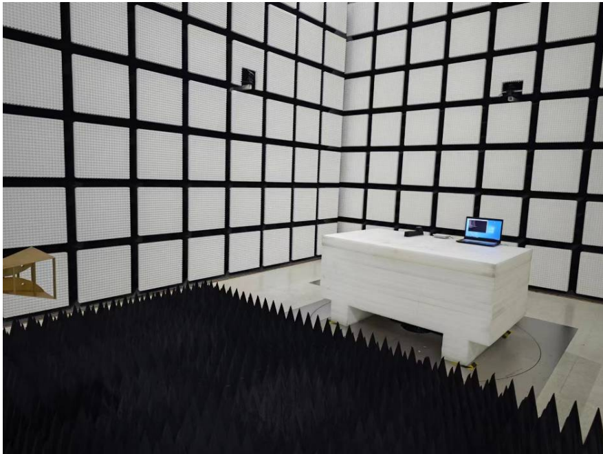
Radiated Emissions Above 1G rear View for M1
