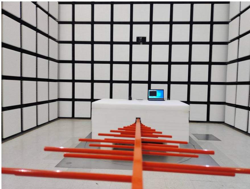
Radiated Emissions Below 1G rear View for M1
