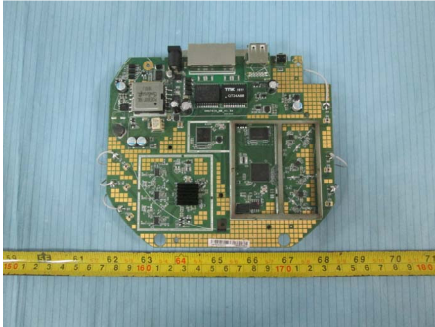
EUT –Main board shield-off Top View
