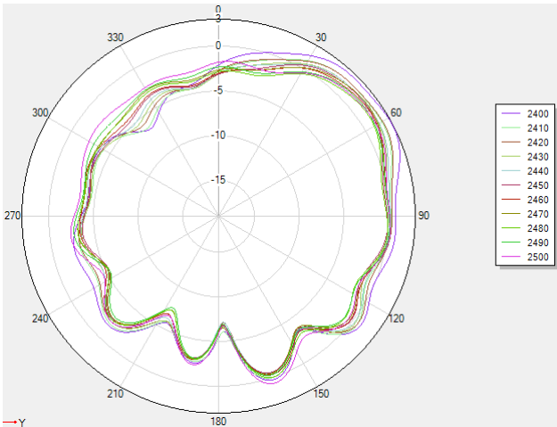
2.4G phi=90deg
