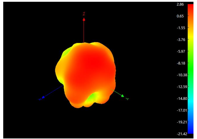
2.4G 3D
