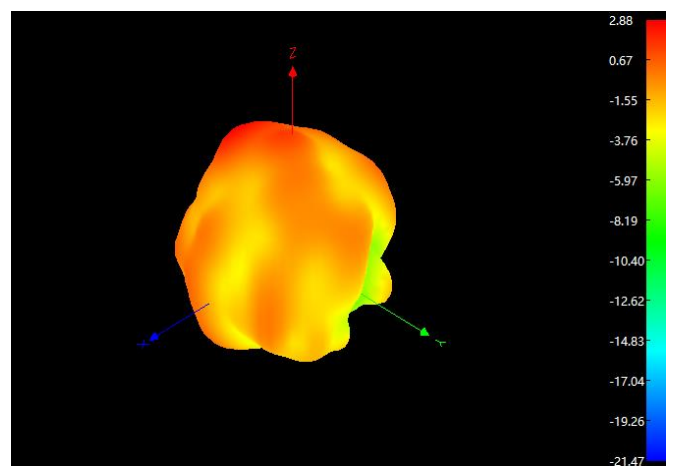
5.15G 3D
