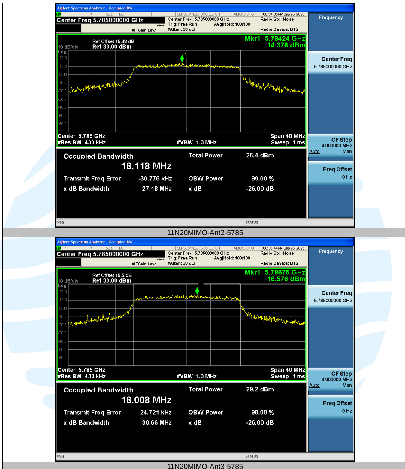
11N20MIMO-Ant3-5785
