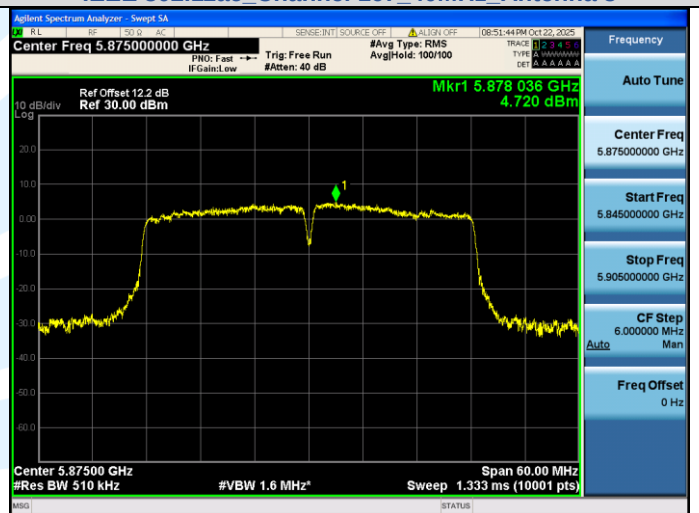
IEEE 802.11ac Channel 175 40MHz Antenna 3
