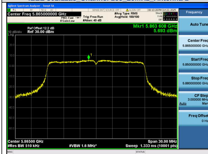
IEEE 802.11ac Channel 173 20MHz Antenna 1
