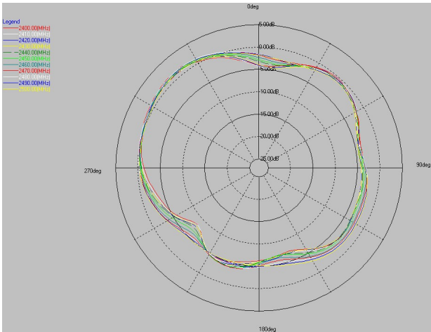
2.4G phi=90deg
