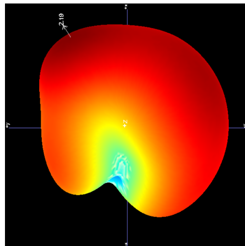
2.4G 3D
