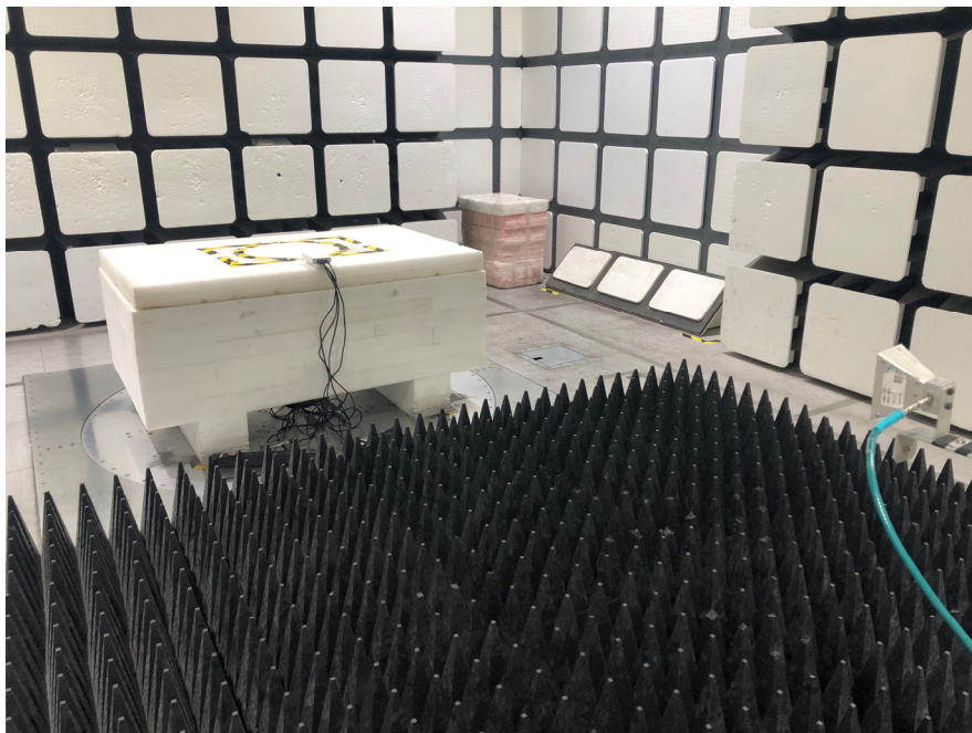
Radiated Emissions Rear View (18-30 GHz)
