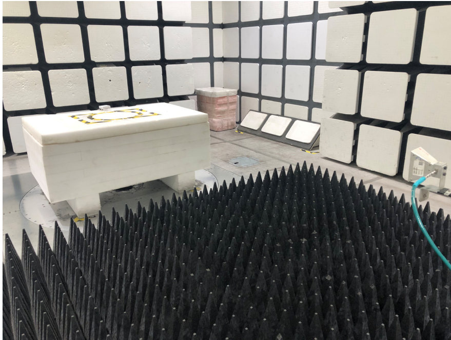
Radiated Emissions FrontView (18-30 GHz)
