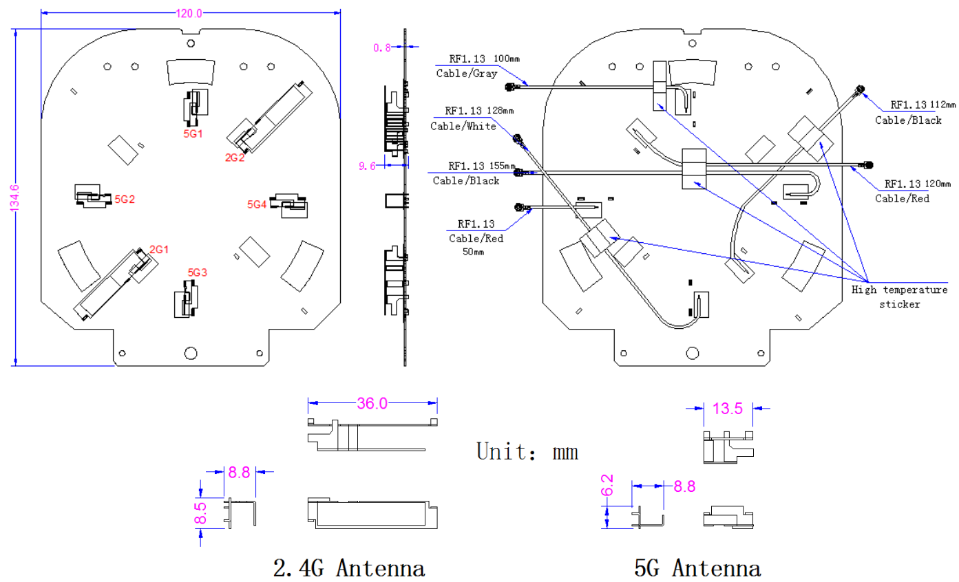
总成图 Mechanical Drawing(unit:mm)
