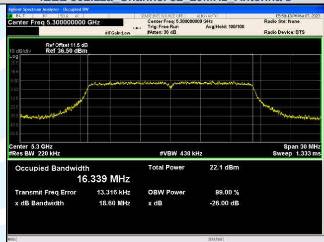
IEEE 802.11a_Channel 60_20MHz_Antenna 1
