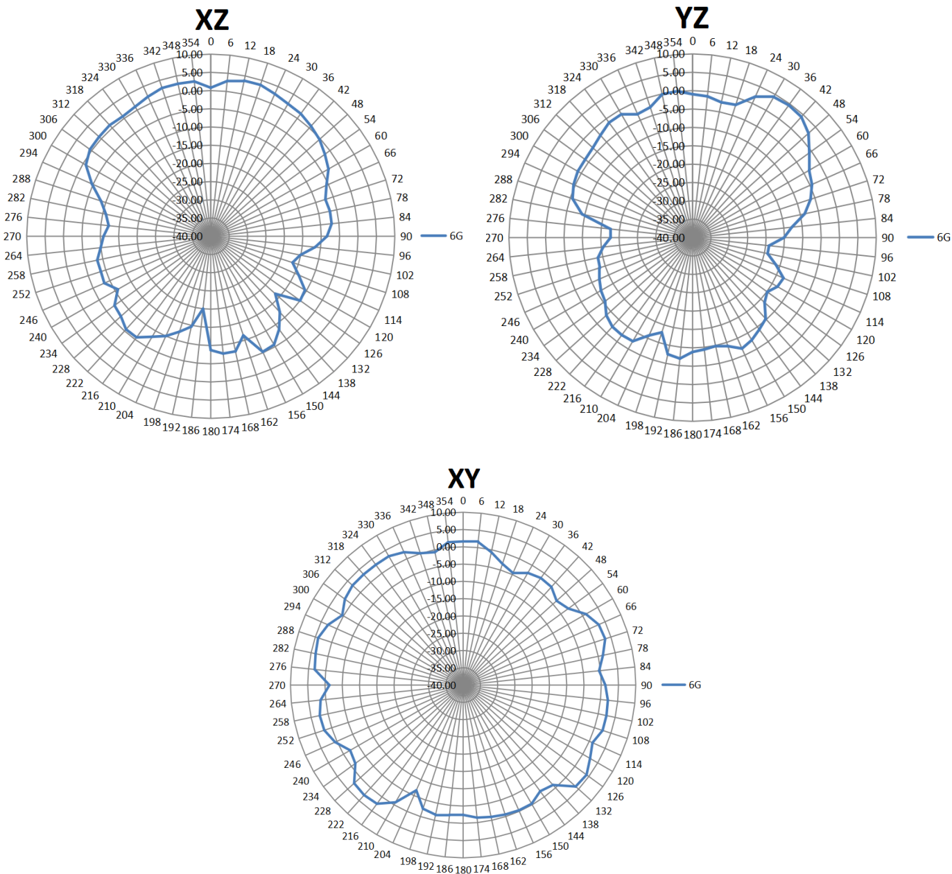
6G 辐射方向图 Radiation Patterns(unit:dB)
