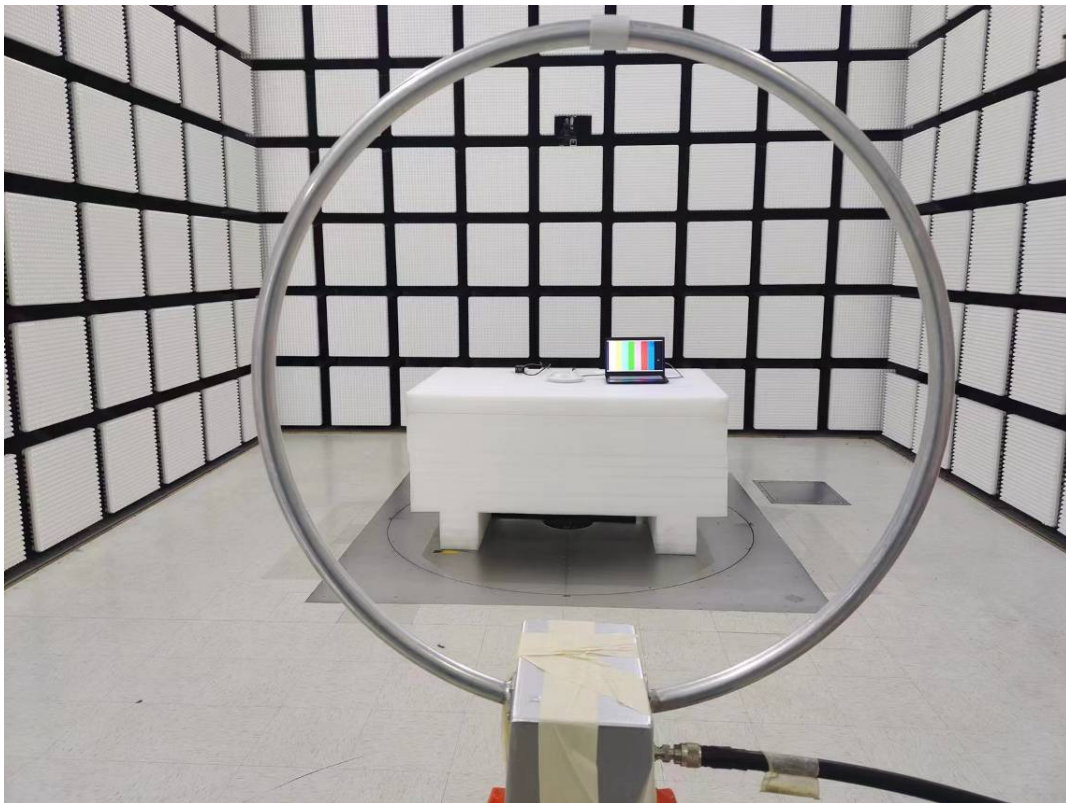
Radiated Emission Below 30MHz View Parallel
