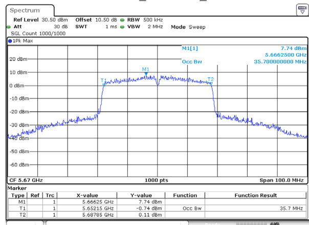
802.11ac40_5670MHz_Ant 1
