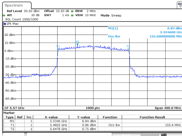
802.11ax160_5570MHz_RU_FULL_Ant 2
