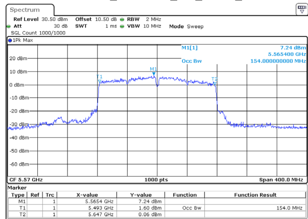
802.11ac160_5570MHz_RU_FULL_Ant 1
