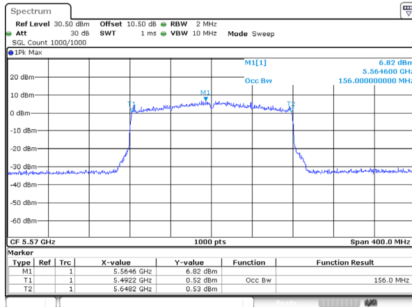
802.11ax160_5570MHz_RU_FULL_Ant 0
