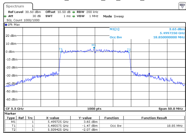
802.11ax20_5500MHz_RU_FULL_Ant 0
