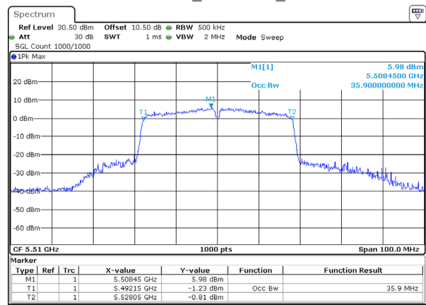
802.11ac40_5510MHz_Ant 0
