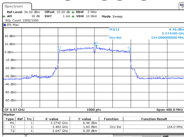
802.11ac160_5570MHz_RU_FULL_Ant 2
