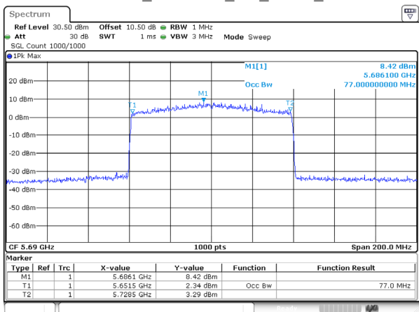
802.11ax80_5690MHz_RU_FULL_Ant 1
