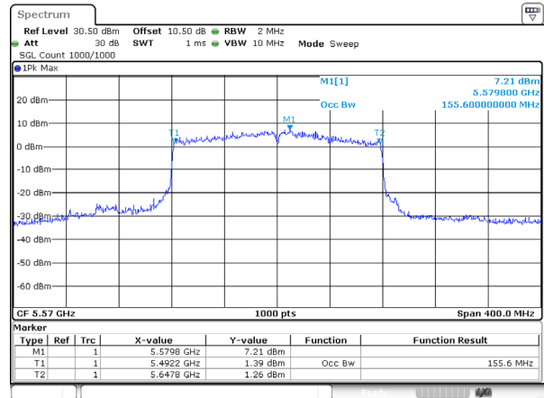
802.11ax160_5570MHz_RU_FULL_Ant 1
