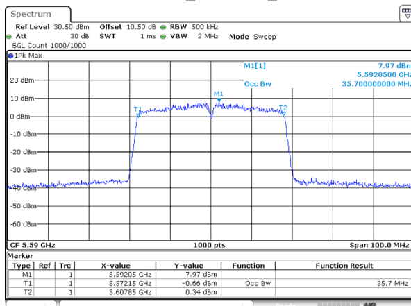
802.11ac40_5590MHz_Ant 1
