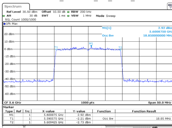
802.11ax20_5600MHz_RU_FULL_Ant 0
