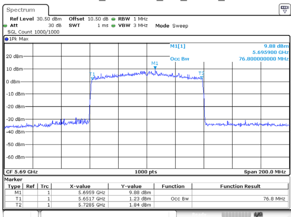
802.11ax80_5690MHz_RU_FULL_Ant 2
