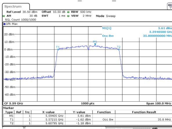
802.11ac40_5590MHz_Ant 0
