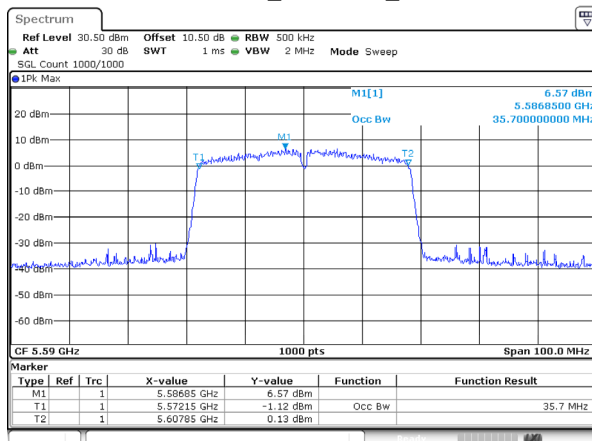
802.11ac40_5590MHz_Ant 2
