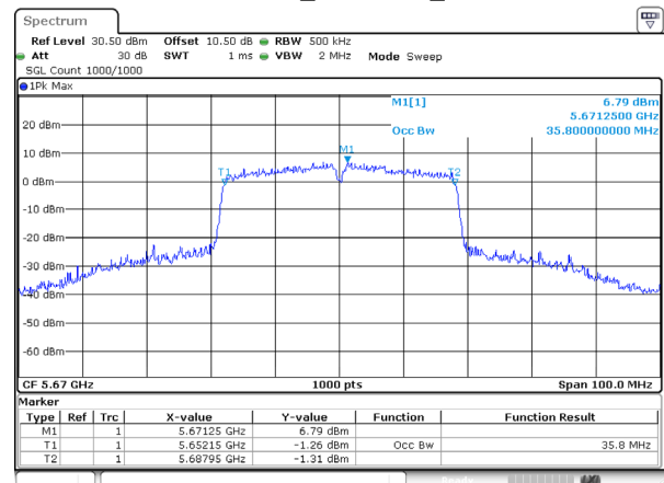
802.11ac40_5670MHz_Ant 2
