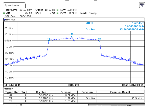
802.11ac40_5670MHz_Ant 0
