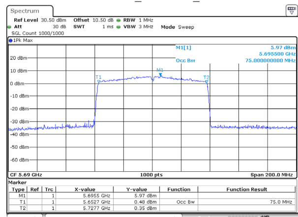
802.11ac80_5690MHz_Ant 0
