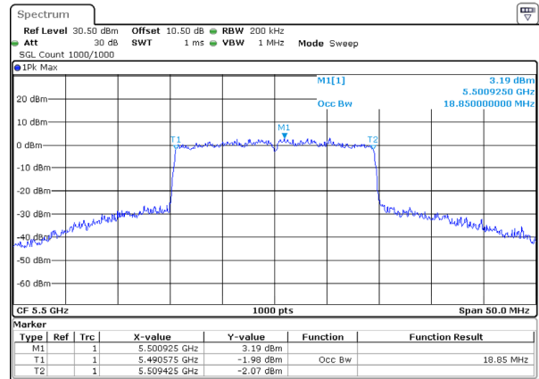
802.11ax20_5500MHz_RU_FULL_Ant 1
