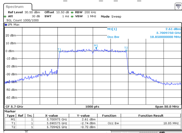
802.11ax20_5700MHz_RU_FULL_Ant 0
