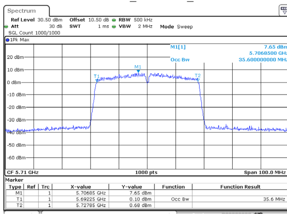
802.11ac40_5710MHz_Ant 1
