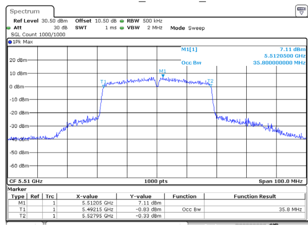
802.11ac40_5510MHz_Ant 2
