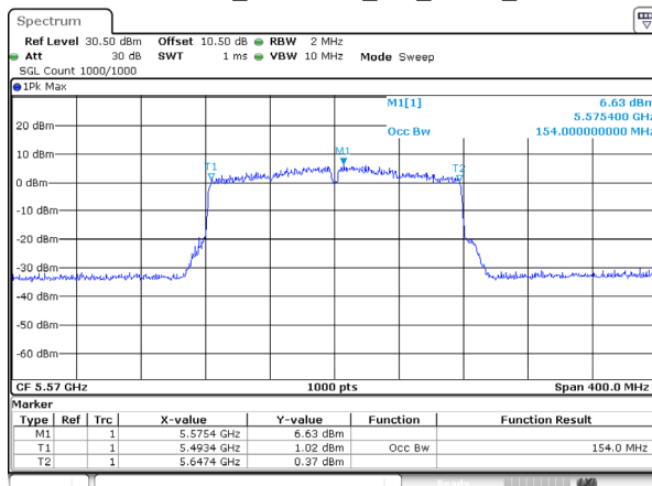
802.11ac160_5570MHz_RU_FULL_Ant 0
