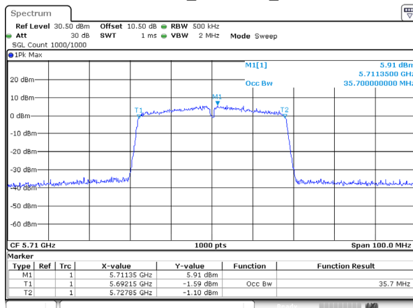
802.11ac40_5710MHz_Ant 0
