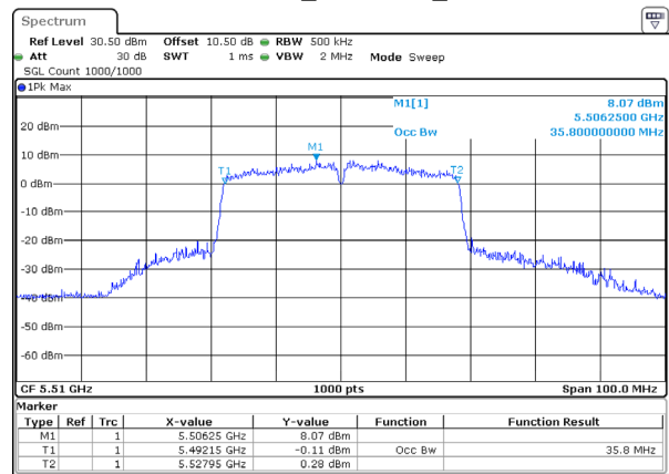
802.11ac40_5510MHz_Ant 1
