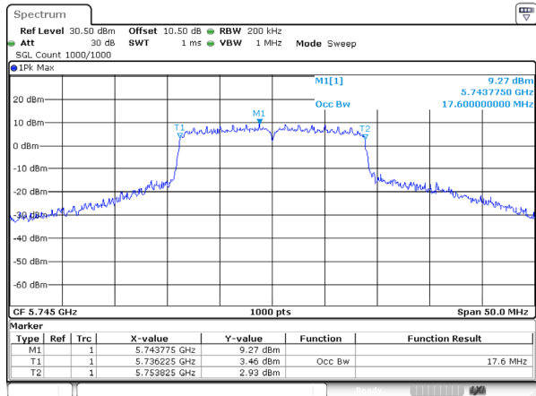
802.11ac20_5745MHz_Ant 2
