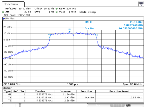
802.11a_5825MHz_Ant 1
