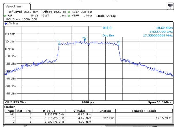
802.11ac20_5825MHz_Ant 1
