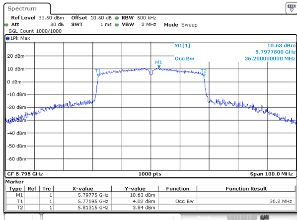
802.11ac40_5795MHz_Ant 0
