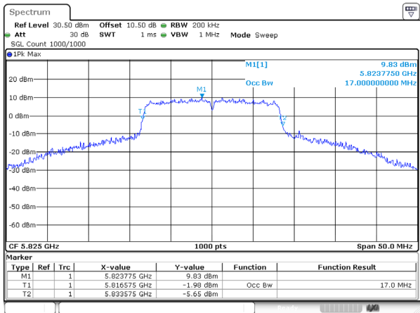
802.11a_5825MHz_Ant 2
