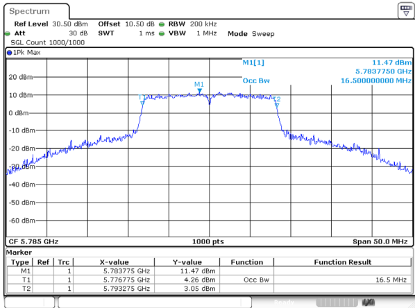
802.11a_5785MHz_Ant 1
