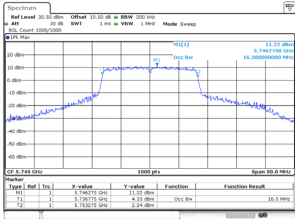
802.11a_5745MHz_Ant 1
