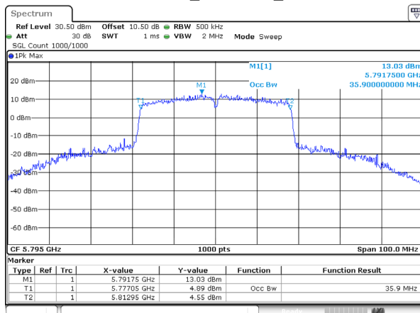
802.11ac40_5795MHz_Ant 1
