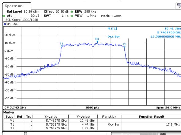
802.11ac20_5745MHz_Ant 0
