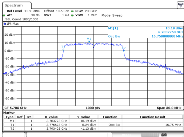
802.11a_5785MHz_Ant 2
