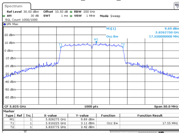
802.11ac20_5825MHz_Ant 0
