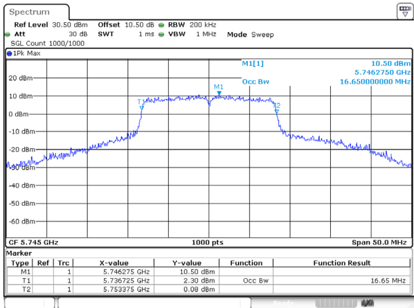
802.11a_5745MHz_Ant 2
