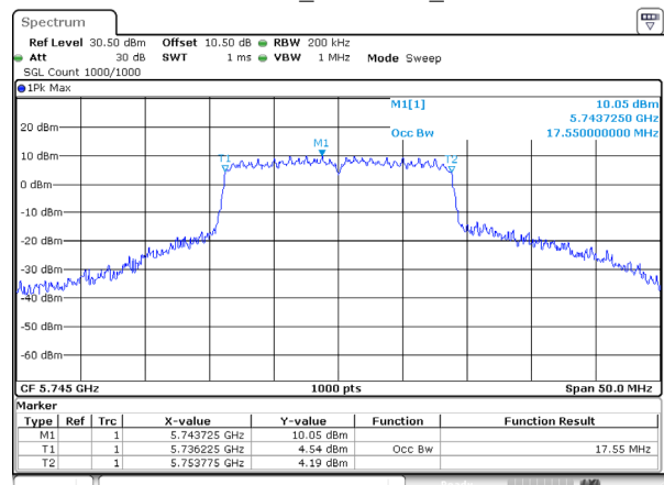
802.11ac20_5745MHz_Ant 1
