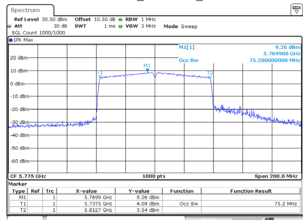
802.11ac80_5775MHz_Ant 0
