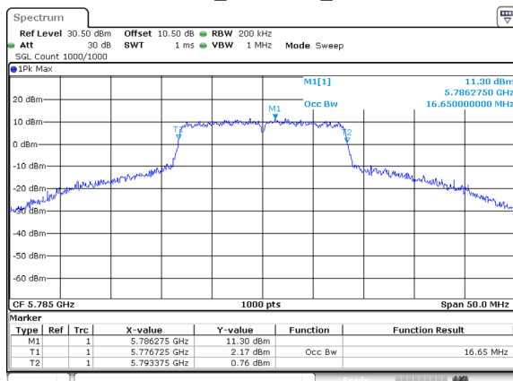
802.11a_5785MHz_Ant 0
