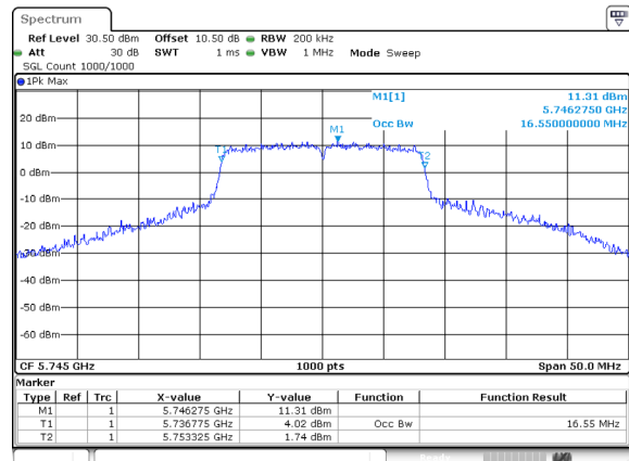
802.11a_5745MHz_Ant 0
