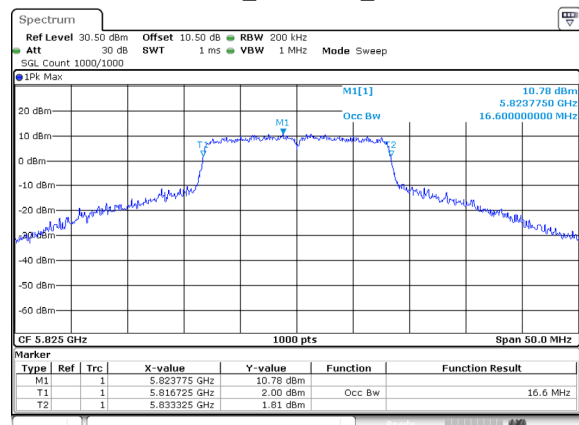
802.11a_5825MHz_Ant 0
