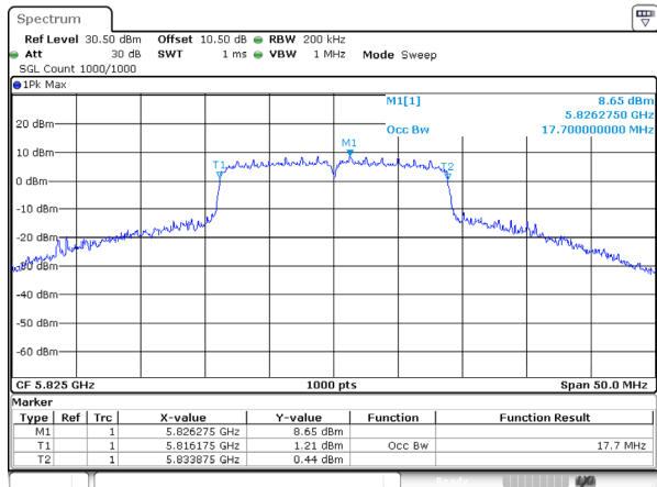
802.11ac20_5825MHz_Ant 2
