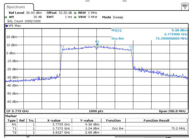
802.11ac80_5775MHz_Ant 2
