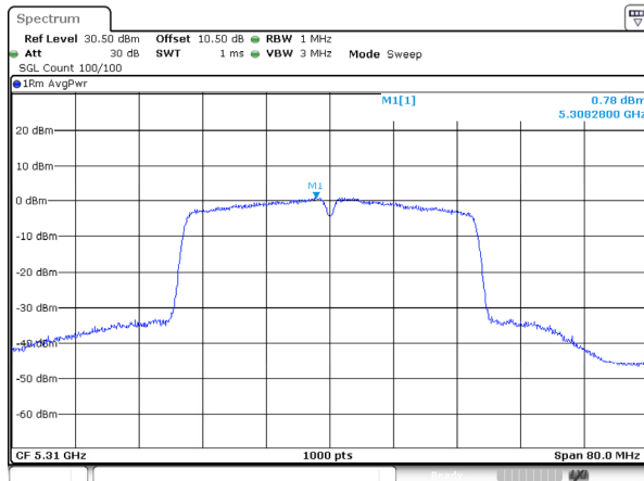
802.11ac40_5310MHz_Ant 0
