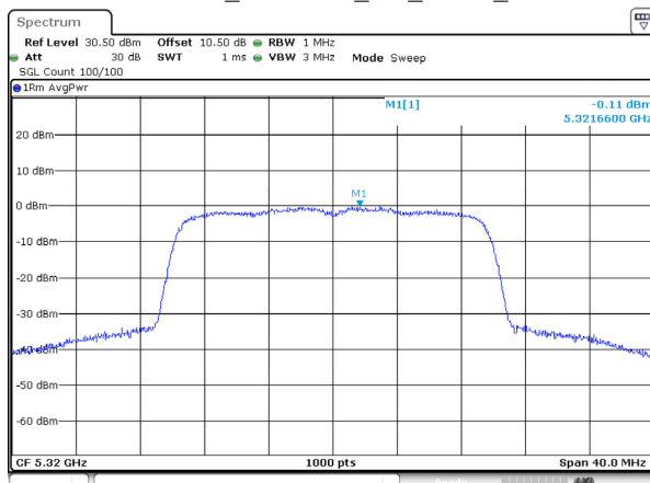
802.11ax20_5320MHz_RU_FULL_Ant 1
