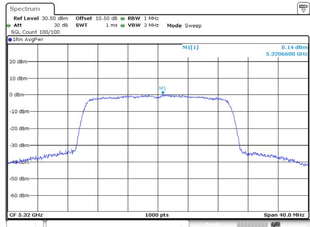
802.11ax20_5320MHz_RU_FULL_Ant 0
