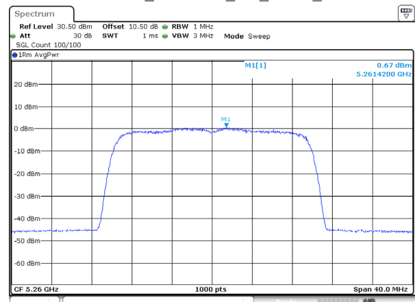
802.11ax20_5260MHz_RU_FULL_Ant 2
