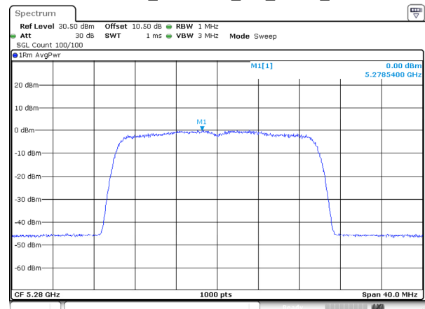
802.11ax20_5280MHz_RU_FULL_Ant 1
