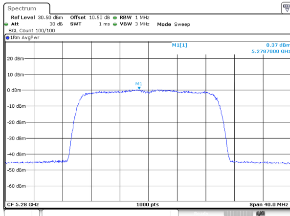
802.11ax20_5280MHz_RU_FULL_Ant 0
