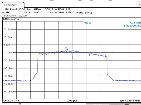
802.11ax160_5250MHz_RU_FULL_Ant 1
