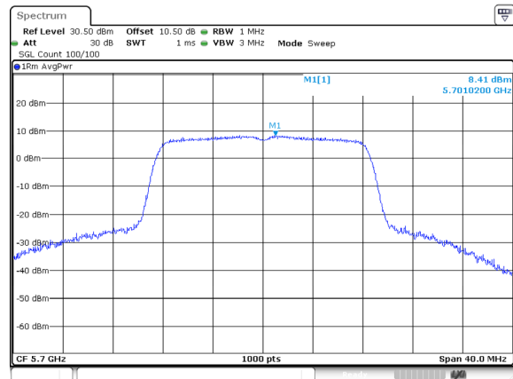
802.11a_5700MHz_Ant 0
