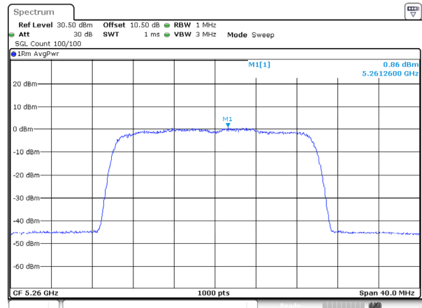
802.11ax20_5260MHz_RU_FULL_Ant 0
