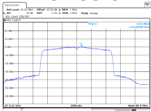
802.11ax40_5310MHz_RU_FULL_Ant 2
