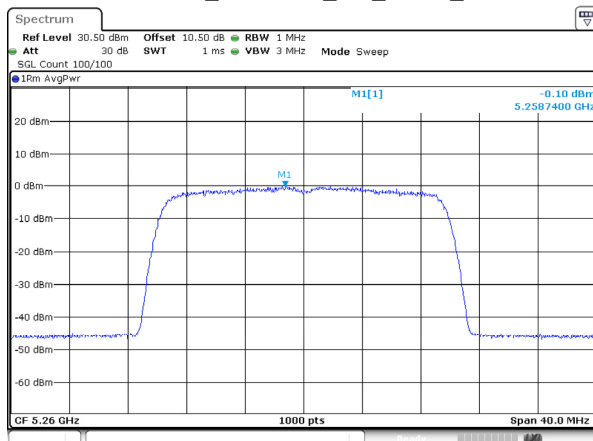
802.11ax20_5260MHz_RU_FULL_Ant 1
