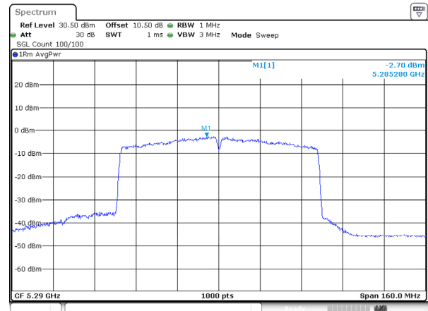
802.11ac80_5290MHz_Ant 0
