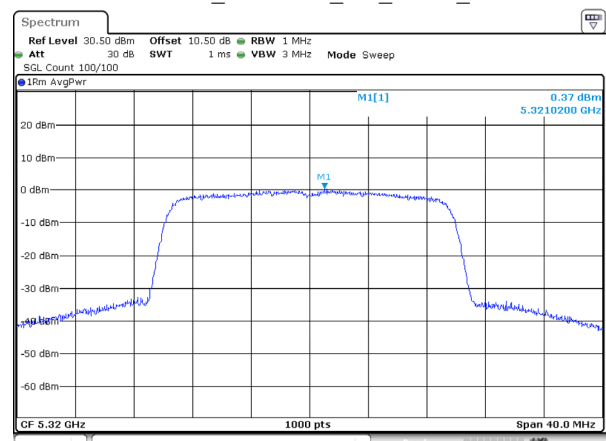
802.11ax20_5320MHz_RU_FULL_Ant 2
