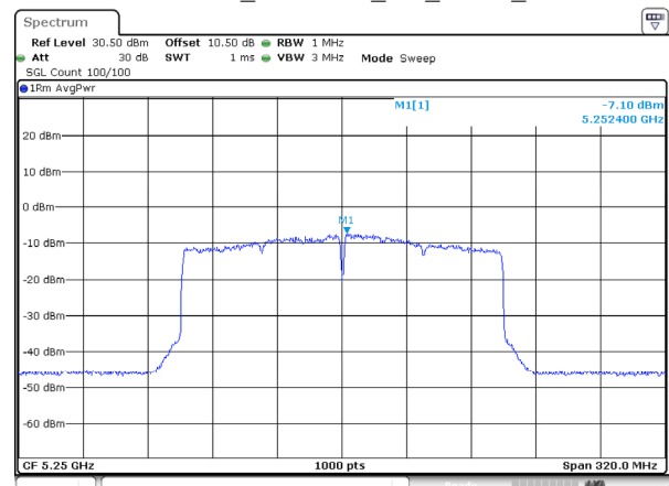
802.11ax160_5250MHz_RU_FULL_Ant 2
