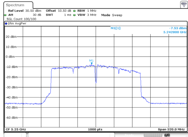
802.11ac160_5250MHz_RU_FULL_Ant 1
