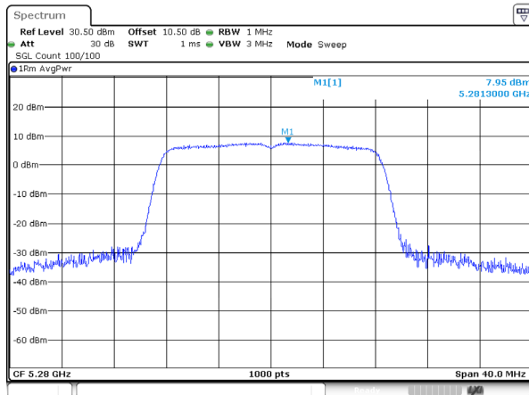
802.11a_5280MHz_Ant 2
