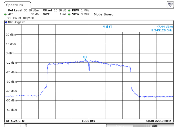
802.11ax160_5250MHz_RU_FULL_Ant 0
