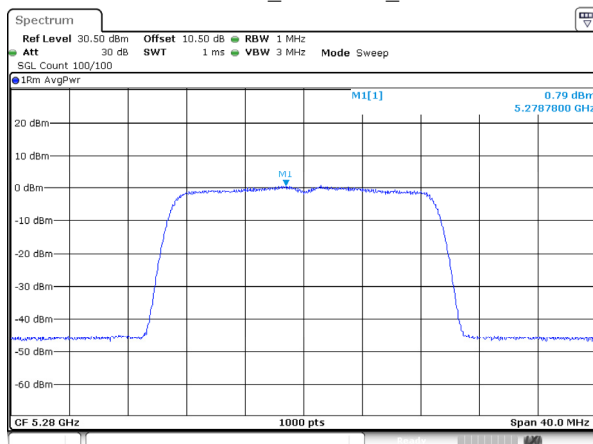
802.11ac20_5280MHz_Ant 1
