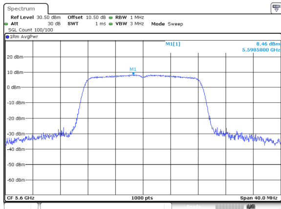
802.11a_5600MHz_Ant 0
