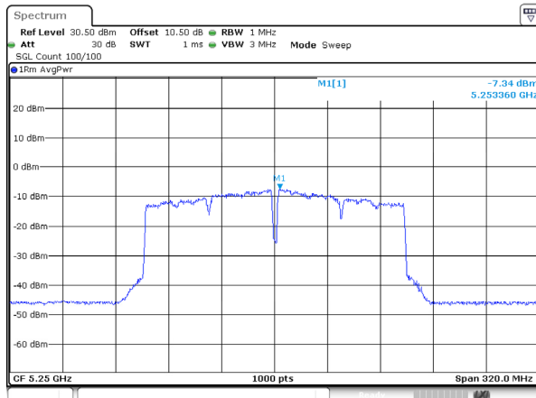
802.11ac160_5250MHz_RU_FULL_Ant 2
