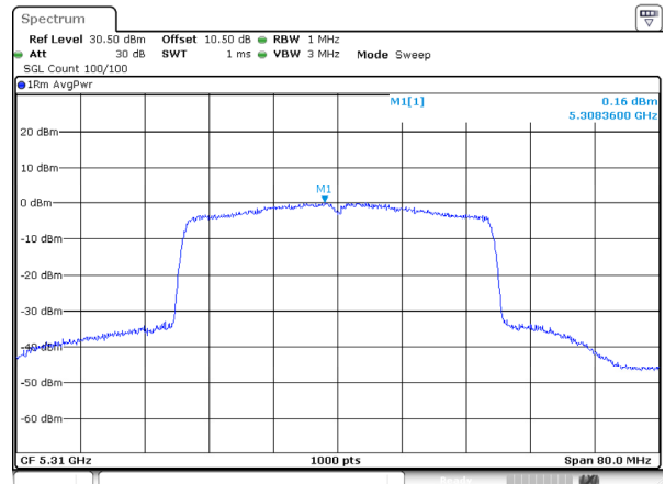
802.11ax40_5310MHz_RU_FULL_Ant 1
