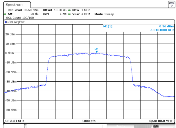
802.11ax40_5310MHz_RU_FULL_Ant 0
