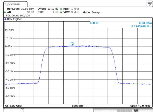
802.11ac20_5280MHz_Ant 0
