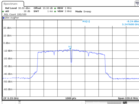
802.11ac160_5250MHz_RU_FULL_Ant 0
