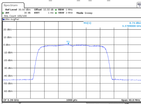
802.11ax20_5280MHz_RU_FULL_Ant 2
