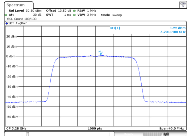
802.11ac20_5280MHz_Ant 2
