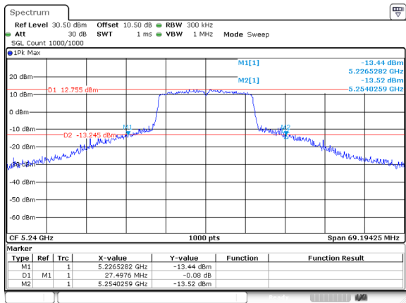
802.11a_5240MHz_Ant 0
