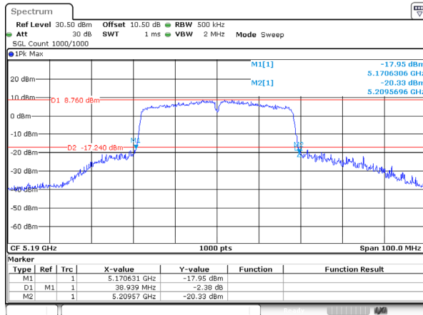
802.11ac40_5190MHz_Ant 0
