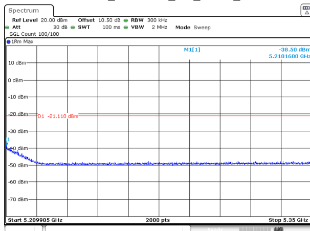
802.11ax20_5200MHz_RU_FULL_Ant 0
