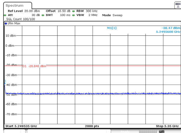
802.11ac20_5240MHz_Ant 2
