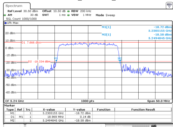
802.11ac20_5240MHz_Ant 0
