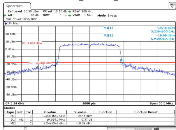
802.11ac20_5240MHz_Ant 2
