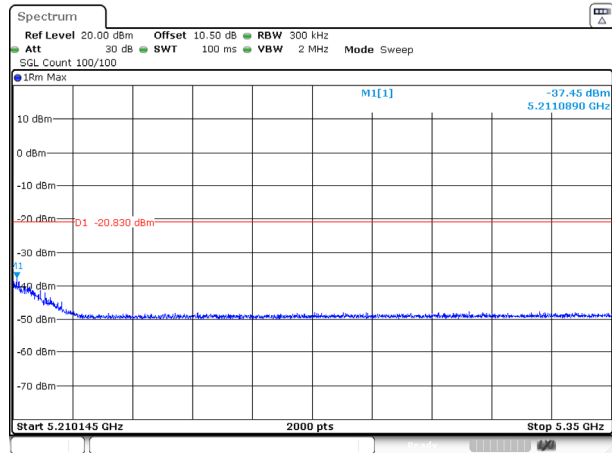
802.11ax20_5200MHz_RU_FULL_Ant 1
