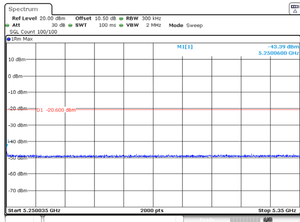
802.11ax20_5240MHz_RU_FULL_Ant 2
