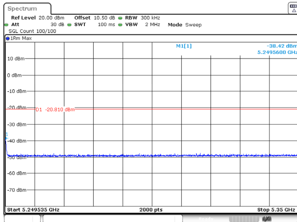
802.11ac20_5240MHz_Ant 1
