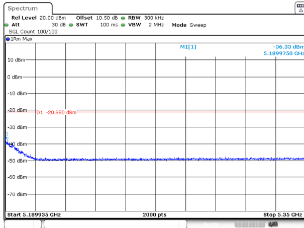
802.11ax20_5180MHz_RU_FULL_Ant 1
