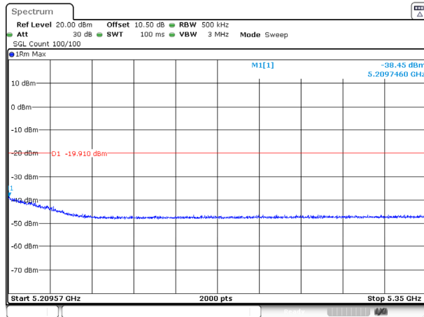
802.11ac40_5190MHz_Ant 0
