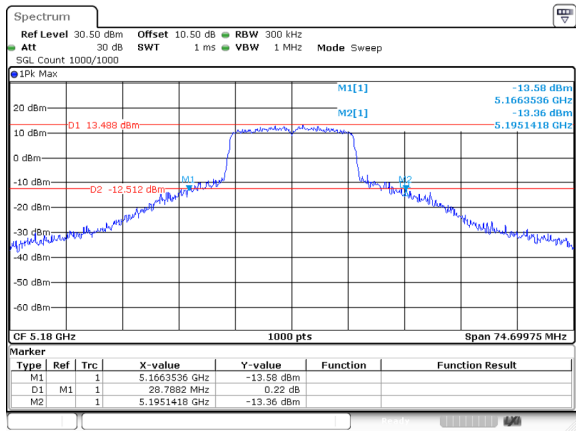
802.11a_5180MHz_Ant 0
