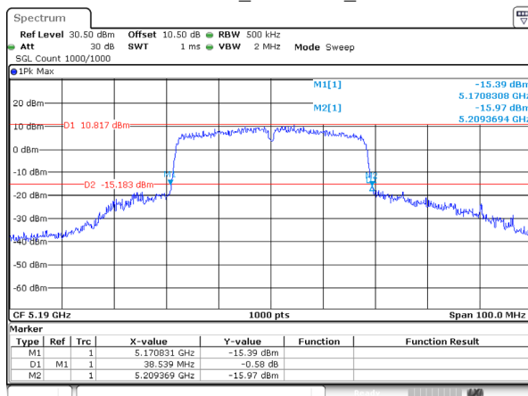
802.11ac40_5190MHz_Ant 2
