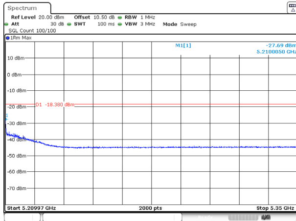
802.11ax40_5190MHz_RU_FULL_Ant 0
