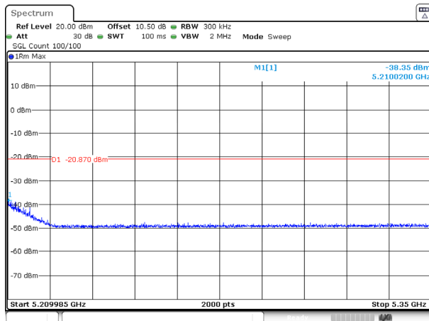
802.11ax20_5200MHz_RU_FULL_Ant 2
