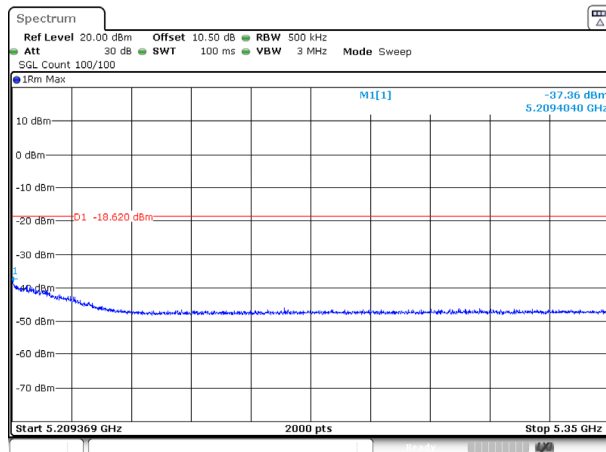
802.11ac40_5190MHz_Ant 2
