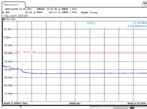
802.11ax40_5190MHz_RU_FULL_Ant 2
