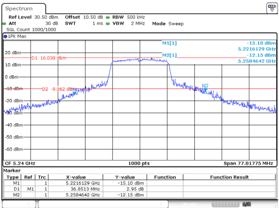
802.11a_5240MHz_Ant 1
