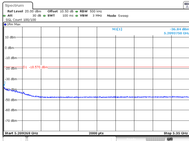
802.11ac40_5190MHz_Ant 1
