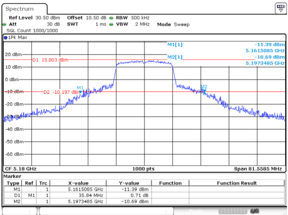
802.11a_5180MHz_Ant 1
