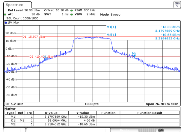
802.11a_5200MHz_Ant 2
