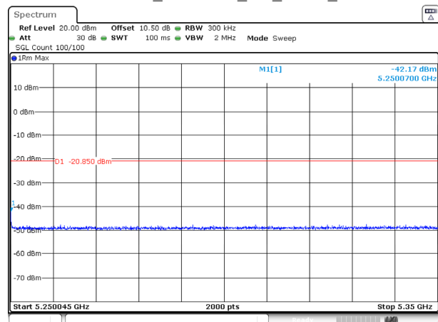
802.11ax20_5240MHz_RU_FULL_Ant 0
