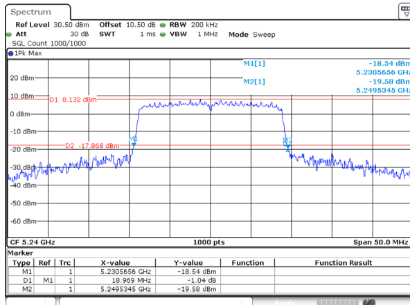
802.11ac20_5240MHz_Ant 1
