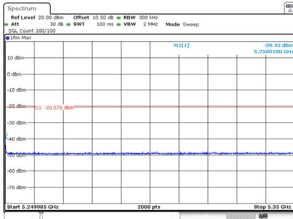
802.11ax20_5240MHz_RU_FULL_Ant 1
