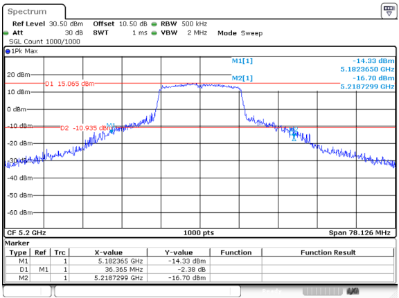
802.11a_5200MHz_Ant 0
