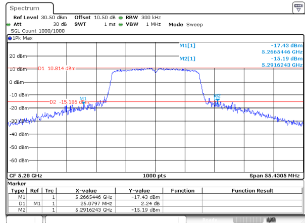
802.11a_5280MHz_Ant 1
