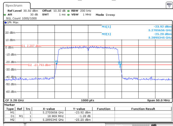
802.11ac20_5280MHz_Ant 2
