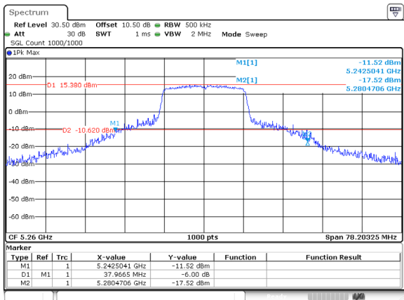
802.11a_5260MHz_Ant 0
