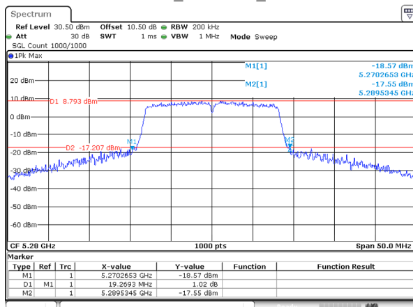
802.11a_5280MHz_Ant 2
