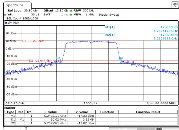
802.11a_5260MHz_Ant 2
