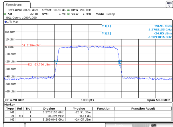
802.11ac20_5280MHz_Ant 0
