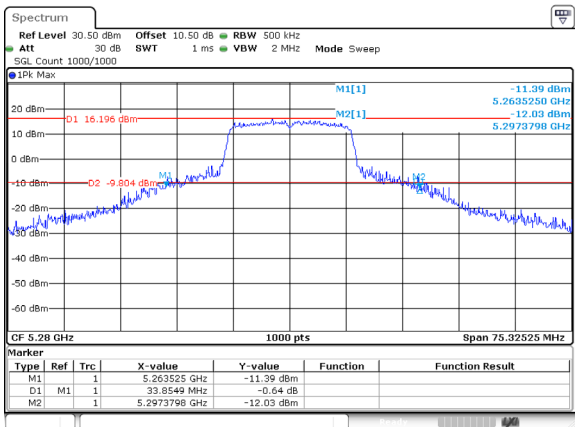
802.11a_5280MHz_Ant 0
