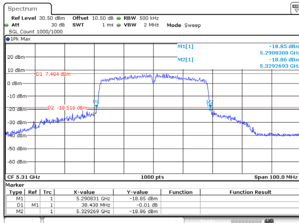
802.11ac40_5310MHz_Ant 2
