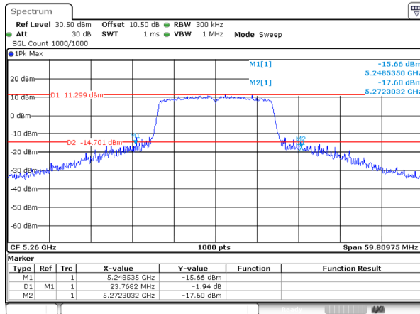
802.11a_5260MHz_Ant 1
