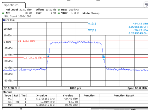
802.11ac20_5280MHz_Ant 1
