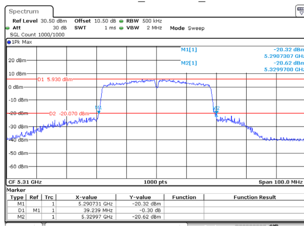
802.11ac40_5310MHz_Ant 0
