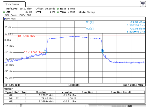
802.11ac80_5290MHz_Ant 0
