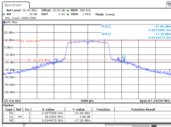
802.11a_5600MHz_Ant 1
