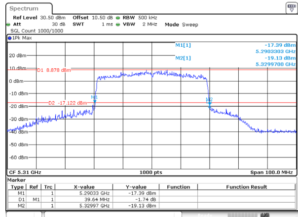
802.11ax40_5310MHz_RU_FULL_Ant 1
