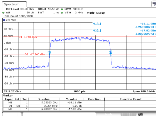
802.11ax40_5270MHz_RU_FULL_Ant 0
