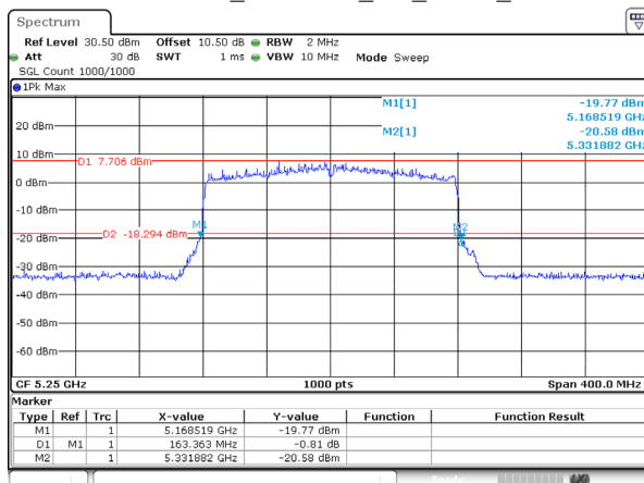
802.11ax160_5250MHz_RU_FULL_Ant 1
