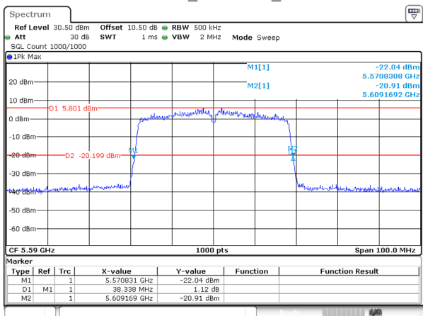
802.11ac40_5590MHz_Ant 1
