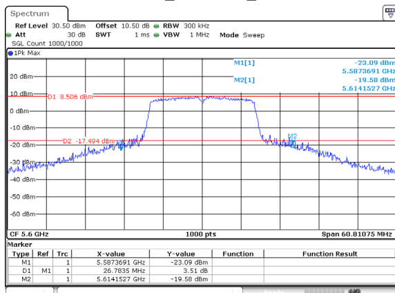
802.11a_5600MHz_Ant 0
