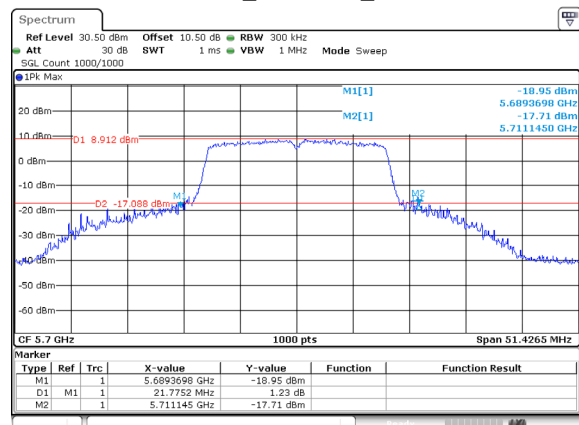
802.11a_5700MHz_Ant 0
