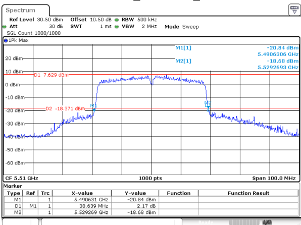
802.11ac40_5510MHz_Ant 2
