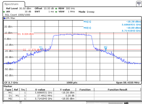
802.11a_5700MHz_Ant 1
