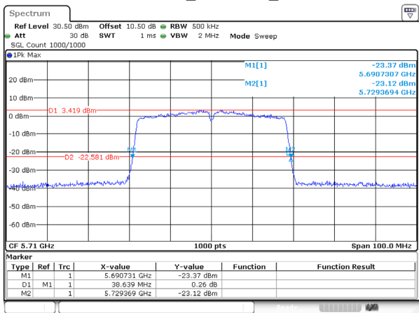
802.11ac40_5710MHz_Ant 0
