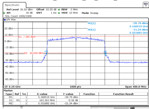
802.11ax160_5250MHz_RU_FULL_Ant 2
