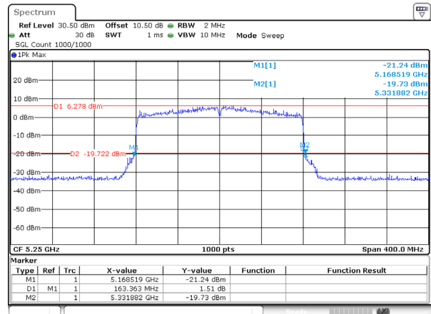
802.11ax160_5250MHz_RU_FULL_Ant 0
