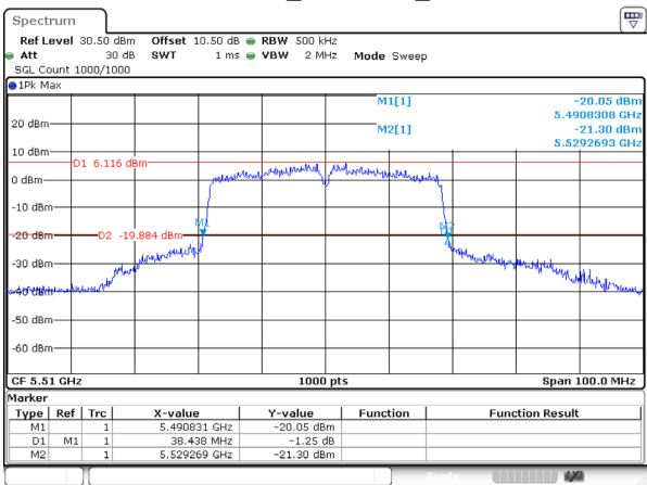
802.11ac40_5510MHz_Ant 1
