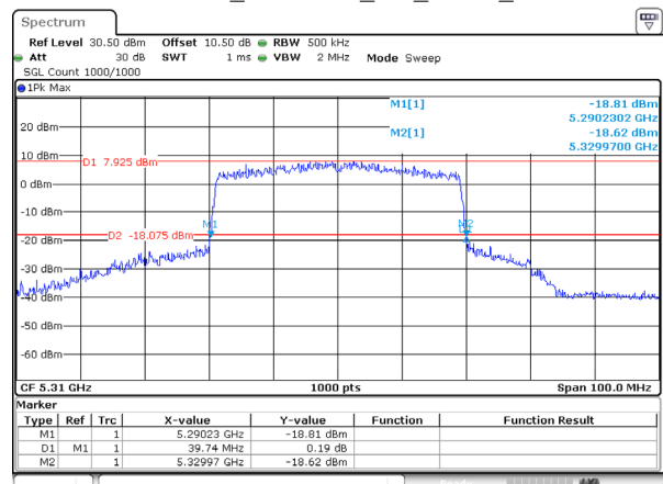
802.11ax40_5310MHz_RU_FULL_Ant 2
