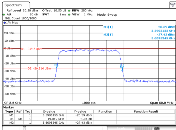
802.11ac20_5600MHz_Ant 0
