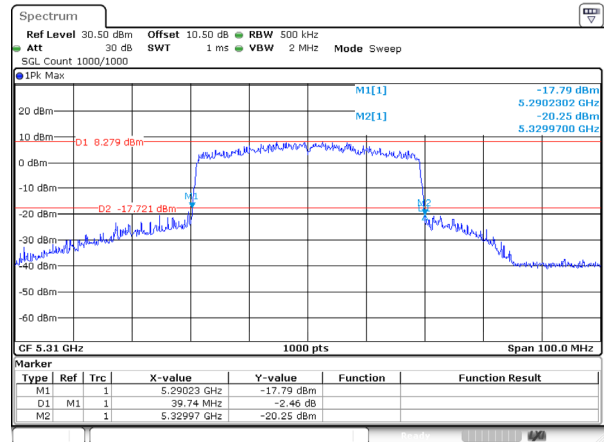
802.11ax40_5310MHz_RU_FULL_Ant 0
