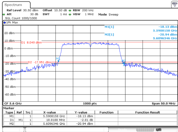
802.11a_5600MHz_Ant 2
