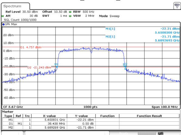
802.11ac40_5670MHz_Ant 1
